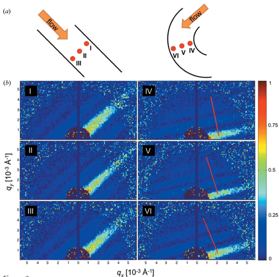
Figure 3 (a) Sketch of the selected observation positions at 30%, 50% and 70% relative width of the channel in straight and curved channels, respectively. (b) Correlation images of normalized g_2 ( \tau = 20 \text{ ms} ) at positions I–III in a straight channel and position IV–VI in a curved channel with radius R = 500 \mu\text{m} . The average flow velocity was 10 \mu\text{m s}^{-1} . The red lines in frames IV–VI are oriented parallel to the flow direction.
