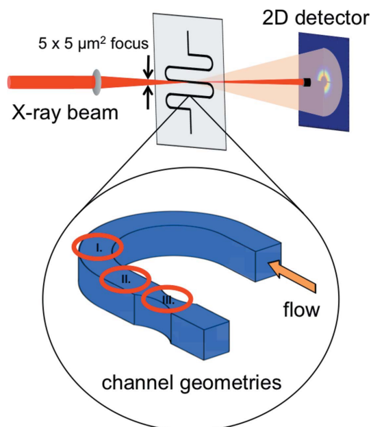
Figure 1 Experimental setup highlighting the three analyzed different microchannel geometries: curved channel (I), straight channel (II) and constriction (III).
