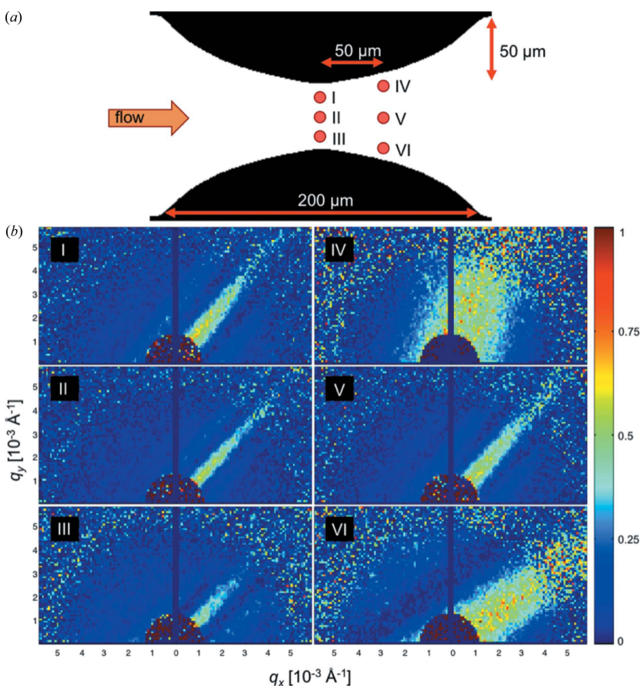
Figure 5 (a) Sketch of the microchannel constriction with six selected measurement positions. I–III are in the narrow part and IV–VI are in the wider part 50 \mu\text{m} downstream of the center of the constriction. (b) Two-dimensional correlation patterns of normalized g_2 ( \tau = 10 ms) at positions I–III in the central most narrow part of the constriction and at positions IV–VI 50 \mu\text{m} downstream of the center of the constriction. The average flow velocity in the straight channel before the constriction was 6 \mu\text{m s}^{-1} .
