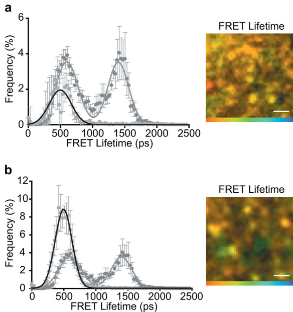
FIGURE 3. Two t -SNARE conformations are a result of differential SNAP-25 engagement. a , truncation of the C terminus of SNAP-25 to mimic BoNT/E cleavage (SNAP-25-(1–181)) abolished the state 2 conformation as shown in the histogram of FRET lifetimes (left panel) resulting in a largely uniform spatial distribution of FRET lifetimes (right panel) with a lifetime corresponding to the state 1 conformation. b , truncation of the entire C-terminal helix of SNAP-25 (SNAP-25-(1–120)) also abolished the state 2 conformation (left panel) resulting in a more uniform spatial distribution of FRET lifetimes (right panel). All color scales: 0–2000 ps. All scale bars 1 \mu m unless otherwise stated. Graphs show means \pm S.E., n = at least five independent experiments.
