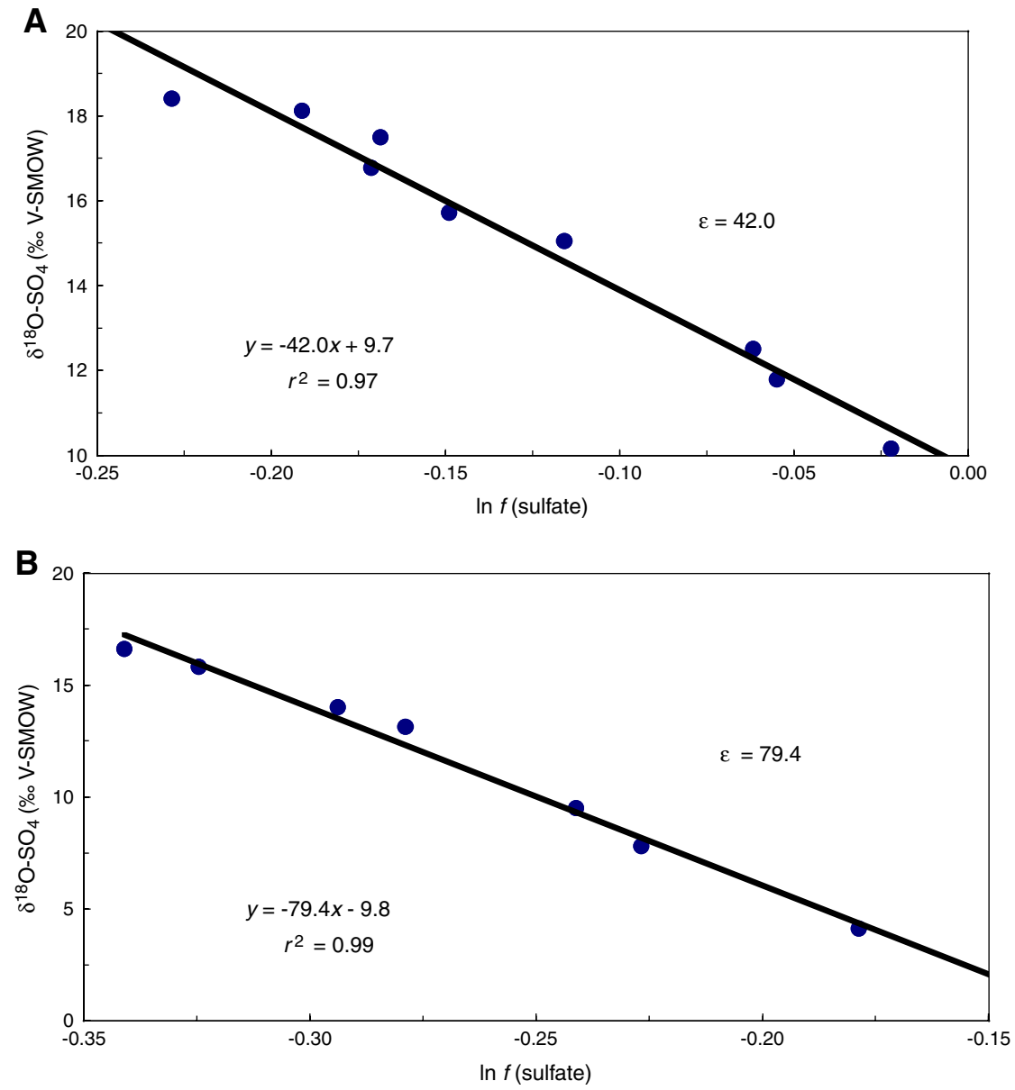
Figure F7. Site 1226 oxygen isotope enrichment factors for (A) upper and (B) lower MSR zones. V-SMOW = Vienna-standard mean ocean water.
