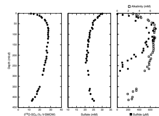
F5. Pore water profiles, Site 1226, p. 18.
