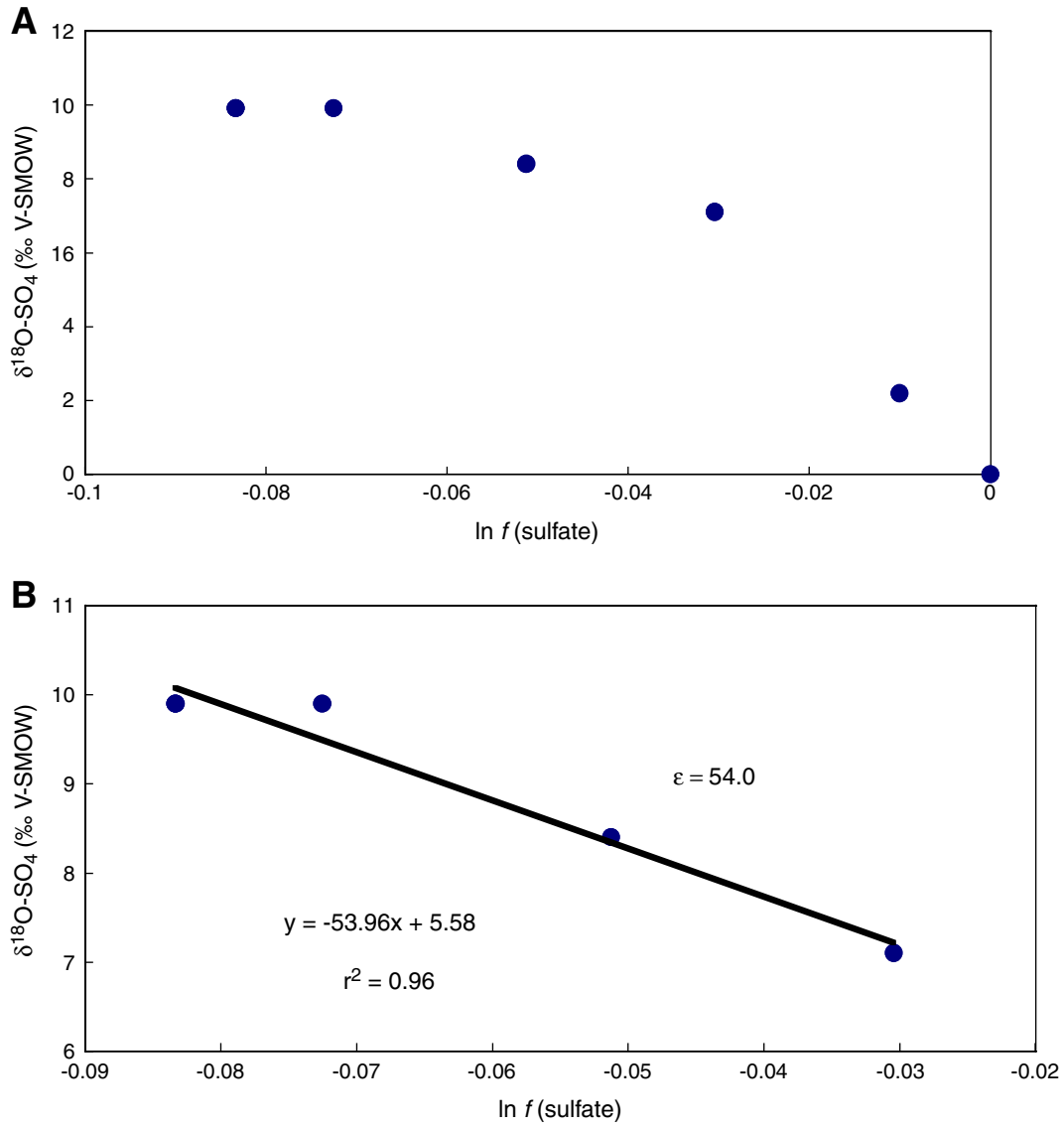
Figure F4. Isotopic fractionation during MSR at Site 1225. A. \delta^{18}\text{O}\text{-SO}_4 vs. fraction of \text{SO}_4 remaining ( \ln f ) in the upper MSR zone (0–200 mbsf) showing nonlinear behavior. B. Sulfate oxygen isotope enrichment factor, \epsilon\text{-SO}_4 , for linear region of A. V-SMOW = Vienna-standard mean ocean water.
