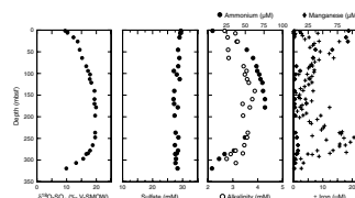
F3. Pore water profiles, Site 1225, p. 16.
