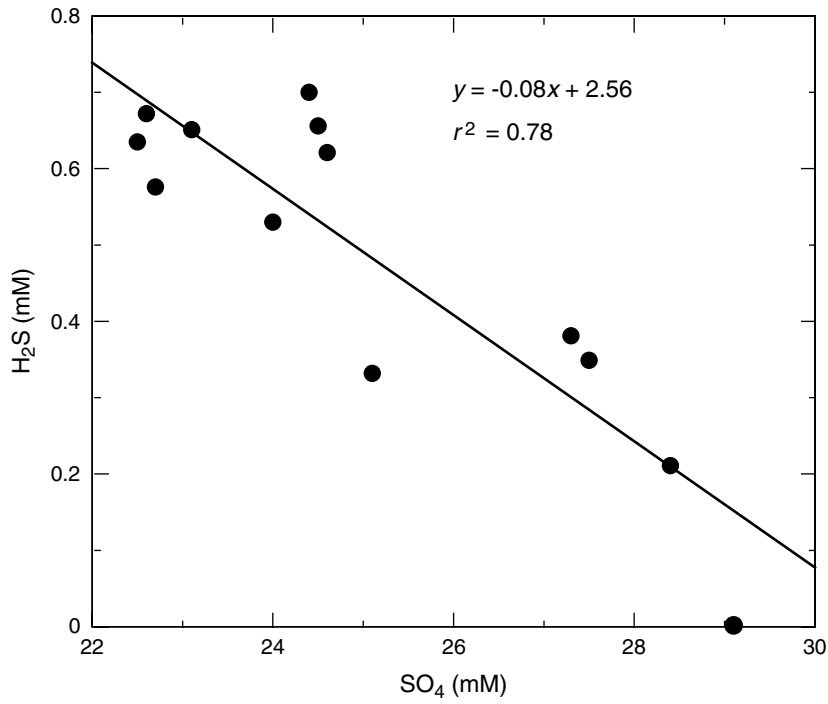
Figure F6. Site 1226 sulfate vs. sulfide. Negative linear correlation suggests sulfide formation at the expense of sulfate. Data plot far below 1:1 slope for MSR-dominated systems. Data are from D'Hondt, Jørgensen, Miller, et al. (2003).
