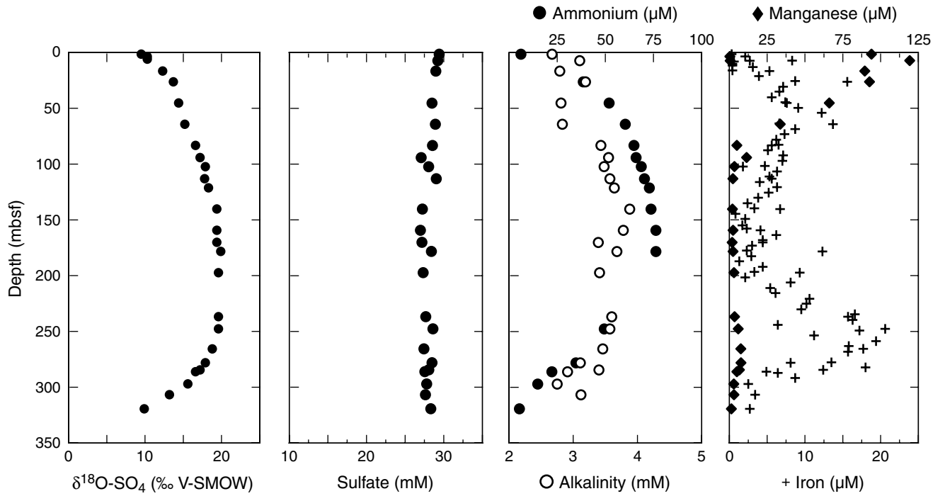
Figure F3. Site 1225 pore water profiles of \delta^{18}\text{O}\text{-SO}_4 , dissolved sulfate, ammonium and alkalinity, and dissolved manganese and iron vs. depth. \delta^{18}\text{O}\text{-SO}_4 data are from this study. All other data are from D'Hondt, Jørgensen, Miller, et al. (2003). V-SMOW = Vienna-standard mean ocean water.
