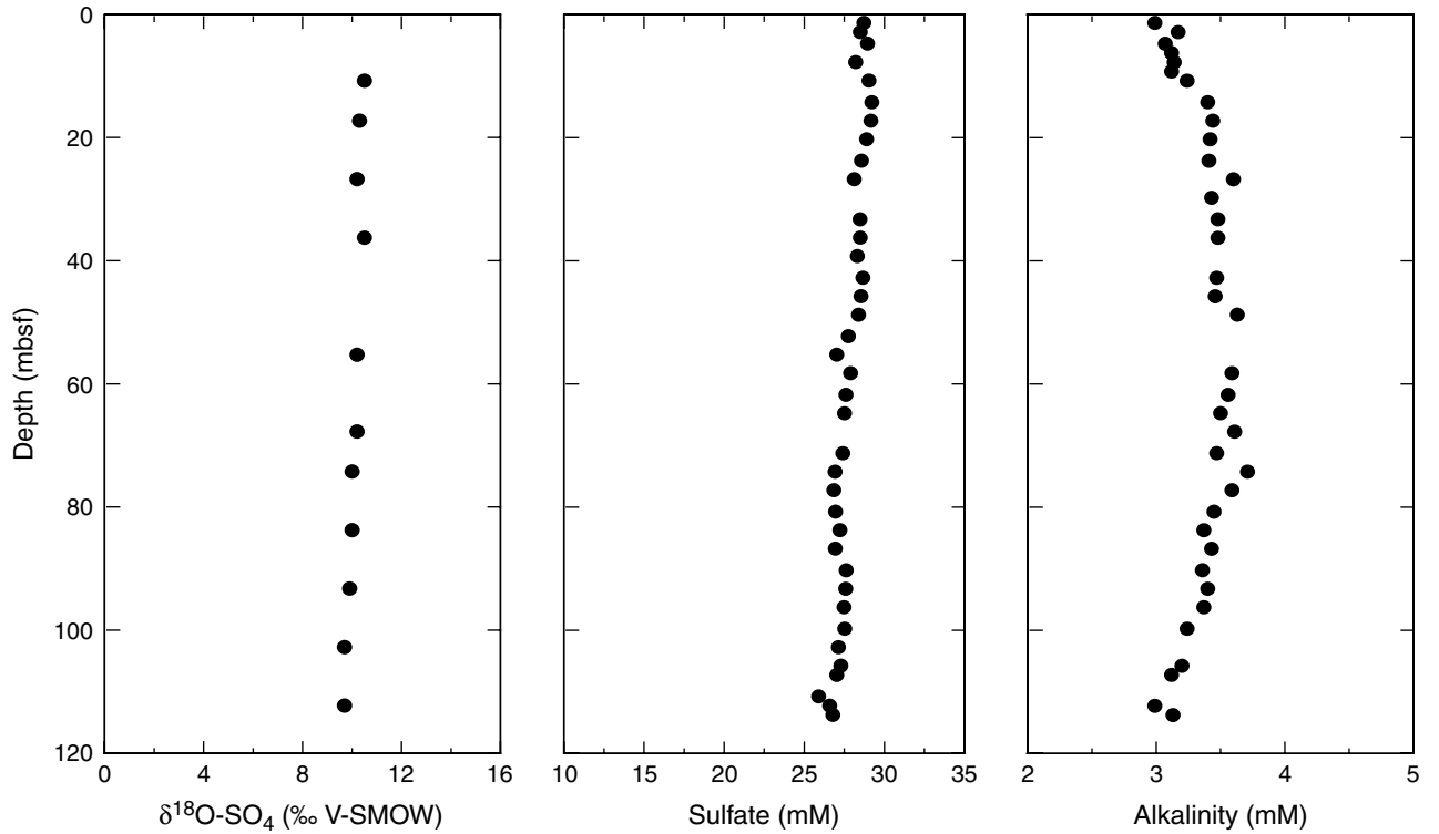
Figure F2. Site 1231 pore water profiles of \delta^{18}\text{O}\text{-SO}_4 , dissolved sulfate, and alkalinity vs. depth. \delta^{18}\text{O}\text{-SO}_4 data are from this study. All other data are from D'Hondt, Jørgensen, Miller, et al. (2003). V-SMOW = Vienna-standard mean ocean water.
