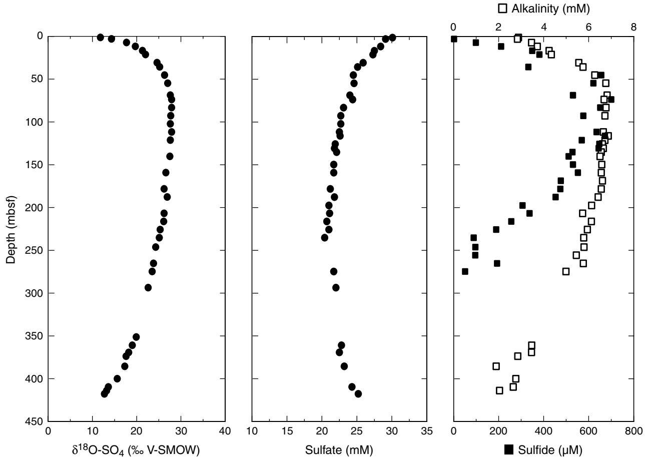
Figure F5. Site 1226 pore water profiles of \delta^{18}\text{O}\text{-SO}_4 , dissolved sulfate, and dissolved sulfide ( \Sigma\text{H}_2\text{S} = \text{HS}^-_{(\text{aq})} + \text{H}_2\text{S} ) and alkalinity vs. depth. \delta^{18}\text{O}\text{-SO}_4 data are from this study. All other data are from D'Hondt, Jørgensen, Miller, et al. (2003). V-SMOW = Vienna-standard mean ocean water.
