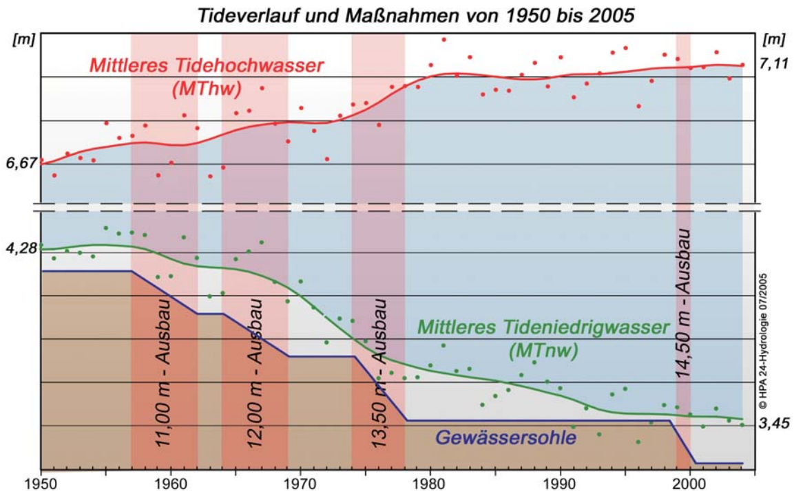
Fig. 1: Mean depth of the waterway, mean low water (MLW, green line) and mean high water (MHW, red line) at Hamburg St. Pauli 1950–2004. The depth of the waterway is given in chart datum (SKN) while MLW and MHW are indicated in m above the tide gage (Pegelnul) of 5 m. The MLW is not stable during the interval of interest (1980–1990) but the MHW is stable. The horizontal lines delineate 20 cm differences. Courtesy of Hamburg Port Authority, Hydrology
