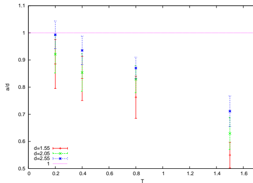
Figure 15: Plot of a/d versus T at d = 1.55, 2.05 and 2.55 in 4 SUSY matrix quantum mechanics.
