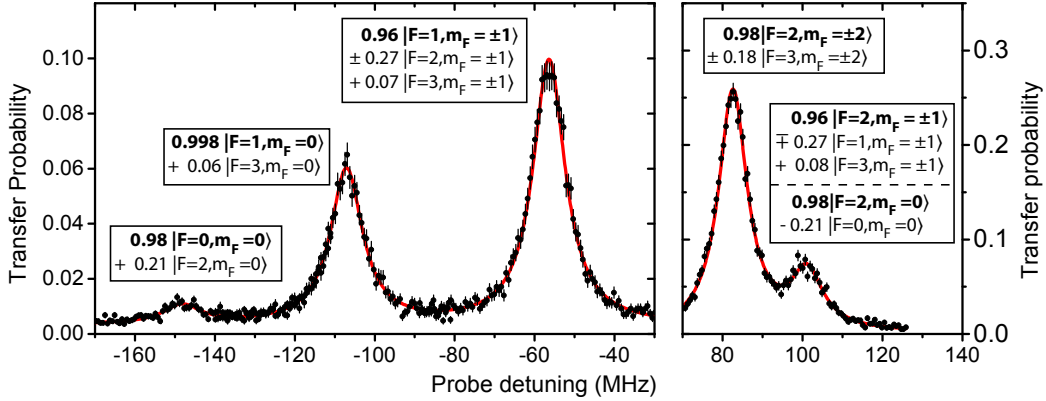
Figure 3.5.: Spectroscopy of excited states perturbed by the trap light Single spectrum recorded at P_{1064} = 2.25 W. Five resonances are clearly visible. The peaks are labeled with the energy eigenstates expressed in the hyperfine basis (see text). Splitting of the F=2 state (double peak in the very right part of the spectrum), which is not predicted in the weak-field approximation, is an unambiguous indication of hyperfine-breakdown. The leftmost peak indicates a state which for weak power coincides with the unperturbed F=0 state. The F=0 state does not decay to the F=2 ground state. The fact that population transfer is observable here stems from the admixture of the F = 2, m_F = 0 excited state to the energy eigenstate.
