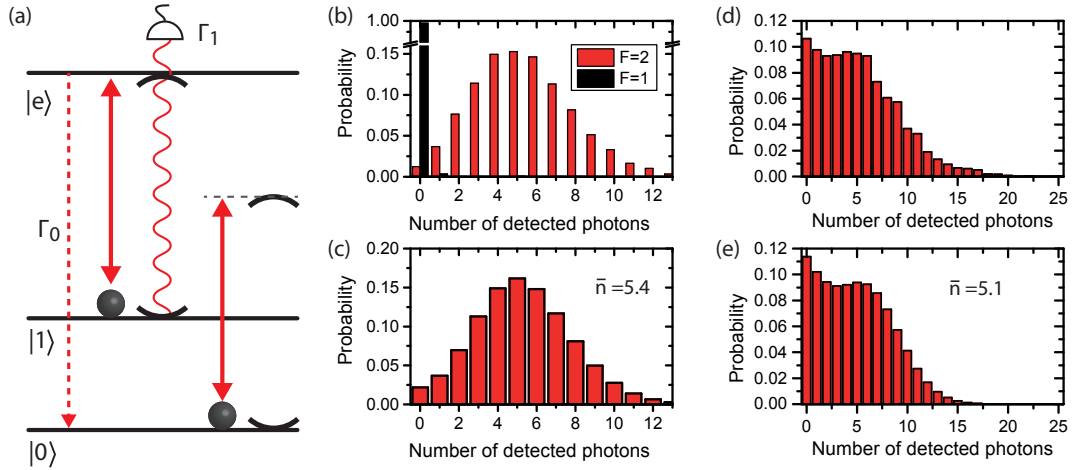
Figure 2.7.: Hyperfine state detection (a) Sketch of the scheme for cavity-assisted hyperfine-state detection. (b) Measured photon number distribution for a probing time of T = 15 \mu\text{s} in the case of |1\rangle = |5S_{1/2}, F = 2\rangle and |e\rangle = |5P_{3/2}, F = 3\rangle . The red (black) bars show data that was measured after initializing the atom in the F=2 ( F=1 ) ground state. (c) Theory values calculated with \Gamma_1=370 kHz and \Gamma_0=1 kHz. The atom in this case is lost to a dark state only after an average of 370 signal photons has been detected. (d) Result of an attempt to perform state detection with |1\rangle = |5S_{1/2}, F=1\rangle and |e\rangle = |5P_{3/2}, F=0\rangle . (e) Theory values calculated for \Gamma_1=100 kHz and \Gamma_0=13 kHz.
