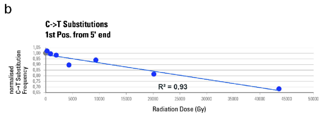
Figure 4. X-ray-induced effects on aDNA nucleotide misincorporation patterns for the first 25 positions from both ends of the molecule. (a) The misincorporation frequencies of the non-scanned controls are shown as a green line. Lower frequencies (red line) of C to T substitutions at the 5' ends and G to A substitutions at the 3' ends can be observed after irradiation at 43.5 kGy, since the fraction of aDNA fragments without terminal nucleotide misincorporations increases through exposure. (b) Normalised C to T substitution frequencies of the 1 st position from 5' end of endogenous DNA molecules are plotted against cumulative radiation dose received after 0 s (0 Gy), 2.2 s (~206 Gy), 10 s (~937 Gy), 21.5 s (~2.02 kGy), 46.4 s (~4.35 kGy), 100 s (~9.37 kGy), 215.4 s (~20.2 kGy) and 464.2 s (~43.5 kGy). The non-scanned control is represented as a grey circle, the scans as blue circles. Substitution frequencies were normalised by the corresponding non-scanned controls, and averaged per exposure time group consisting of two aliquots from independent DNA-libraries.
