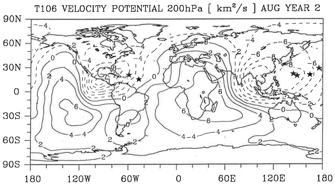
Figure 17 Velocity potential at 850 and 200 hPa and the number of generated hurricanes in August year 2 (small number of storms).
