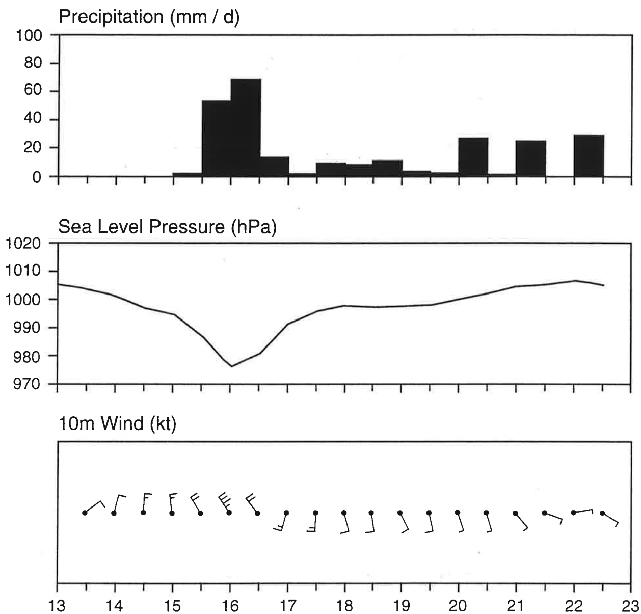
Figure 2 Meteogram for Fu-Chou (Fukien, China) showing precipitation, surface pressure and 10m wind for every 12 hrs from August 13 to August 22 Year 1 of the simulation.
