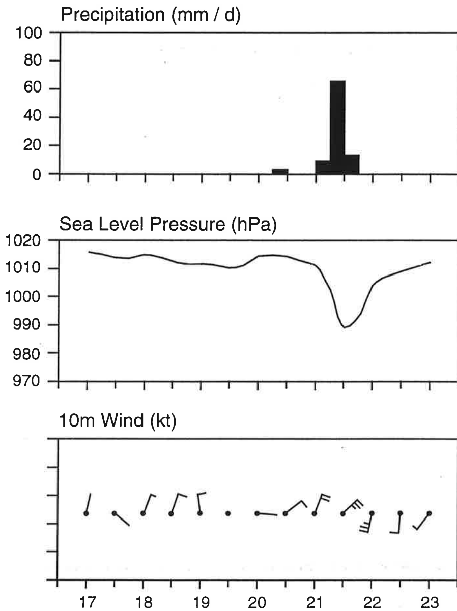
Figure 3: Meteogram for Charleston (South Carolina, USA) showing precipitation, surface pressure and 10m wind for every 6hrs from September 17 to September 23, 1989, hurricane Hugo, predicted by the ECMWF model from September 17, 1989 12 UTC.
