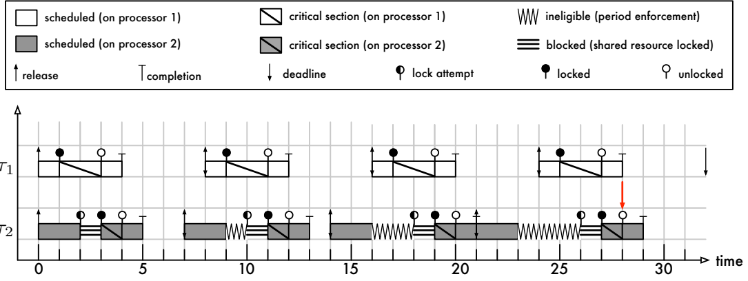
Figure 5: Example schedule of two tasks \tau_1 and \tau_2 on two processors sharing one lock-protected resource. The example assumes that lock requests take effect only when the critical section segment becomes eligible to be scheduled according to the rules of the period enforcer algorithm. Under this interpretation, the fourth job of task \tau_2 misses its deadline at time 28.
