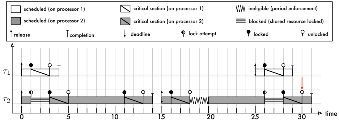
Figure 8: Example schedule of two tasks \tau_1 and \tau_2 on two processors sharing one lock-protected resource. The example assumes that lock requests take effect immediately and that critical sections are exempt from period enforcement (i.e., period enforcement is applied only to any computation after a critical section). As in Figure 7, the second job of task \tau_2 misses its deadline at time 30.
