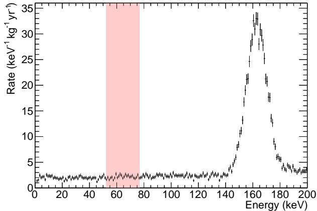
FIG. 1. Spectrum of remaining events after all cuts. The peak at 164 keV originates from ^{131m}\text{Xe} . The red shaded area indicates the \pm 3\sigma region around the expected 2\nu 2\text{K} peak of ^{124}\text{Xe} .
