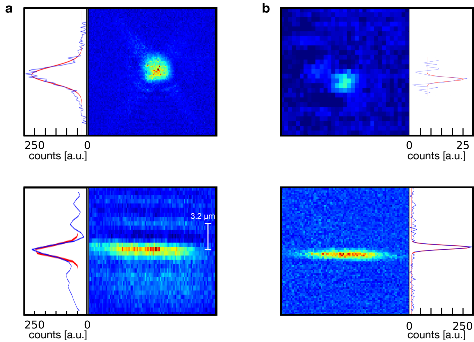
Figure 4.2: Effect of dimple spill out on plane loading process. Absorption images of different cloud realizations. (a) Fully loaded dimple trap (top left, P = 1 mW) containing about 10^4 atoms. After adiabatic release into the long scale z-Lattice (bottom, V_z = 178 E_R ) atoms populate not only the central but also the neighboring planes. (b) Spilling out the dimple trap (top right) by reducing its power to P = 0.1 mW, reduces the number of atoms and the size of the cloud, such that only a single plane of the vertical lattice gets populated (bottom right).
