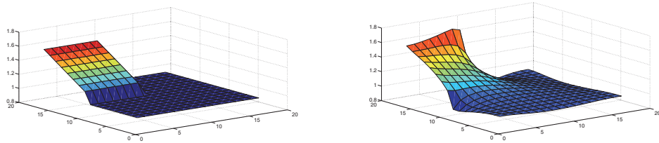
(a) Desired state at grid point 65 in time. (b) Computed state at grid point 65 in time for \beta = 10^{-6} .
