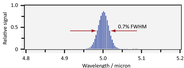
Figure 2: Spectrum of the FEL laser line centered at 5 μm measured with the grating spectrometer.
