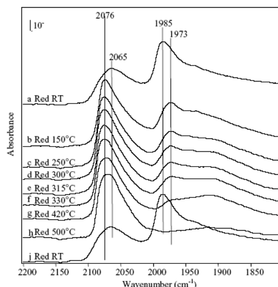
Fig. 7: IR spectra for Pd/ZnO/Al 2 O 3 catalysts undergoing an oxidation-reduction cycle. Note that between scans (h) and (j) the sample was oxidized at 500 °C for two hours, followed by reduction at room temperature for two hours in H 2 . The peaks associated with Pd-CO (linear: 2065 cm -1 , bridged: 1985 cm -1 ) and Pd-Zn (linear: 2076 cm -1 ) can be clearly identified in these spectra. The formation of the Pd-Zn occurs readily even at low temperatures. Oxidation recreates the Pd surface.
