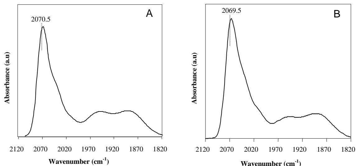
Fig. 8: IR spectra of adsorbed CO for catalyst samples A and B. Catalyst A was reduced at 450 °C for 2 hours before being tested for SRM at 250 °C, whereas catalyst B underwent no pretreatment. The two spectra are nearly identical and show the bands characteristic of linearly bound CO on Pd-Zn bimetallic, while the bands attributed to linearly bound CO on Pd are not detected. The relative ratio of the bridged to linear CO is another indication that the surface consists of the Pd-Zn alloy phase.
