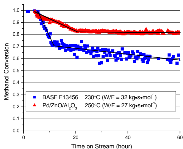
Fig.1: Activity over 60 h comparison between commercial Cu-based catalyst (BASF F13456) and Pd/ZnO/Al 2 O 3 . The Cu-based catalyst suffers from fast deactivation, whereas the Pd-based catalyst deactivates to a lesser extent. However, the activity of the Pd-based catalyst is initially lower and it is tested at 250 °C where the Cu-based catalyst is active at 230 °C.
