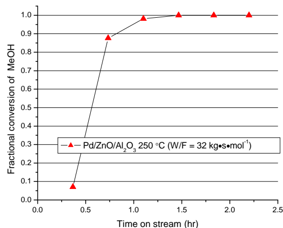
Fig.2: Regeneration of a deactivated Pd/ZnO/Al 2 O 3 catalyst after oxidation at 420 °C and exposure to steam reforming conditions at 250 °C. The catalyst is found to regain its initial activity within approximately 1 hour on stream.
