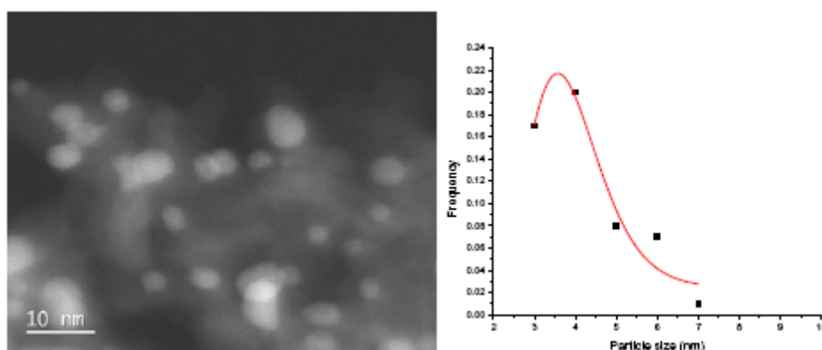
Fig. 5: HAADF STEM image of 8.8 wt % Pd/ZnO/Al 2 O 3 reduced at 420 °C for 2 hours. The particle size distribution of this catalyst is shown; the number average diameter is 3.7 nm.
