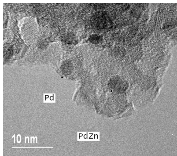
Fig. 7: HRTEM image of Pd/ZnO/Al 2 O 3 catalysts reduced at 250 °C. This image illustrates that both bulk PdZn and Pd nanoparticles can be identified within close proximity via cross-fringe analyses. It is also evident that the nanoparticles are not seen to be core-and-shell, although the EDX data shows a large variation between the near-edge and bulk compositions when reduced at this temperature.
