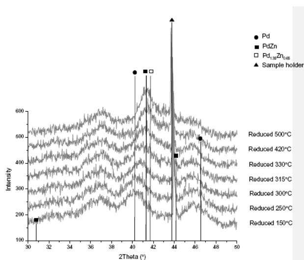
Fig.4: XRD patterns of Pd/ZnO/Al 2 O 3 catalysts reduced in-situ at various temperatures. The relative amounts of bulk Pd and Pd-Zn change as the catalyst is reduced at elevated temperature. Note that the sharp peak at 44 ° 2-theta is attributed to the metallic sample holder.
