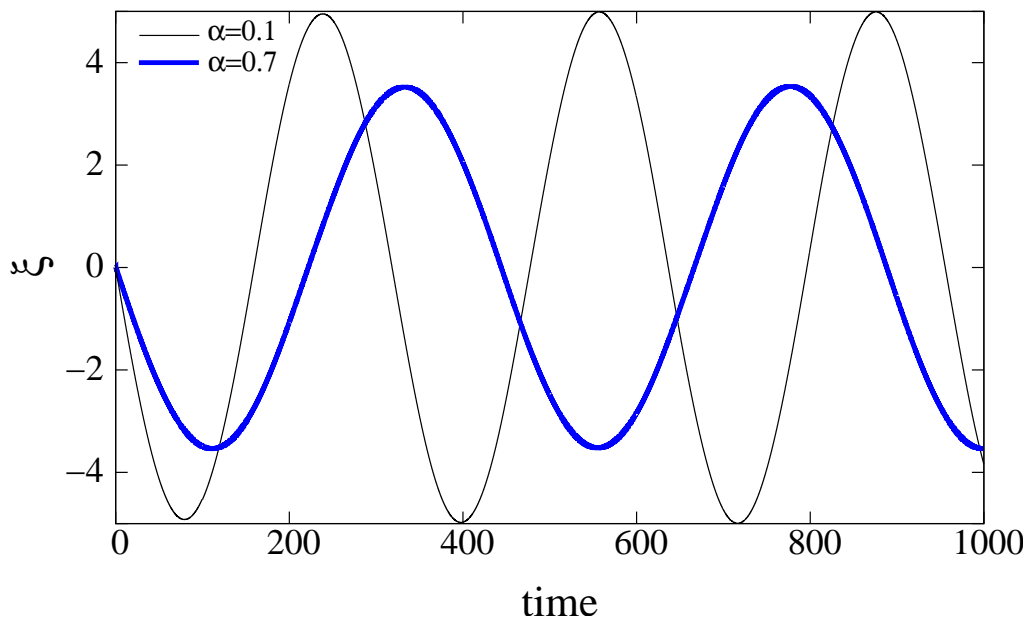
Figure 3: A plot of the dipole oscillations for \alpha = 0.1 and \alpha = 0.7 . The other parameters are \xi(0) = 0 , p(0) = 0.1 , \delta(0) = 0 , \gamma(0) = 40 , \Lambda = 5 , \Omega = 0.0002 . We notice that, as the strength of the secondary lattice increases, the dipole oscillations are blocked in accordance with the experimental observations of [31]. Since we are in the negligible mean field interaction regime, the dipole oscillations are not damped.
