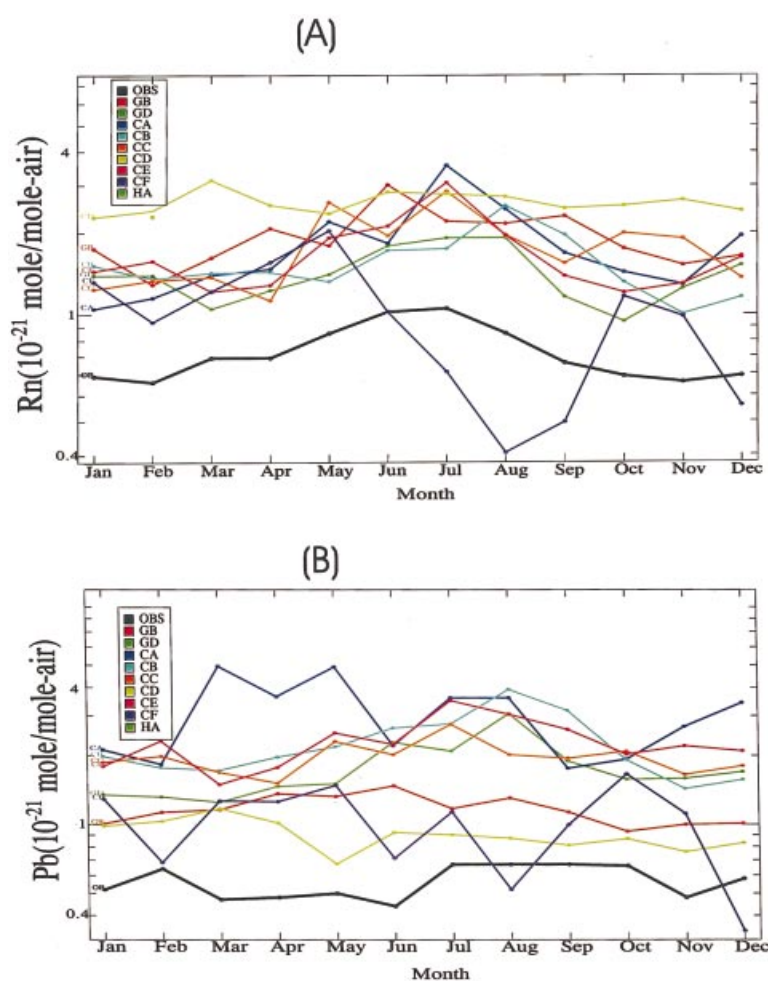
Fig. 16. Comparison of modeled and observed monthly mean mixing ratio of surface level ^{222}\text{Rn} and ^{210}\text{Pb} at Amsterdam Island (37.83°S, 72.53°E).
