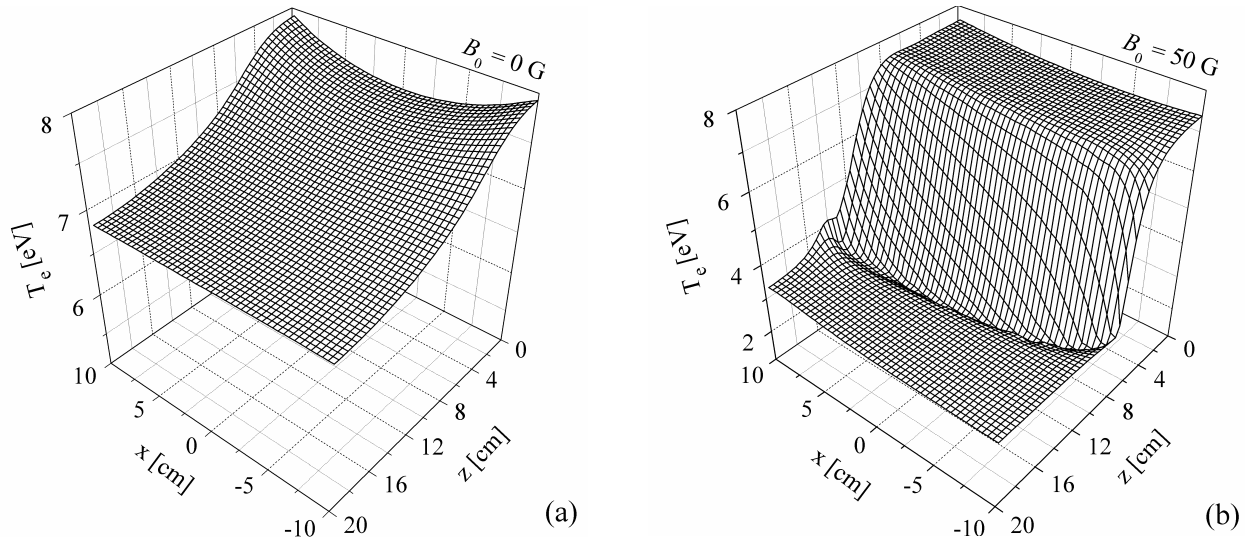
Figure 3. Spatial distribution of the electron temperature obtained within the 2D model for B_0 = 0 G (a) and B_0 = 50 G (b).
