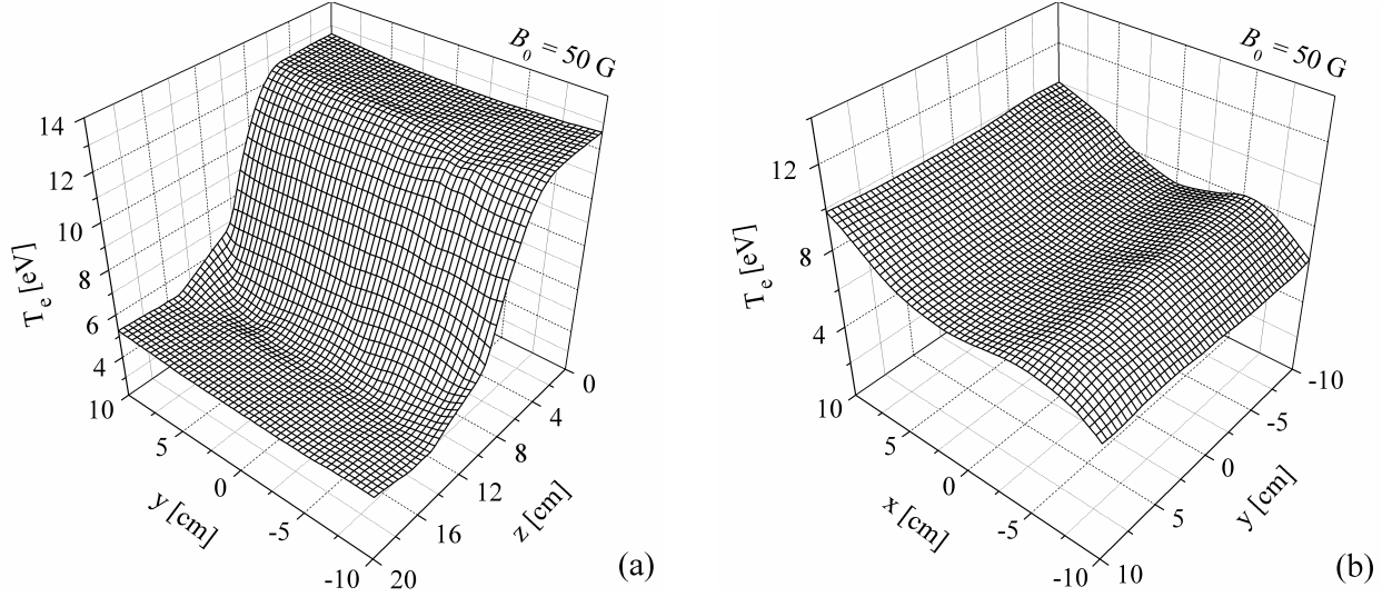
Figure 11. Results from the 3D-model: Spatial distribution of the electron temperature in the (y-z) -plane for x = 0 in (a) and in the (x-y) -plane for z \equiv z_0 = 10 cm in (b).
