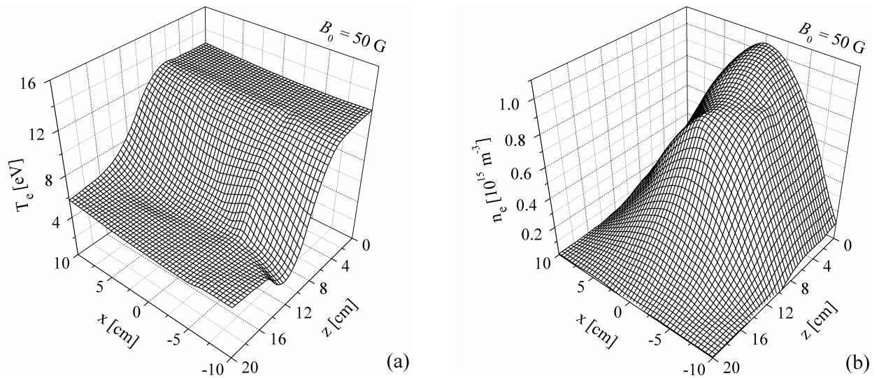
Figure 10. Results from the 3D-model: Spatial distribution of the electron temperature (a) and density (b) obtained in the ( x - z )-plane, for y = 0 .
