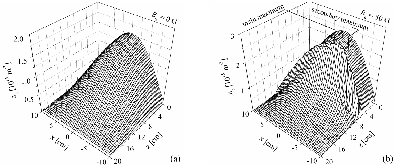
Figure 4. Spatial distribution of the electron concentration obtained within the 2D model for B_0 = 0 G (a) and B_0 = 50 G (b).
