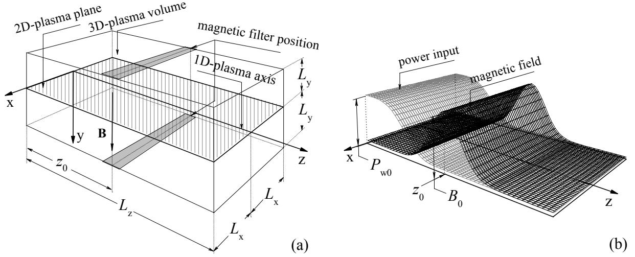
Figure 1. Configuration of the plasma volume in (a) and an illustration of the z -variations of the magnetic field and of the power input in (b).
