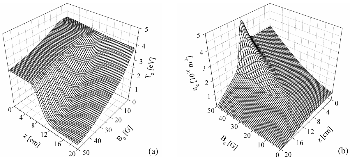
Figure 2. Results from the 1D-model: Axial distribution of the electron temperature (a) and density (b) for varying values of the magnetic field B_0 at the center of the filter.
