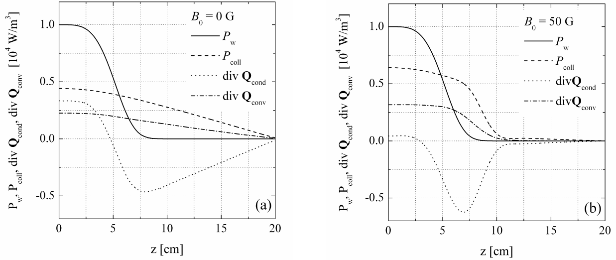
Figure 8. Axial changes, for x = 0 , of the different terms ( P_w , P_{\text{coll}} and the contributions of the conductive and convective fluxes to \text{div}\mathbf{Q}_e ) in the electron energy balance (5) for B_0 = 0 G (a) and B_0 = 50 G (b); results from the 2D-model.
