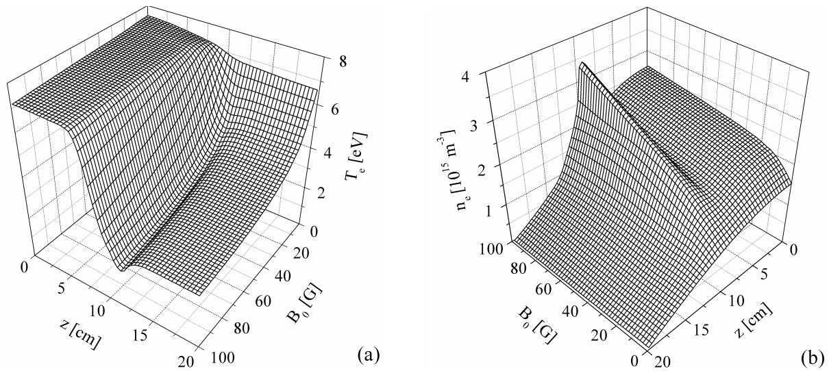
Figure 7. Changes of the axial distribution, for x=0 , of the electron temperature (a) and density (b) for varying values of the magnetic field B_0 obtained from the 2D model.
