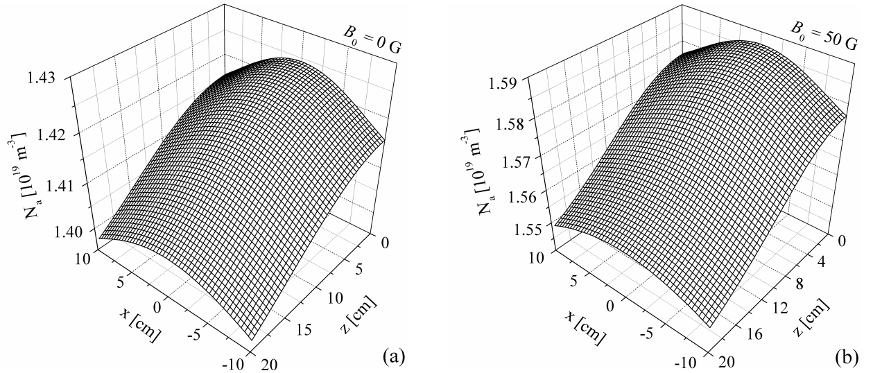
Figure 6. Spatial distribution of the atomic gas component obtained within the 2D model for B_0 = 0 G (a) and B_0 = 50 G (b).
