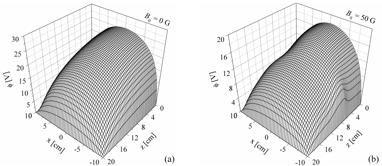
Figure 5. Spatial distribution of the potential of the dc electric field obtained within the 2D model for B_0 = 0 G (a) and B_0 = 50 G (b).
