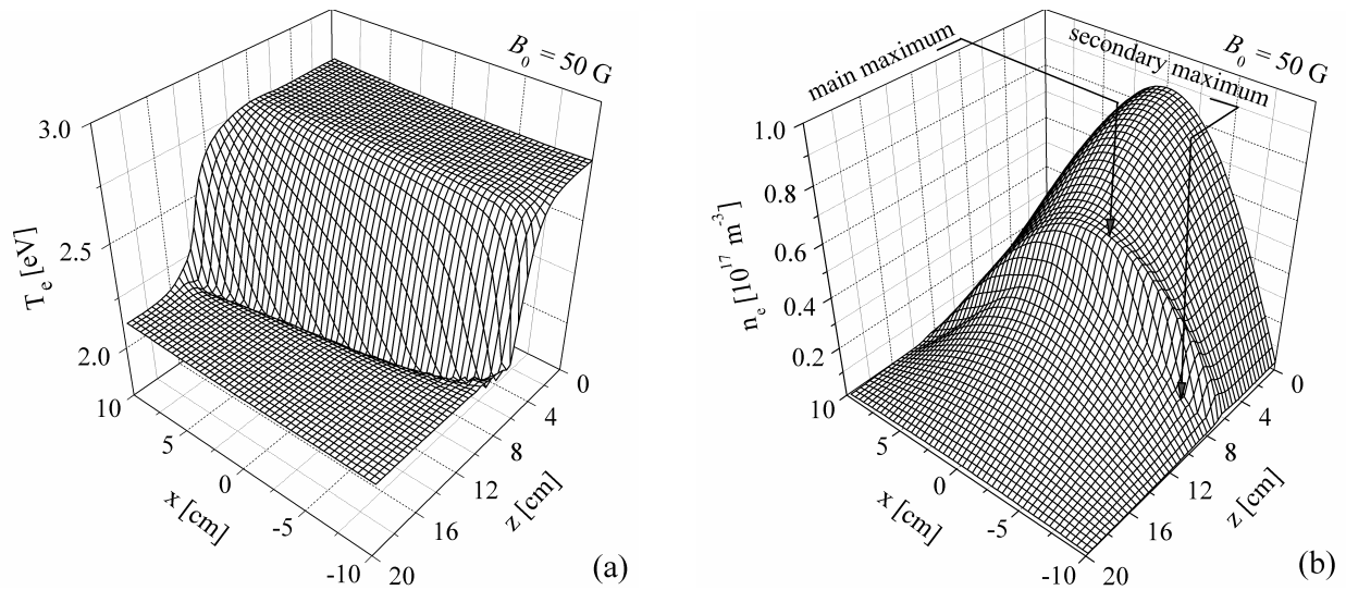
Figure 9. An argon discharge: spatial distribution of the electron temperature (a) and density (b) obtained within the 2D model.
