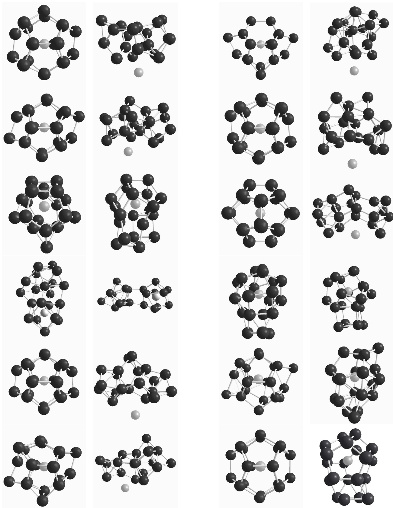
FIG. 1: The energetically lowest-lying configurations found for all M@Si_{20} systems as shown in the second and fourth columns have either lost their cage structure and dopant (bright) or undergone a transition to a smaller distorted cage with some peripheral silicon atoms. The corresponding most stable (distorted) cage-like structures are given in columns one and three. From top to bottom: M = Ba, Ca, Cr, Cu, K, and Na on the left, and M = Pb, Rb, Sr, Ti, V and Zr on the right half.
