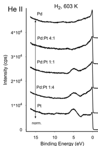
Figure 5: He II spectra for pure Pt, pure Pd and all PdPt samples after treatment D ( H_2 at 603 K)
