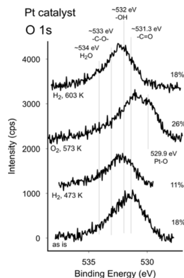
Figure 1: XPS spectrum of pure Pt, the O 1s spectrum measured after the four pretreatments.
