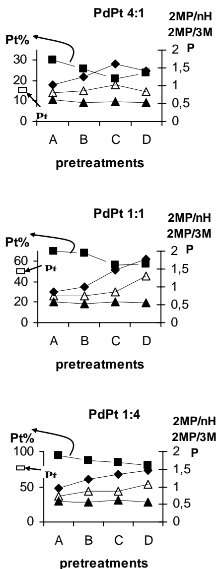
Figure 9: Selectivity and surface composition changes following different pretreatment conditions on bimetallic samples. ■ – Pt on the surface (XPS), ◆ – 2MP/nH from cis isomer, ▲ – 2MP/3MP from cis isomer, Δ – 2MP/3MP from trans isomer.
