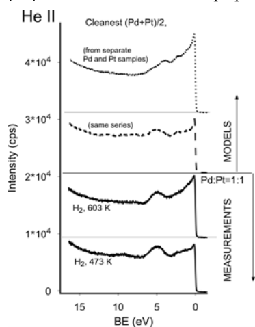
Figure 6: UPS spectrum of Pd:Pt = 1:1 in states B (473 K) and D (603 K) compared with models, which is average of the He II spectra of Pd and Pt from the same series in state B and from different Pd and Pt samples in state D .
