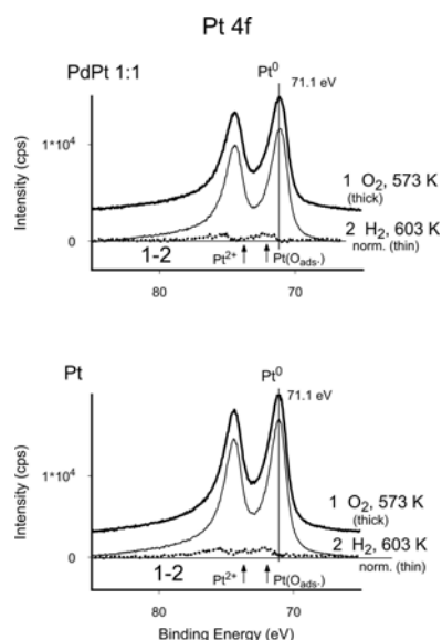
Figure 2: Changes in the Pt 4f line after treatments C (thick line) and D (thin line) (O 2 at 573 K and H 2 at 603 K).
