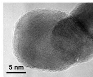
Figure 8: High resolution electron micrograph of a single PdPt 1:4 particle of about 15 nm diameter after various treatments and catalytic reactions.
