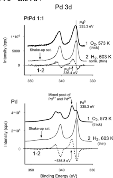
Figure 3: Changes in the Pd 3d line after treatments C (thick line) and D (thin line) (O 2 at 573 K and H 2 at 603 K)
