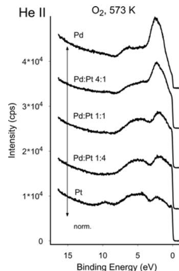
Figure 4: He II spectra for pure Pt, pure Pd and all PdPt samples after treatment C (O 2 at 573 K)
