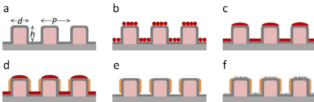
Figure 2. Concept. To fabricate functional Janus micropillar arrays, (a) the top faces of the micropillars were decorated with (b) one or more self-assembled monolayers of polymeric particle in a Langmuir trough. This covers and protects the top face after the particles were merged into a film by exposure to saturated toluene vapour (c), and the walls of the micropillars
