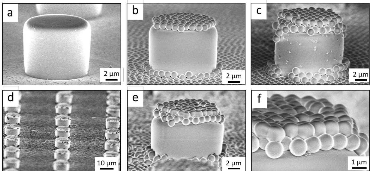
Figure 7. SEM images of silica-coated SU-8 micropillars. (a) silica-coated SU8 micropillar, (b) particle micropillars, c-f) particle micropillars that are decorated with an additional layer of PS particles before (c) and after (d-f) exposure to toluene vapour (dimensions: d = 11 \mu\text{m} , P = 40 \mu\text{m} , and h = 9 \mu\text{m} ).
