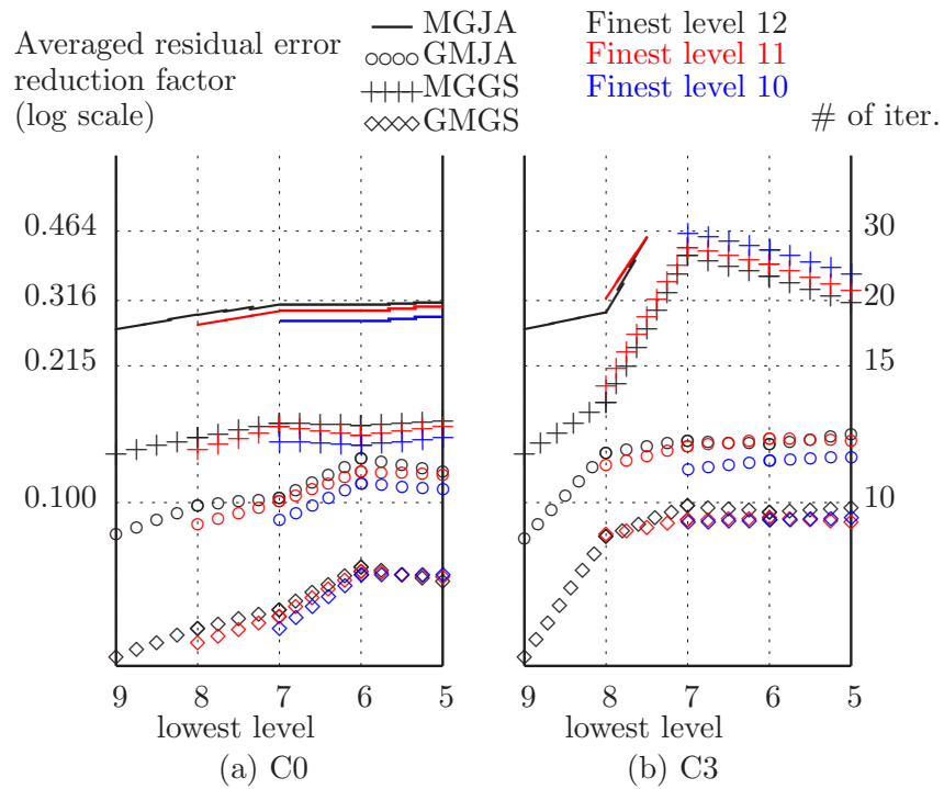
Figure 22: The averaged residual error reduction factor of four different solvers for the full square domain with the inner conducting areas C0 and C3.
