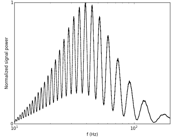
FIG. 2: Several precession cycles contribute comparably to the signal: Power ( |\hat{h}_\times|^2/S_h(f) ) versus frequency for a spinning binary viewed edge on in the \times polarization, computed directly from a Fourier transform of the gravitational-wave signal. In this figure, the binary is a 10 + 1.4M_\odot BH-NS binary with \chi_1 = 1 and \beta^* \approx \pi/3 (solid). Each pair of peaks corresponds to a single precession cycle. The signal is divided by the high-power zero-detune advanced LIGO noise PSD (power spectral density) [41].
