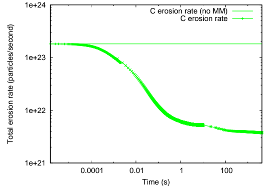
Fig. 3. Integral net C erosion rate, for the model without mixed materials and with mixed materials. The curve for the mixed materials combines runs with different time-steps for the plate. The integral net deposition is within 1% of the integral net erosion.
