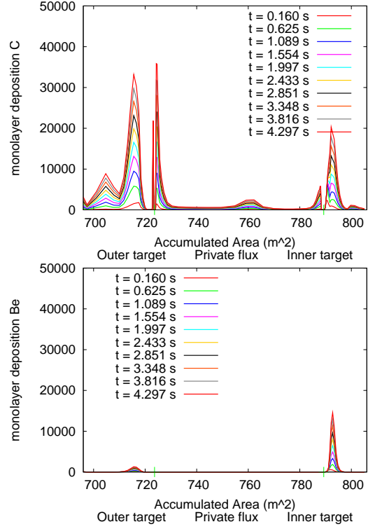
Fig. 5. Monolayers of deposition of C (top) and Be (bottom) for targets (bottom) for the ITER simulation. The x-coordinate starts at the main chamber wall just above the outer target and moves around the divertor region to the top of the inner target. The outer and inner target strike points are at 723.6 and 789.3, respectively.
