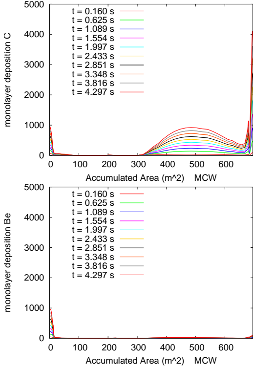
Fig. 4. Monolayers of deposition of C (top) and Be (bottom) for the main chamber wall for the ITER simulation. The x-coordinate starts at the main chamber wall (MCW) just above the inner target and moves around the main chamber to the outer target.
