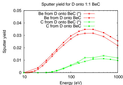
Fig. 6. Physical sputtering yields of Be and C produced by D bombardment of a 1:1 mixture of Be and C. The lines labeled with (*) indicates that the single species TRIM data[6] were used, and scaled by the relative fraction of the Be or C in the mixture ( \frac{1}{2} in this case).
