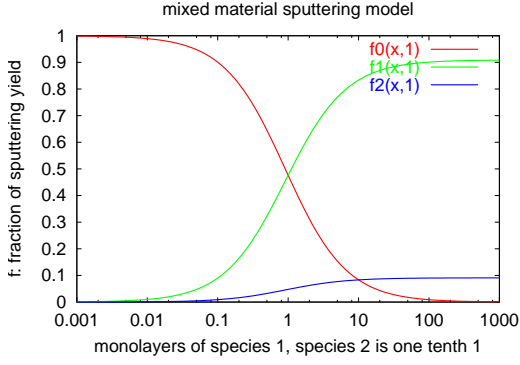
Fig. 1. The model for the fractional sputtering yield from mixed materials. f_0 is the sputter fraction of the base material, and f_1 and f_2 are the sputter fraction of deposited species “1” and “2”, where “2” is assumed to constitute one tenth the mono-layers of “1”.
