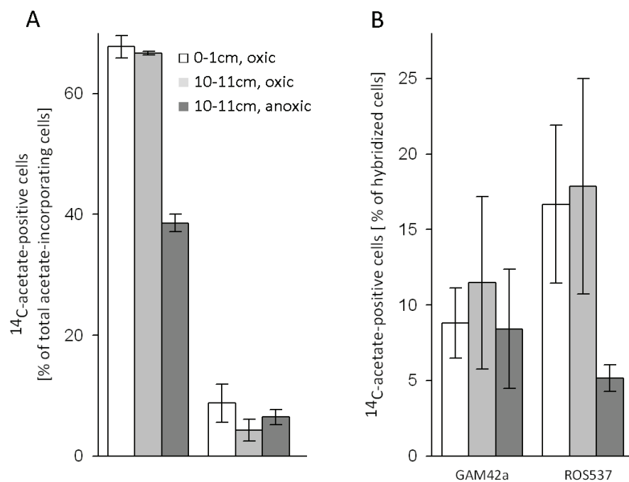
Figure 4 Relative abundances of ^{14}\text{C} -acetate incorporating members of Gammaproteobacteria and RCB in slurries of October 2008.
