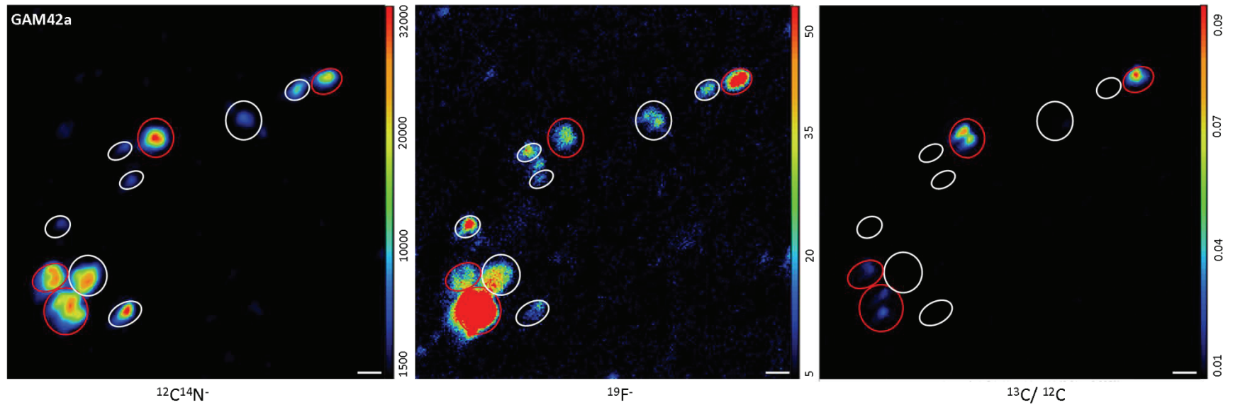
Figure 17 ^{13}\text{C} -acetate incorporation by individual cells of Gammaproteobacteria (GAM42a) revealed by nanoSIMS after fluorescence activated cell sorting. Circles indicate single cells of Gammaproteobacteria identified by the natural abundances of ^{12}\text{C} -carbon and ^{14}\text{N} -nitrogen ( ^{12}\text{C}^{14}\text{N} -) and the abundance of fluorine ( ^{19}\text{F} -) after HISH with a HRP-conjugated oligonucleotide probe and CARD with a fluorine containing tyramide. The ^{13}\text{C}/^{12}\text{C} ratios reveal cells that were enriched in ^{13}\text{C} -acetate (red circles). The scale bar corresponds to 1 \mu\text{m} .
