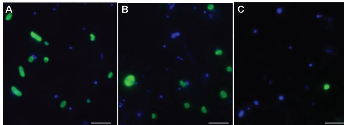
Figure 4 Epifluorescence microscope images of Epsilonproteobacteria . (A) Epsilonproteobacteria and (B) Arcobacter spp. were detected in the sulfidic intertidal pool. (C) In the sediment, Arcobacter spp. accounted for less than 0.5% of all cells. The scalebar corresponds to 5 \mu m.
