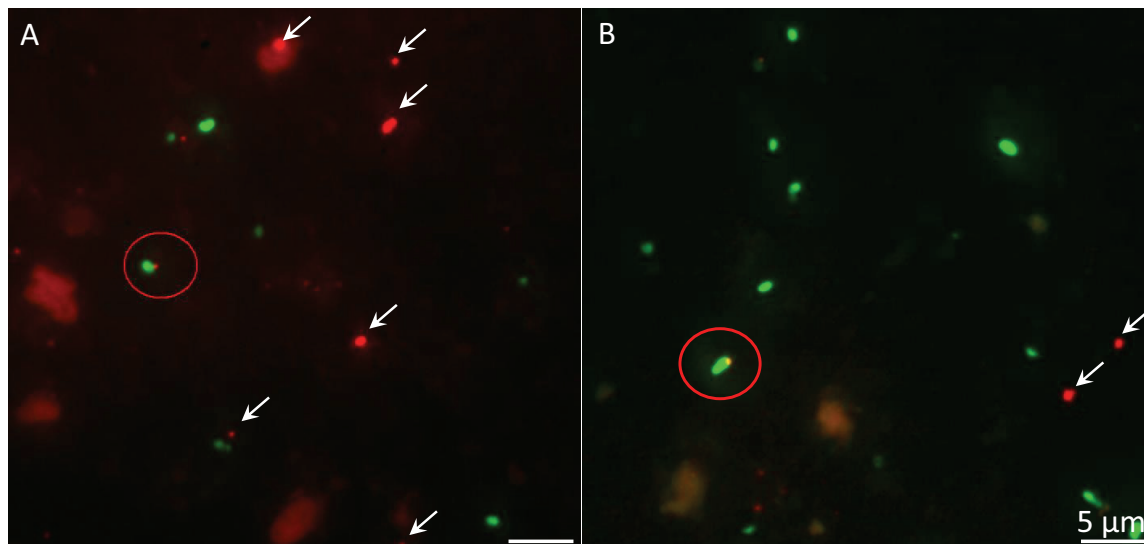
Figure 5 GeneFISH on Janssand sediment.
