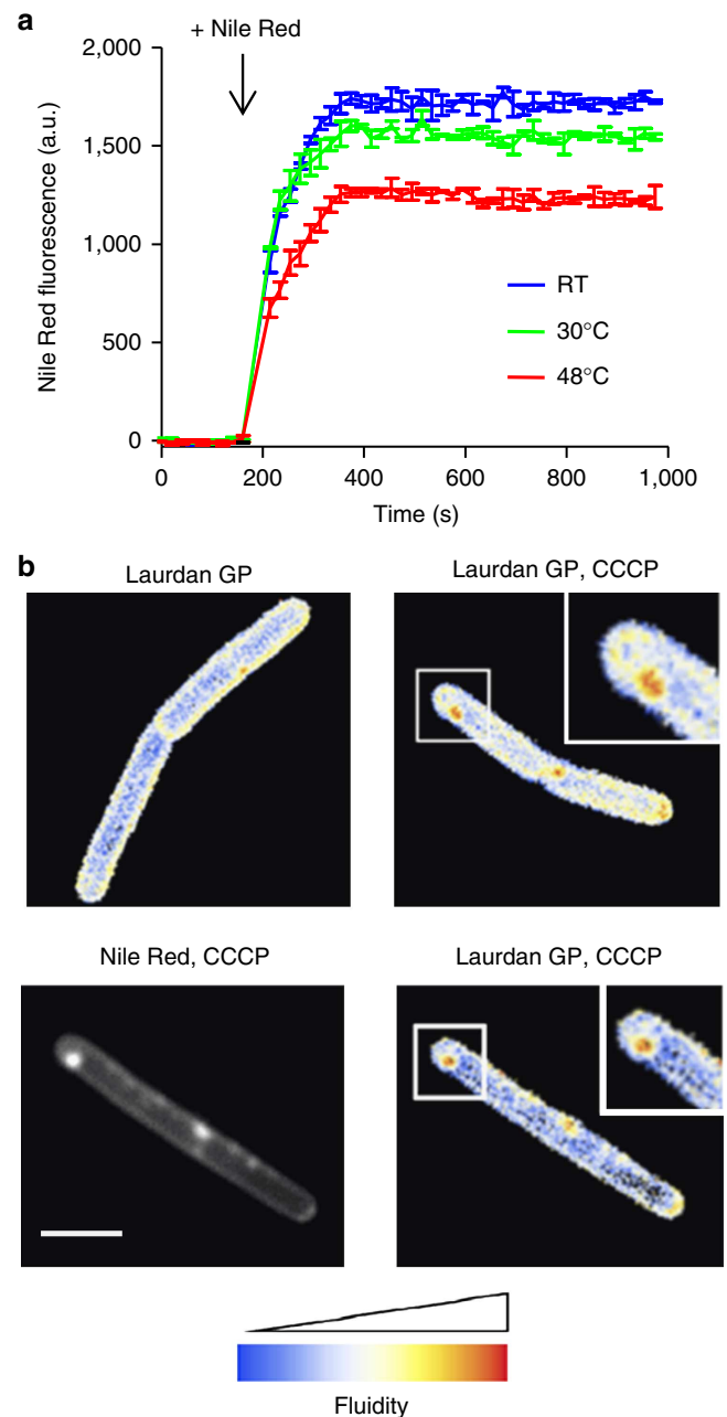
Figure 3 | Analysis of cell membrane fluidity. (a) Nile Red fluorescence intensity of B. subtilis cells grown in room temperature, 30 °C or 48 °C followed by shift to 30 °C, was measured fluorometrically. To prevent rapid adaptation of membrane fluidity 67 , the measurements were carried out with a lipid desaturase ( des )-deficient strain. The curves represent average values with s.d. of three replicate measurements. Strain used: B. subtilis HB5134 ( \Delta des ). (b) Microscopic analysis of fluid membrane domains using Laurdan GP. The images show a colour-coded Laurdan GP intensity map in which red indicates regions of increased fluidity. Membrane fluidity is determined for untreated B. subtilis cells (left panel) and cells treated with CCCP (right panel). See also Supplementary Fig. 10 for the measurement of the average fluidity change. (c) Colocalization of Nile Red foci and Laurdan GP in CCCP-treated B. subtilis cells. Strain used: B. subtilis 168 (wild type). Scale bar, 2 \mu m.
