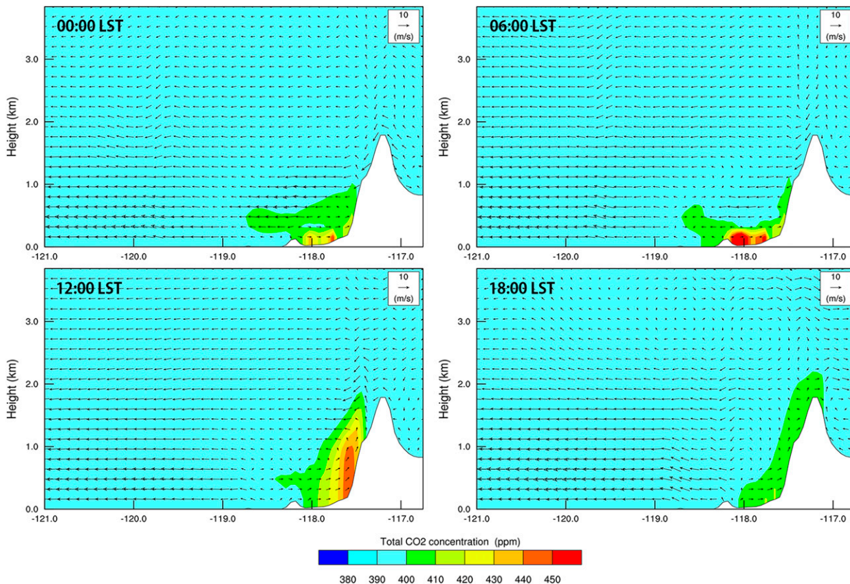
FIG. 4. Vertical cross section of CO 2 concentrations along the line indicated in Fig. 1 for 21 May, displayed in 6-h intervals.
