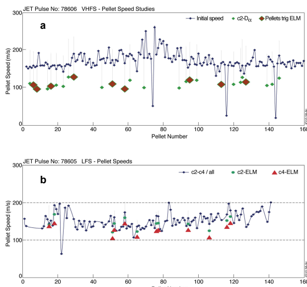
Figure 5 Pellet launch velocity is compared with mean speeds determined from flight times to arrival in the plasma for a) VHFS and b) LFS pellets. Note in both cases less than 1 in 10 pellets launched survive to trigger an ELM.
