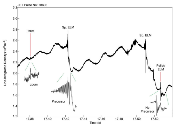
Figure 6 Fast Edge density traces. Only spontaneous ELMs are found to have a short lived n=10 precursor.
