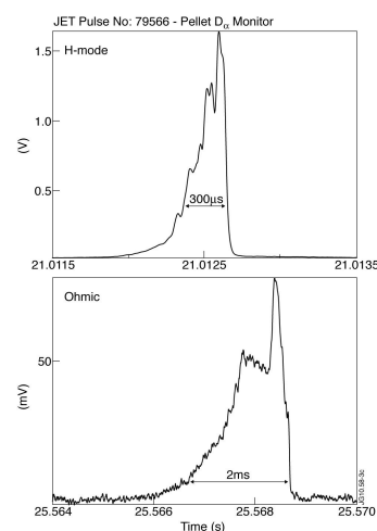
Figure 2 Pellet Ablation in H-mode and Ohmic plasmas
