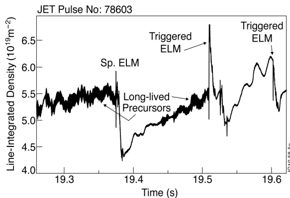
Figure 7 Long lived n=3 precursors are seen in this High Triangularity discharge which can be interrupted by a pellet which triggers an ELM
