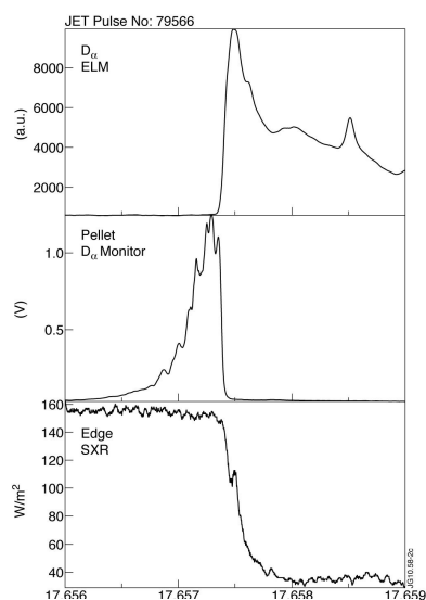
Figure 3. Pellet ELM trigger signals
