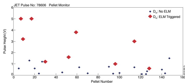
Figure 4. Pellet monitor pulse height against pellet number. Those that trigger an ELM are shown in red and typically are >1\text{V} .
