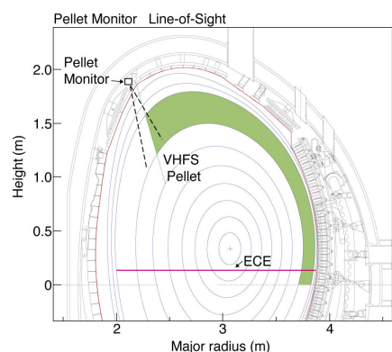
Figure 1. Pellet Monitor Views The mapping of the ablation region to the ECE l.o.s. for Ohmic discharges is indicated in green
