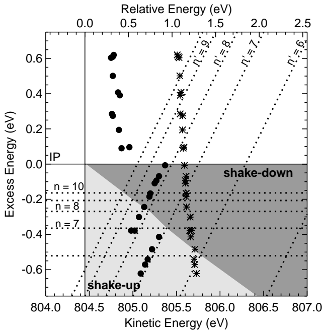
FIG. 3: Behaviour of the center of gravity (asterisks) and the maximum of the spectrum (circles) as a function of photon energy. (See text for explanation.) Horizontal lines mark the excitation energy of some 1snp neutral excited states, and diagonal lines give kinetic energies of relaxation into some 2p^4(1D_2)np' final states. IP designates the experimental Ne 1s ionization potential. Neutral excitation energies ref. [26], final state energies ref. [19].
