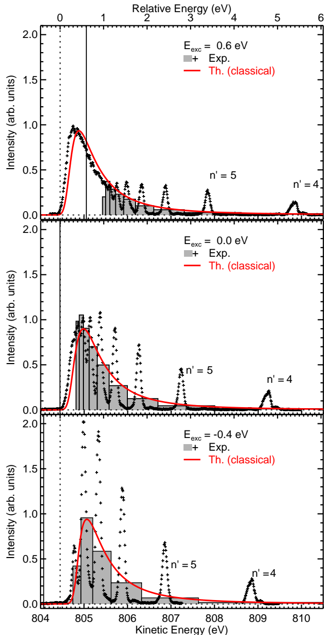
FIG. 1: (Color online) Electron spectra of Ne recorded with excitation energies near to the Ne 1s threshold. The excess energy is indicated in the panels. Discrete lines due to recapture of the photoelectron into a high Rydberg state dominate the spectrum even above the threshold. The gray shaded boxes are drawn as a histogram representation of the experimental spectrum, their areas are proportional to the experimental intensities of the 2p^4(^1D_2)n'p states with n' = 4 - 12 (see text for details). The solid curve is derived from a semi-classical model of PCI-mediated Auger decay [17, 22].
