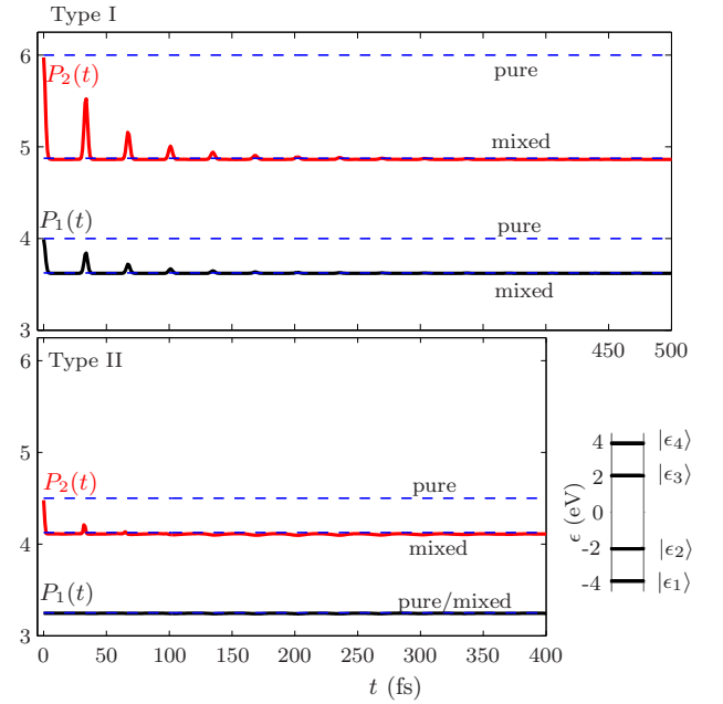
FIG. 2. Reduced purities during the vibronic evolution of a neutral oligoacetylene SSH chain with N = 4 electrons. The system is initially prepared in a superposition |\Psi(0)\rangle = (c_0|\Phi_0\rangle + c_1|\Phi_1\rangle) \otimes |\chi_0\rangle ( |c_0|^2 = 3/4 and |c_1|^2 = 1/4 ) between the ground state |\Phi_0\rangle and an excited electronic state |\Phi_1\rangle . The initial nuclear state |\chi_0\rangle is chosen to be the ground vibrational state associated with |\Phi_0\rangle . Type I: First order coherence, |\Phi_1\rangle = \hat{c}_{\epsilon_3\uparrow}^\dagger \hat{c}_{\epsilon_2\uparrow} |\Phi_0\rangle . Type II: Second order coherence, |\Phi_1\rangle = \hat{c}_{\epsilon_3\downarrow}^\dagger \hat{c}_{\epsilon_2\downarrow} \hat{c}_{\epsilon_3\uparrow}^\dagger \hat{c}_{\epsilon_2\uparrow} |\Phi_0\rangle . The dashed lines signal the fully coherent/incoherent limit of P_1 and P_2 computed using Eqs. (19) and (21) assuming that only |\Phi_0\rangle and |\Phi_1\rangle participate in the dynamics. The orbital labels and energies at initial time are shown in the bottom-right corner.
