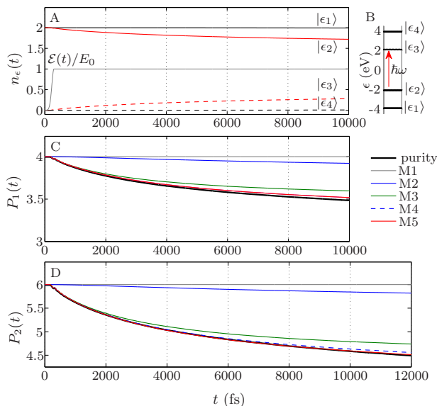
FIG. 3. Reduced purities during photoexcitation of a neutral SSH chain with 4 electrons. (A) Orbital populations during photoexcitation with a laser field E(t) = \mathcal{E}(t) \cos(\omega t) . The laser frequency \hbar\omega = 4.08 eV is chosen to be at resonance with the HOMO-LUMO transition. The envelope function \mathcal{E}(t) has a Gaussian turn-on and remains constant at E_0 = 8.7 \times 10^{-3} V/Å from t = 300 fs on. (B) Single-particle spectrum of the SSH chain at initial time. (C) One-body and (D) two-body purity during the dynamics. The black lines are the result of an explicit simulation of the vibronic dynamics. The colored lines correspond to different models with varying degrees of coherence assumed in the N -body density matrix (see text). In (C) the lines for M3 and M4 are on top of each other and cannot be distinguished.
