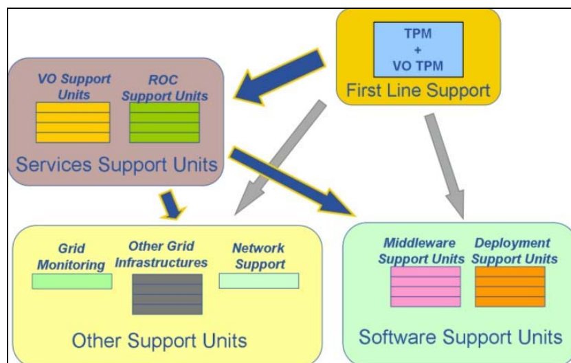
Figure 4: Support units in GGUS and main workflows
