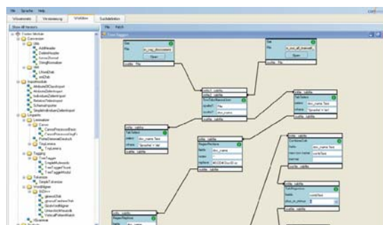
Figure 11: ConWeaver workbench - data analysis workflow
