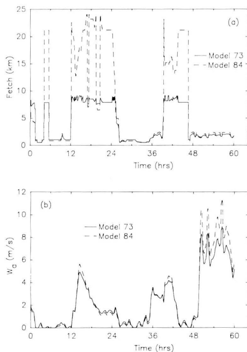
Fig. 3. Time histories of fetch and W_a used in each wave hindcasting model for the data set measured at the Keszthely field site.
