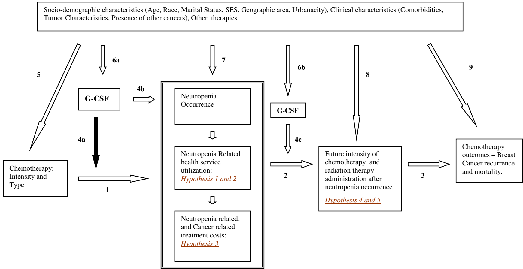
Figure 3 Conceptual framework
