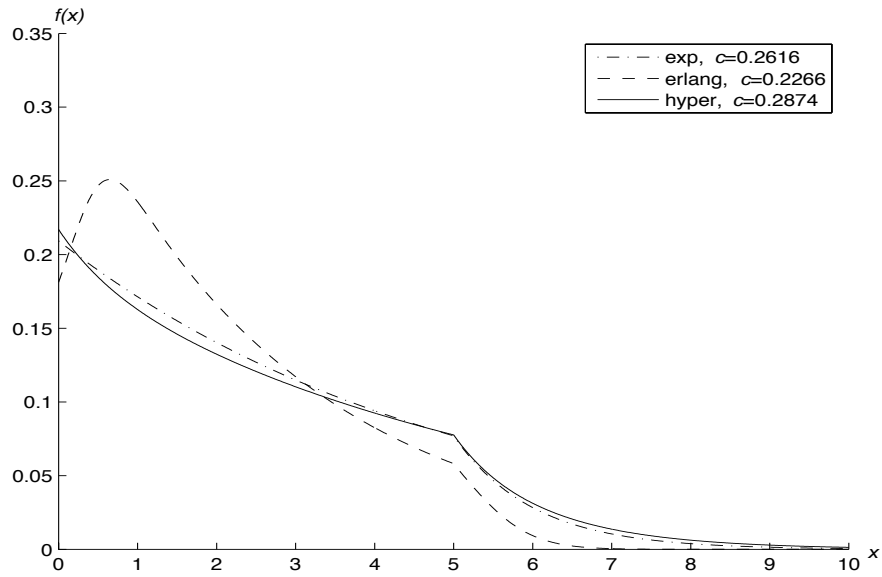
Figure 2.3: f(x) for different service time distributions, \rho = 0.8, b = 5
