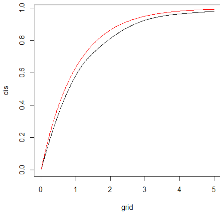
Figure 3.6: Distribution Estimation, p = 0.3
