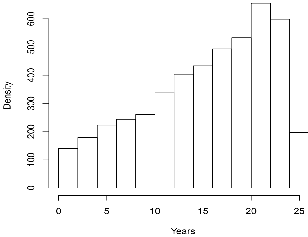
Figure 3.9: Histogram of the uncensored observations in the ARIC data.
