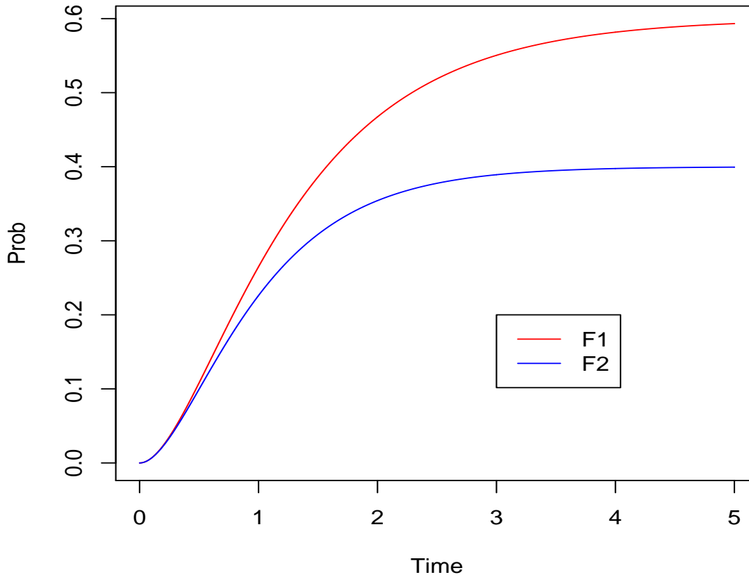
Figure 4.1: Example of Subdistributions
