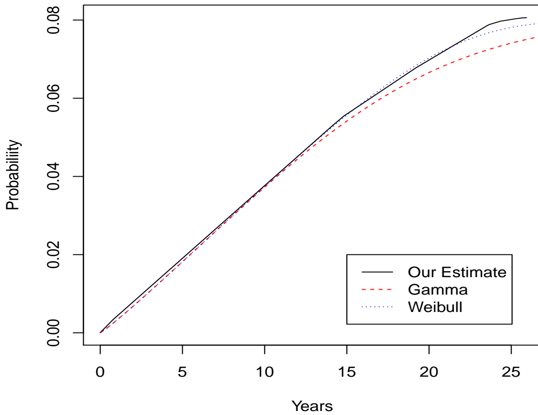
Figure 4.4: Estimates of the Subdistribution of MI for the ARIC Data.
