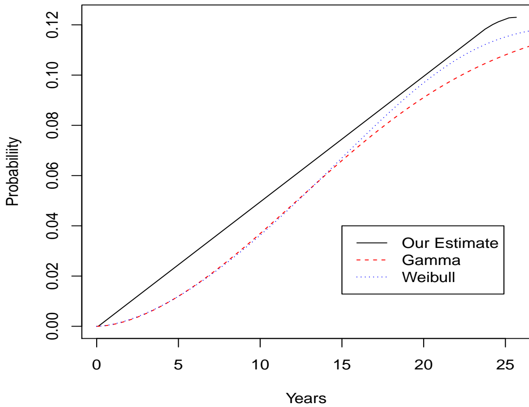
Figure 4.3: Estimates of the Subdistribution of Heart Failure for the ARIC Data.
