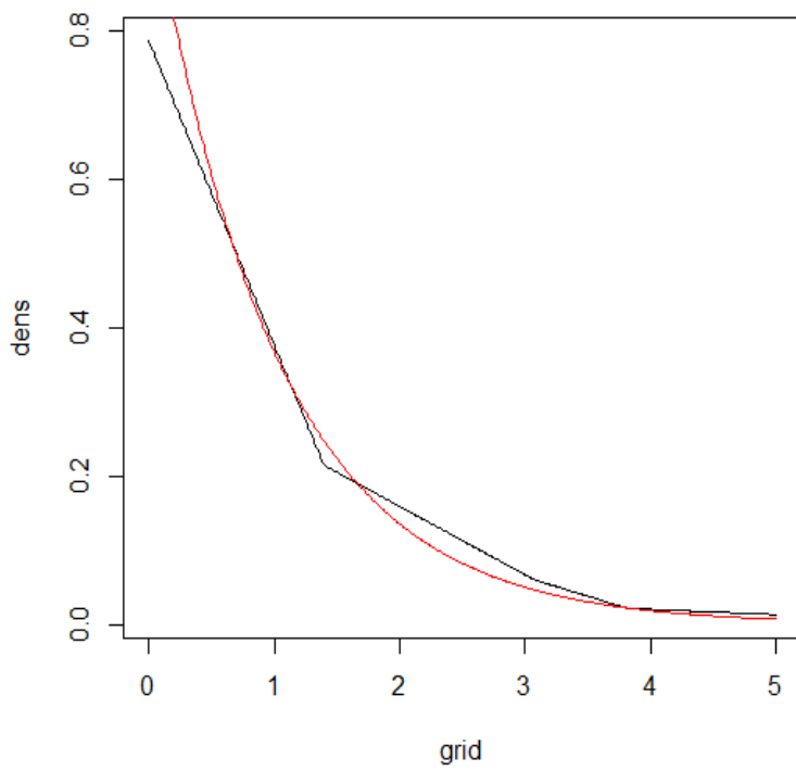
Figure 3.5: Density Estimation, p = 0.3
