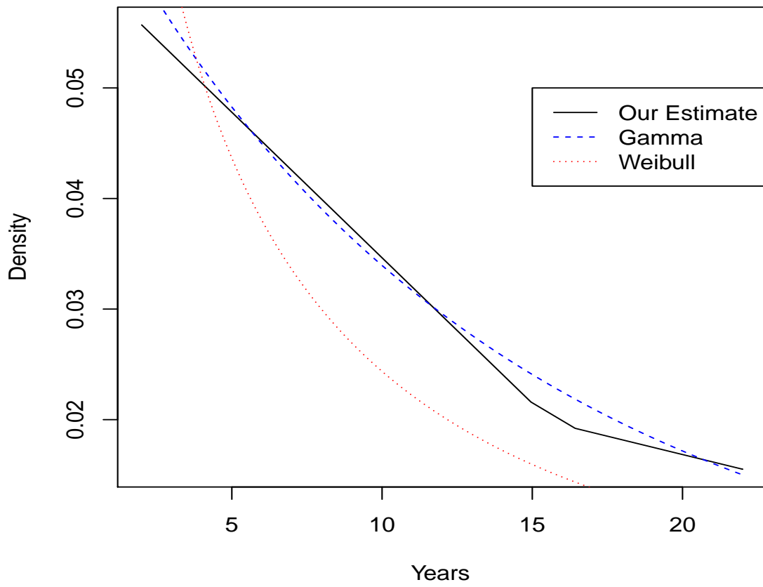
Figure 3.8: Density Estimates for the ARIC data in the Presence of Censoring.
