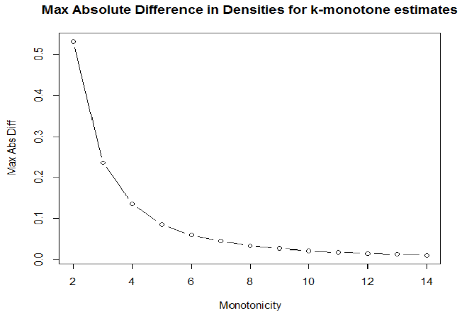
Figure 3.3: k-monotone Density Estimates for the Exponential Distribution.
