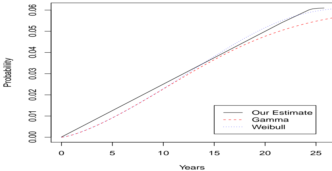
Figure 4.2: Estimates of the Subdistribution of Stroke for the ARIC Data.
