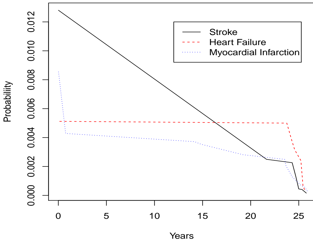
Figure 4.5: Subdensity Estimates for the three competing risks based on our method.
