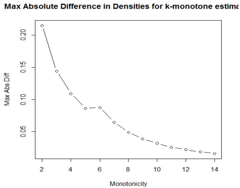
Figure 3.4: Obtaining k-monotone Density Estimates for a 5-Monotone Density.
