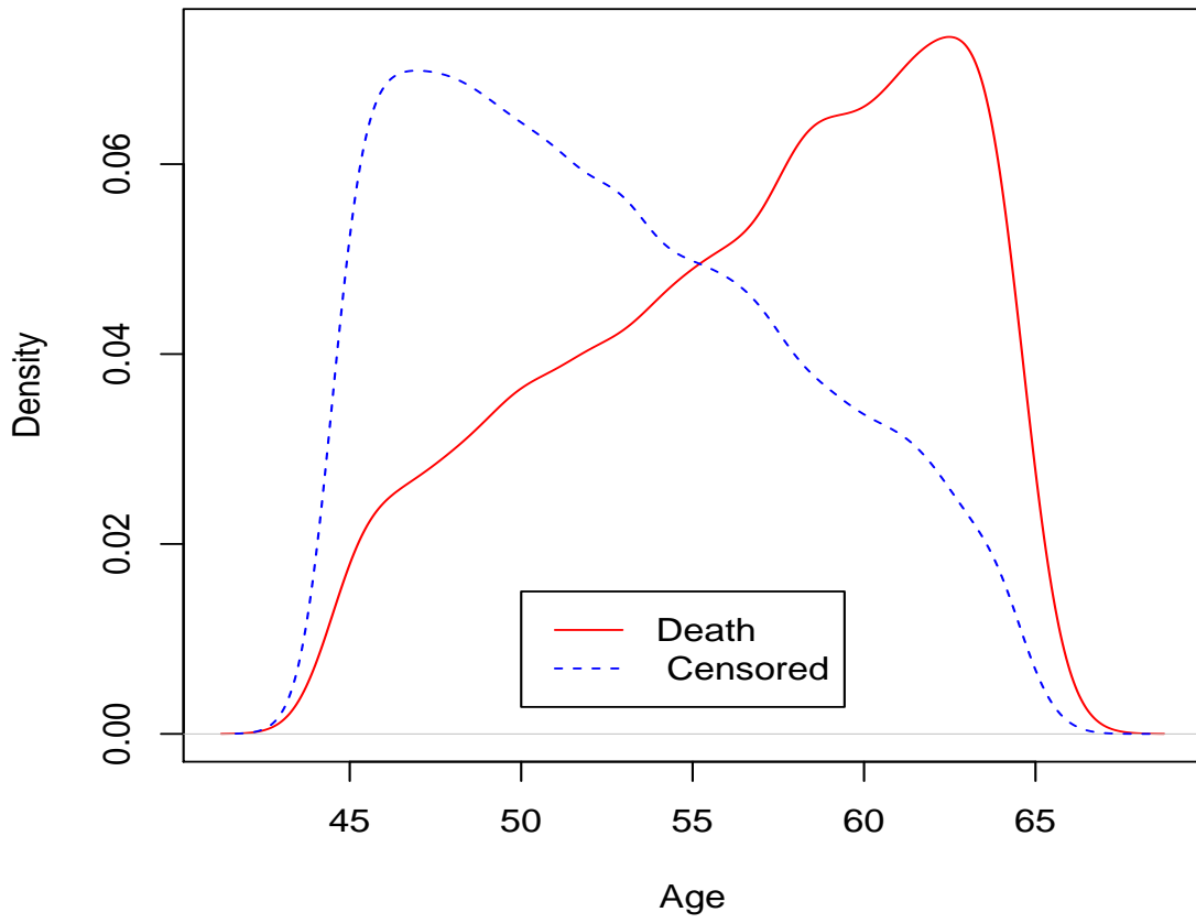
Figure 3.7: Distribution of Age in the Two Groups.
