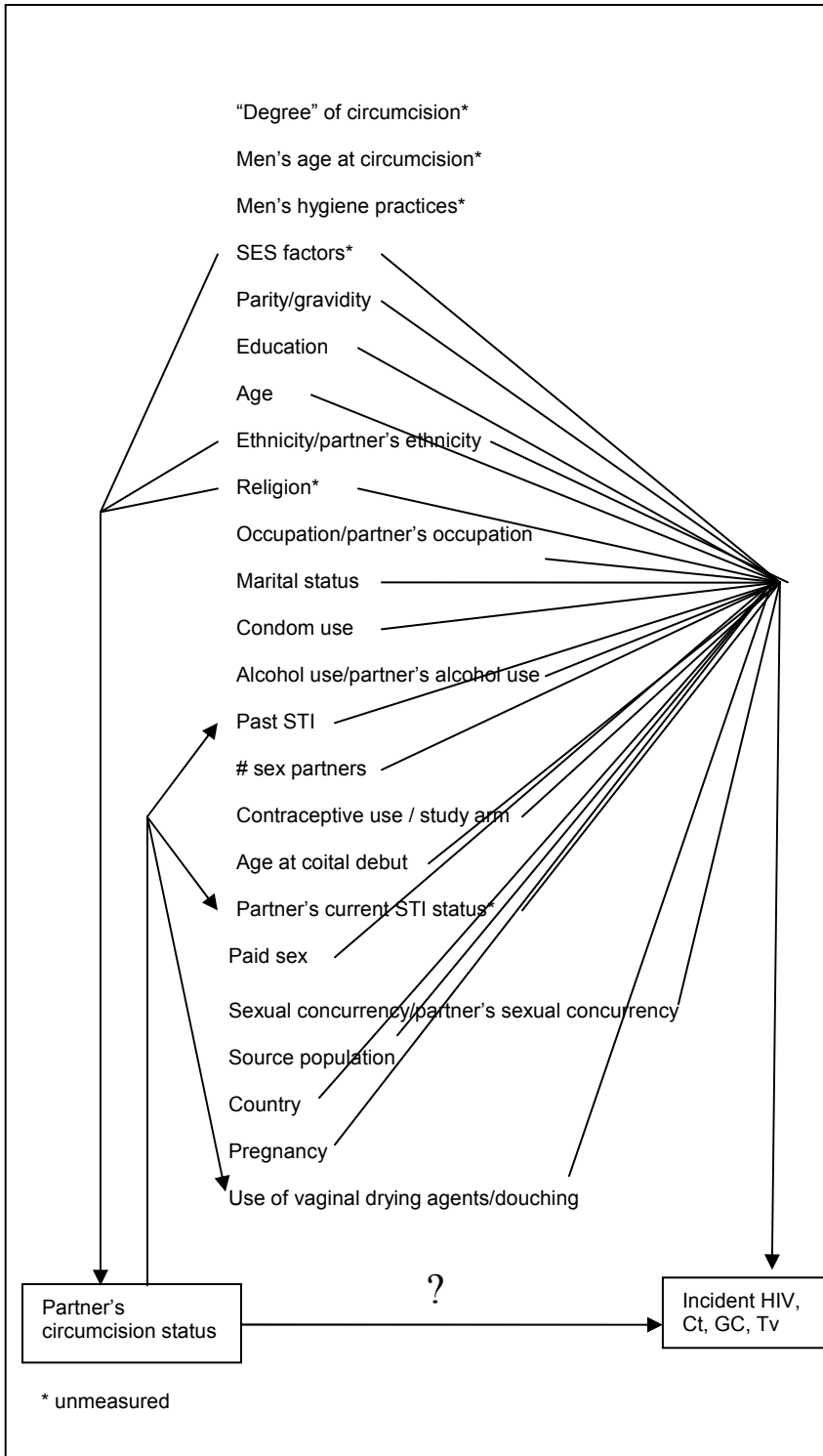
FIGURE 3.1. Causal model for male circumcision and women’s risk of acquisition of HIV/STI (Aim 1).
