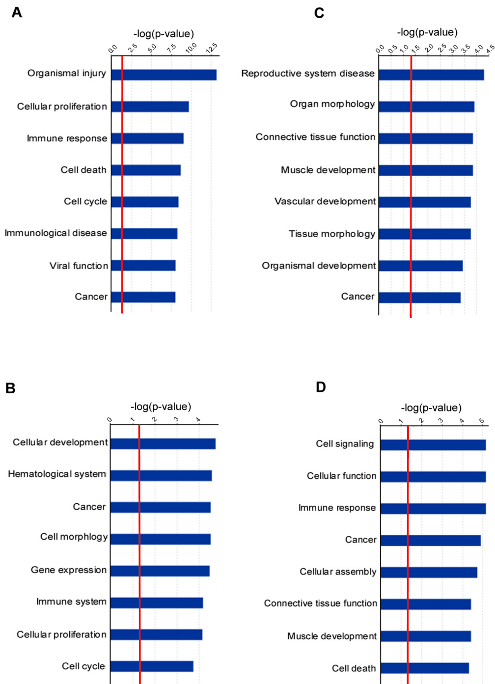
Figure 2 Top functions affected as a result of altered gene expression. Functions determined by: A. Up-regulated genes after NASP overexpression. B. Down-regulated genes after NASP overexpression. C. Up-regulated genes after NASP depletion. D. Down-regulated genes after NASP depletion. Bars represent -\log(p\text{-value}) for disproportionate representation of affected genes in the total number of genes in the selected function/disease category. Threshold (red line) denotes the p = 0.05 level.
