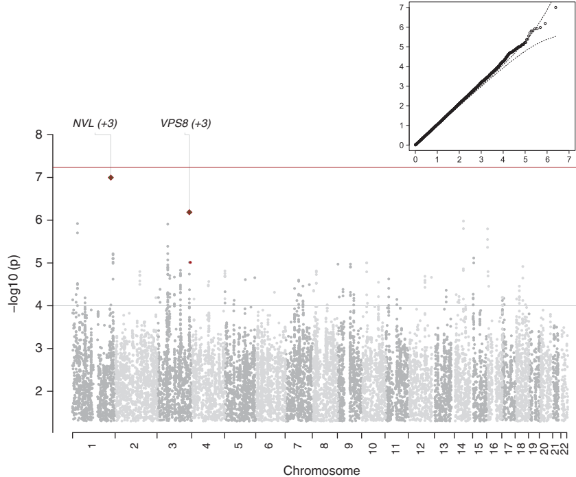
Figure 1 Overview of results from the discovery genome-wide association study mega-analysis for major depressive disorder. The inset shows the quantile–quantile plot (observed by expected P -values on the -\log_{10} scale) showing conformity of the observed results to expectations under the null. The main part of the figure shows the Manhattan plot ( -\log_{10} of the P -value by genomic location) of the association results in genomic context. No region exceeded genome-wide significance in the discovery sample.
