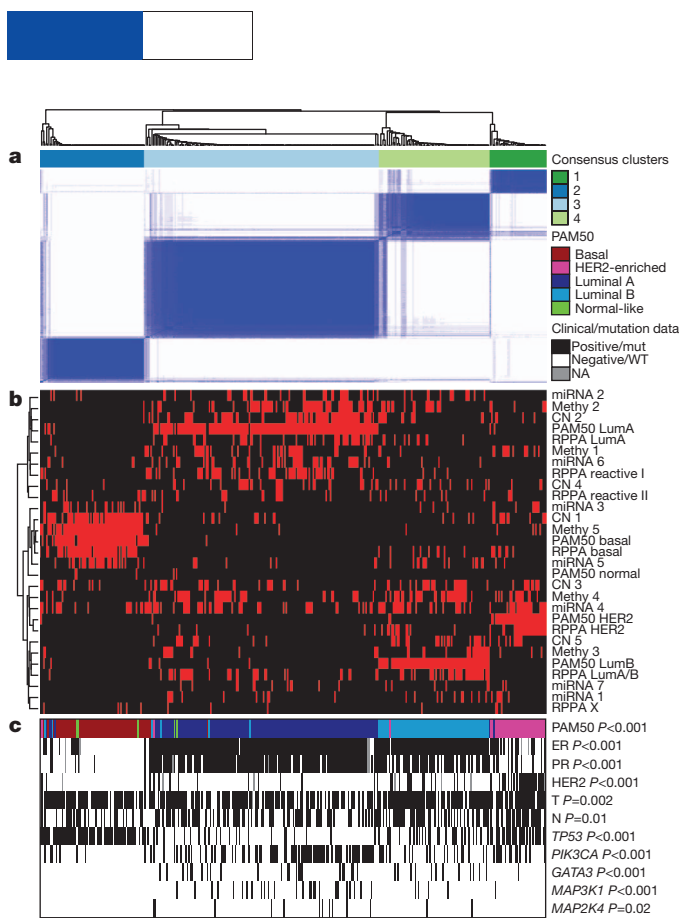
Figure 2 | Coordinated analysis of breast cancer subtypes defined from five different genomic/proteomic platforms. a , Consensus clustering analysis of the subtypes identifies four major groups (samples, n = 348 ). The blue and white heat map displays sample consensus. b , Heat-map display of the subtypes defined independently by miRNAs, DNA methylation, copy number (CN), PAM50 mRNA expression, and RPPA expression. The red bar indicates membership of a cluster type. c , Associations with molecular and clinical features. P values were calculated using a chi-squared test.
