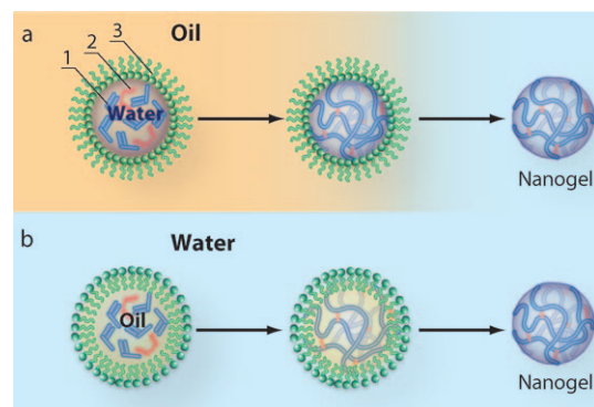
Figure 2. Chemical synthesis of nanogels by copolymerization in colloidal environments. a) Copolymerization of monomers (1) and bifunctional cross-linkers (2) in w/o microemulsions stabilized by surfactants (3) produces nanogels that can then be transferred into aqueous media after removal of the surfactants and organic solvent. b) Copolymerization reactions can also be carried out in o/w emulsions that can be additionally stabilized by surfactants.
