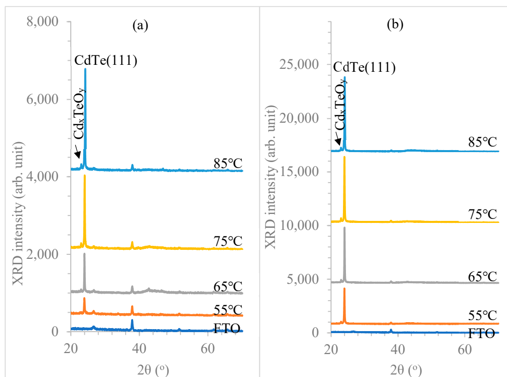
Figure 3. XRD patterns of CdTe thin-films electroplated at different temperatures under (a) as-deposited (AD) and (b) cadmium chloride treated (CCT) conditions.
