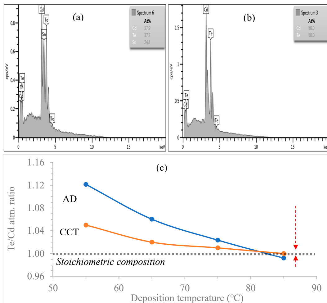
Figure 9. EDX spectra of CdTe grown from the 85 °C electrolyte under (a) AD, (b) CCT conditions (c) is the graphical summary of Te/Cd atomic composition ratio against electroplating temperature of CdTe for both AD and CCT samples.
