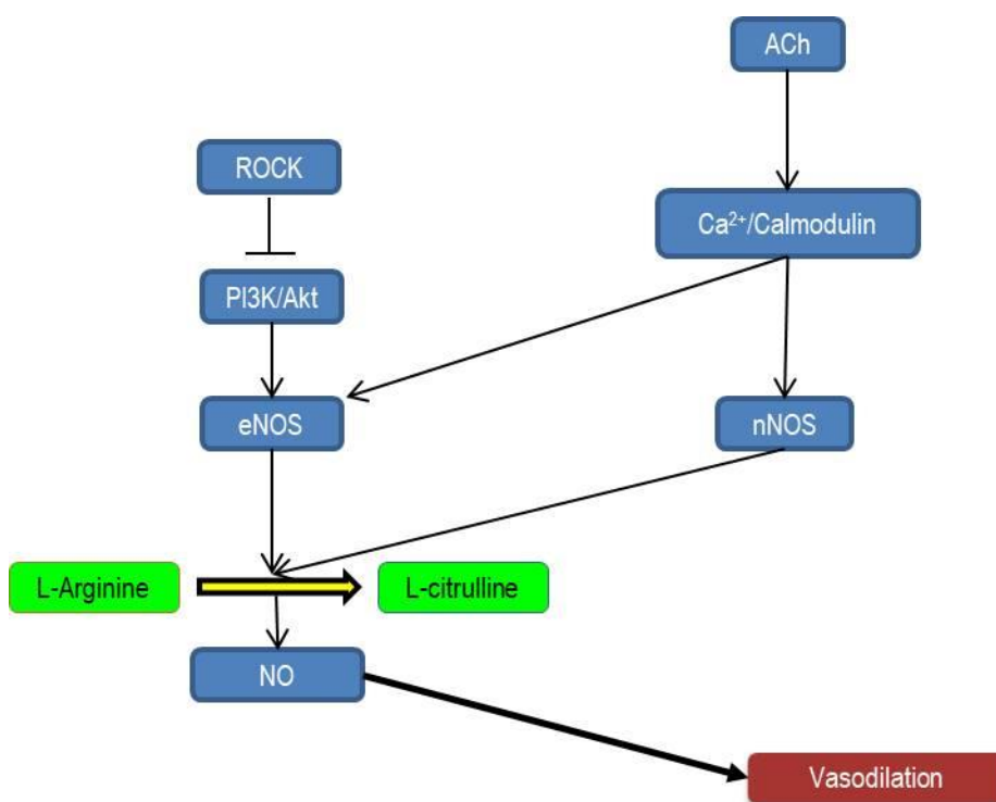
Figure 1.3 The NO pathway
