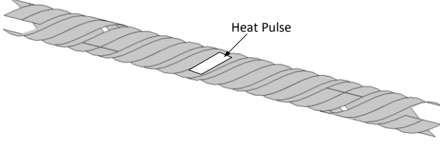
Fig. 1. Geometry of the single-layer CORC cable with three ReBCO tapes and the heat pulse zone.
