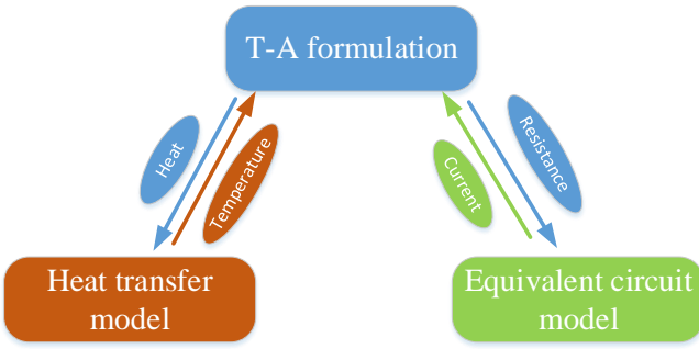
Fig. 2. Numerical algorithm of the 3D quench model
