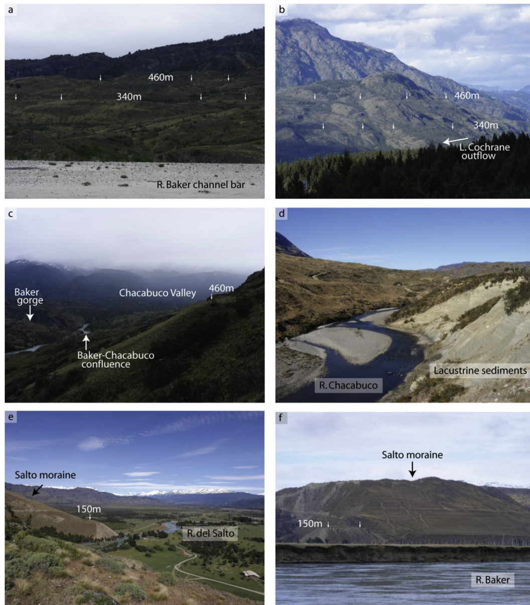
Fig. 7. Photographs of palaeolake landforms. (a) The 460 and 340 m asl shorelines, taken from a channel bar of the Río Baker, downstream of the Maiten valley (Fig. 6a). (b) The 460 and 340 asl shorelines above the Lago Cochrane outflow (Fig. 6c). (c) View upstream towards the Baker-Chacabuco confluence showing the 460 masl shoreline cut into the top of glacial diamicton blanketing the valley side (Fig. 6b). (d) Laminated glaciolacustrine sediments in the lower Chacabuco valley (Fig. 6a). (e) View westwards of a raised delta at ~150 m asl at the exit of Río del Salto in to Valle Grande (Fig. 6a). (f) View of the ~150 m asl raised delta in Valle Grande from the Río Baker. Note the shorelines cut into the ice distal side of the Salto moraine. Photos by V.R. Thorndyraft.
