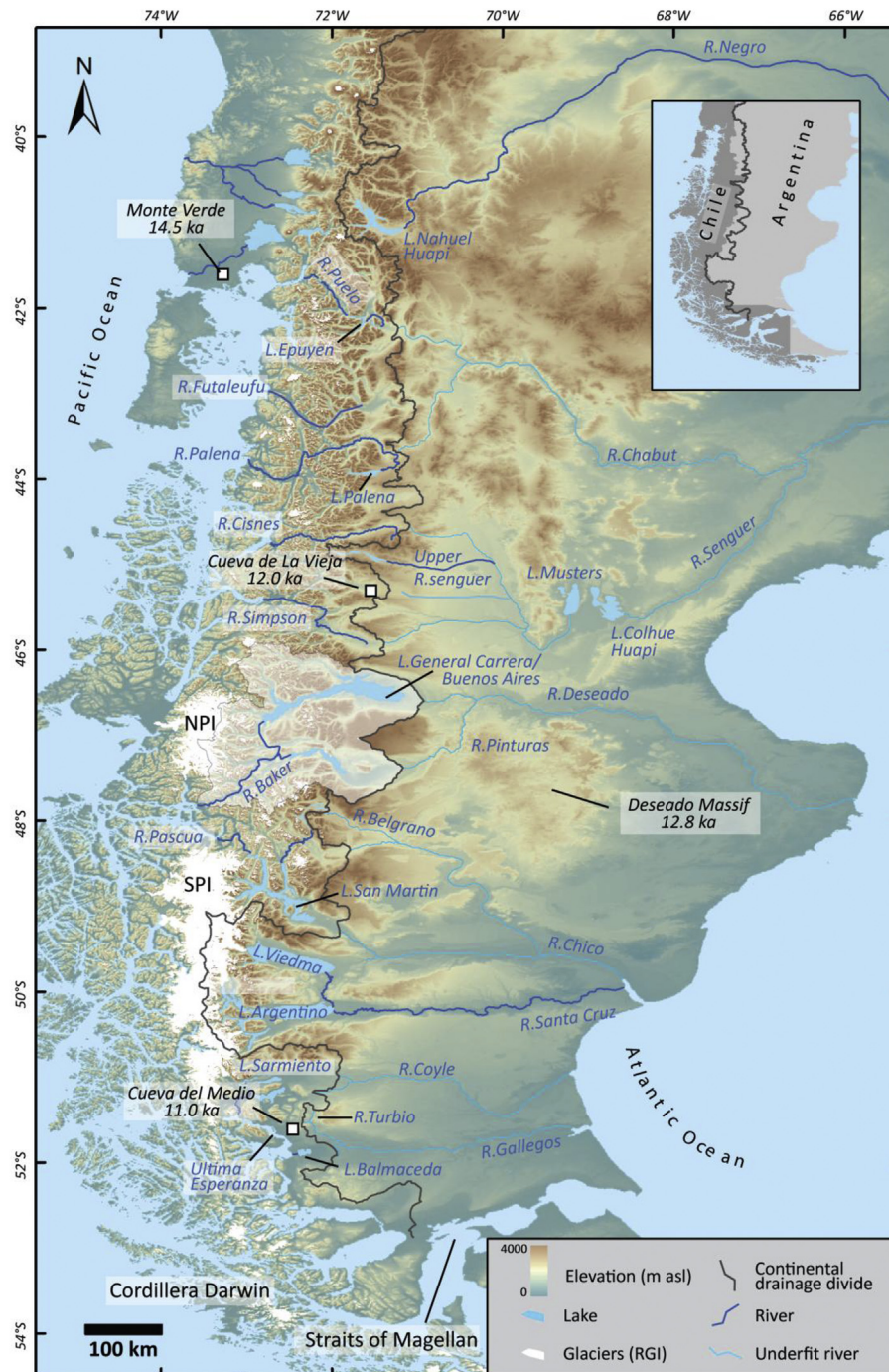
Fig. 16. Map of continental-scale drainage reversals across Patagonia and selected archaeological sites. The main drainage pathways, which experienced Atlantic-Pacific drainage reversals during PIS deglaciation, are shown by the underfit river valleys. Only ríos Negro, Santa Cruz and the upper Senguer maintained an Atlantic drainage pathway. The continental drainage divide is based on the USGS hydrosheds database (30 s South America drainage basin shapefiles). The location of the Río Baker catchment (this study) is shown. North of 46°S, ríos Simpson, Cisnes and Futaleufu drain valleys with now disappeared palaeolakes. A major river capture event also took place at ~50°S where Lago Viedma drained to Lago Argentino and Río Santa Cruz, abandoning its Río Chico pathway to the Atlantic. Contemporary glacier extent is from the Randolph Glacier Inventory. Inset: Map of Chile, Argentina and the continental drainage divide.
