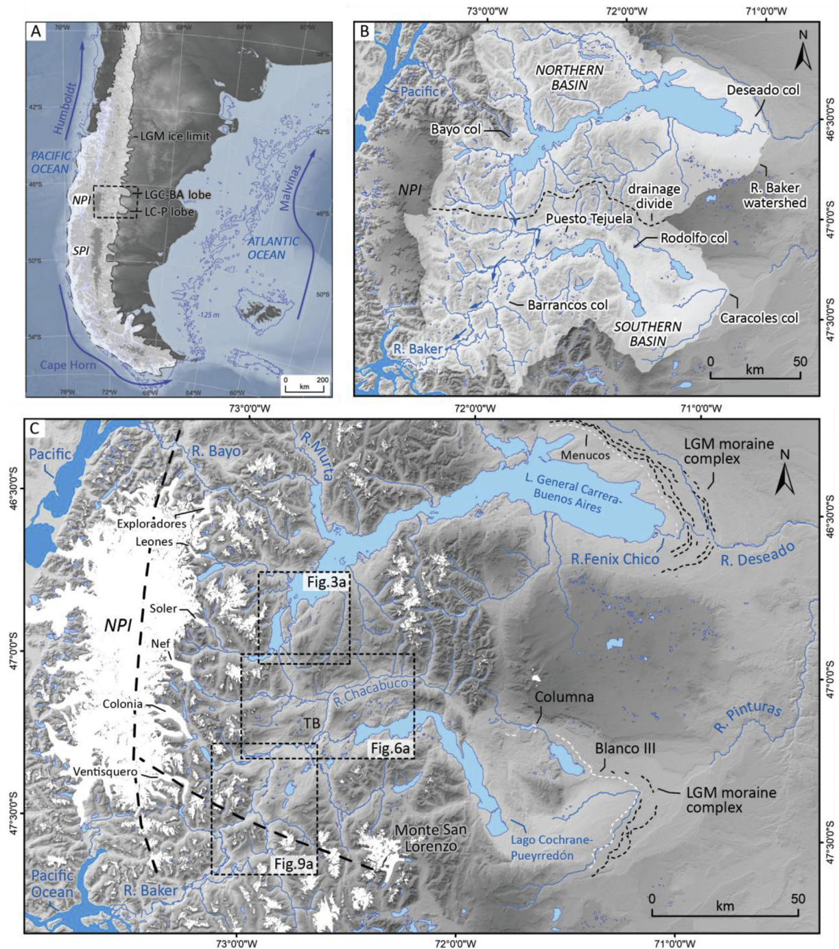
Fig. 1. (a) The study area in southern South America with the LGM ice limit of the former Patagonian Ice Sheet (PIS) (Bendle et al., 2017a) and principal ocean currents shown. (b) The Río Baker catchment, divided into northern and southern basins as used in the text. Blue arrows indicate river flow direction. Also shown are the major palaeolake outflow cols discussed in the text. (c) Regional map showing the spatial context of the main field study areas to the Northern Patagonian Icefield (NPI) and the basins of Lago General Carrera/Buenos Aires (LGC-BA) and Lago Cochrane/Puerreydón (LC-P), the two lakes hypothesised to join through the Baker Valley in the Tamango Basin (TB) sector. Contemporary glaciers (Randolph Glacier Inventory) are shown in white, highlighting both the NPI and Monte San Lorenzo (MSL) ice cap. Also shown are the LGM limits (dotted lines) associated with the main eastward flowing ice-lobes of the PIS, and the LGM ice divides (black dashed lines) from Hubbard et al. (2005). Dates from the youngest moraines (white dotted line) are used in our geochronological review.
