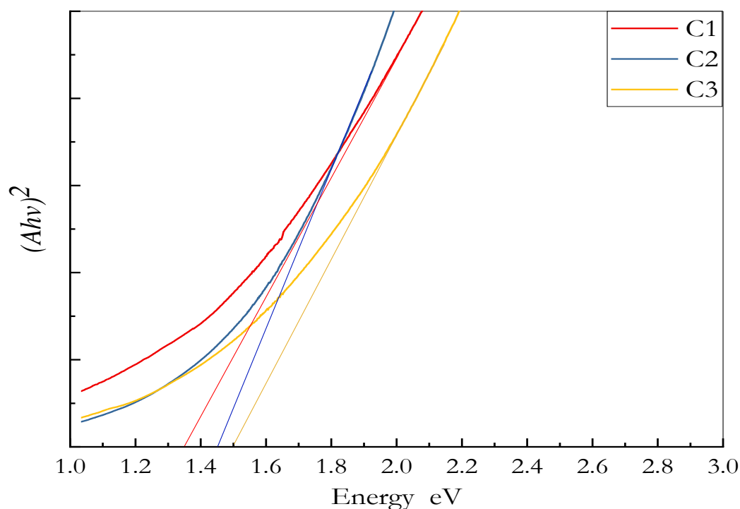
Figure 5.4 Band gap for different Cu content samples from Tauc plot.
