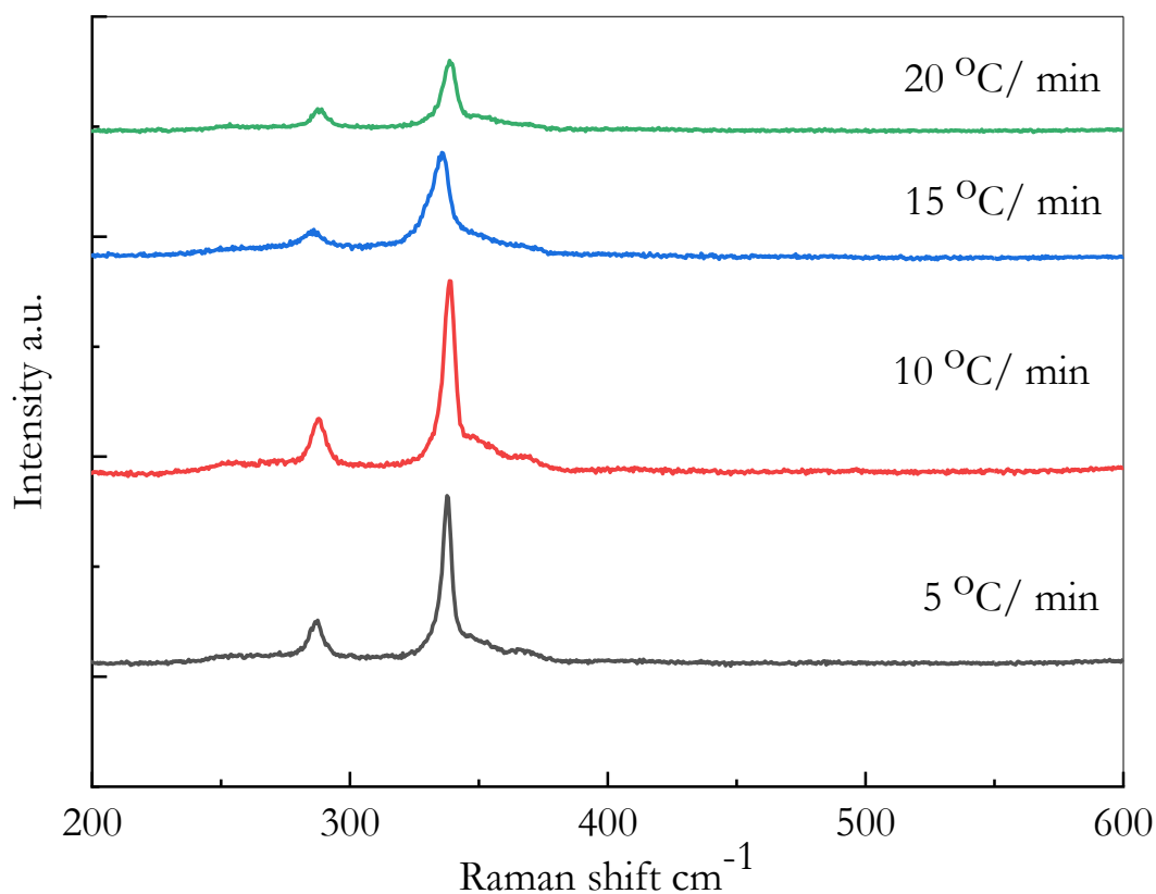
Figure 6.8 Raman measurements of CZTS films at different annealing ramping rate 5, 10, 15 and 20 °C/min at 500 °C.
