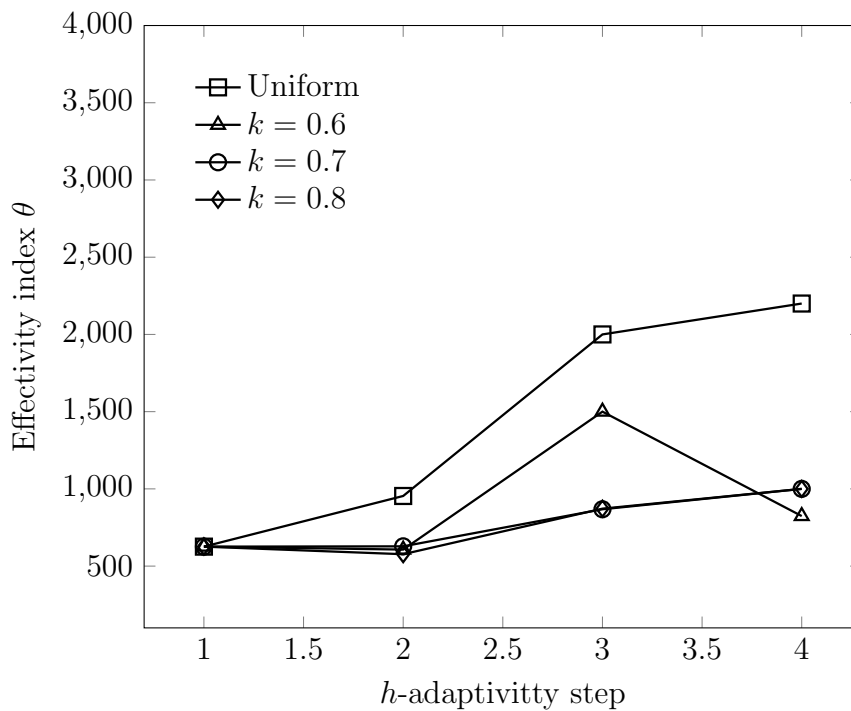
Figure 5.6: The effectivity index \theta using h -adaptivity of the one-dimensional bar problem for the analyses with different k .
