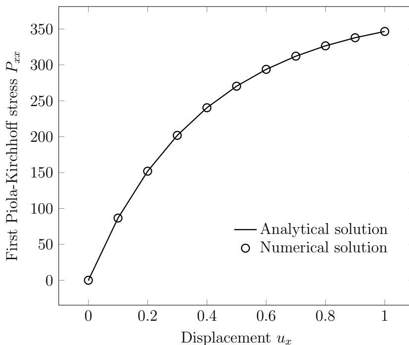
Figure 5.4: First Piola-Kirchhoff stress P_{xx} against displacement u_x of the one-dimensional bar problem.
