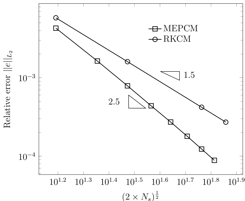
Figure 3.21: Convergence rate of \|e\|_{L_2} in the two-dimensional elasticity problem: a confined square domain using the MEPCM and the RKCM.
