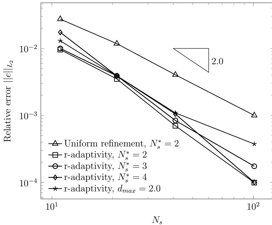
Figure 4.5: Convergence rate of \|e\|_{L_2} of the one-dimensional bar problem using uniform refinement and r -adaptive strategy with various N_s^* .
