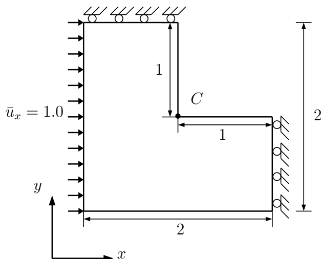
Figure 4.18: The L-shaped plate with a uniform displacement on the left edge.
