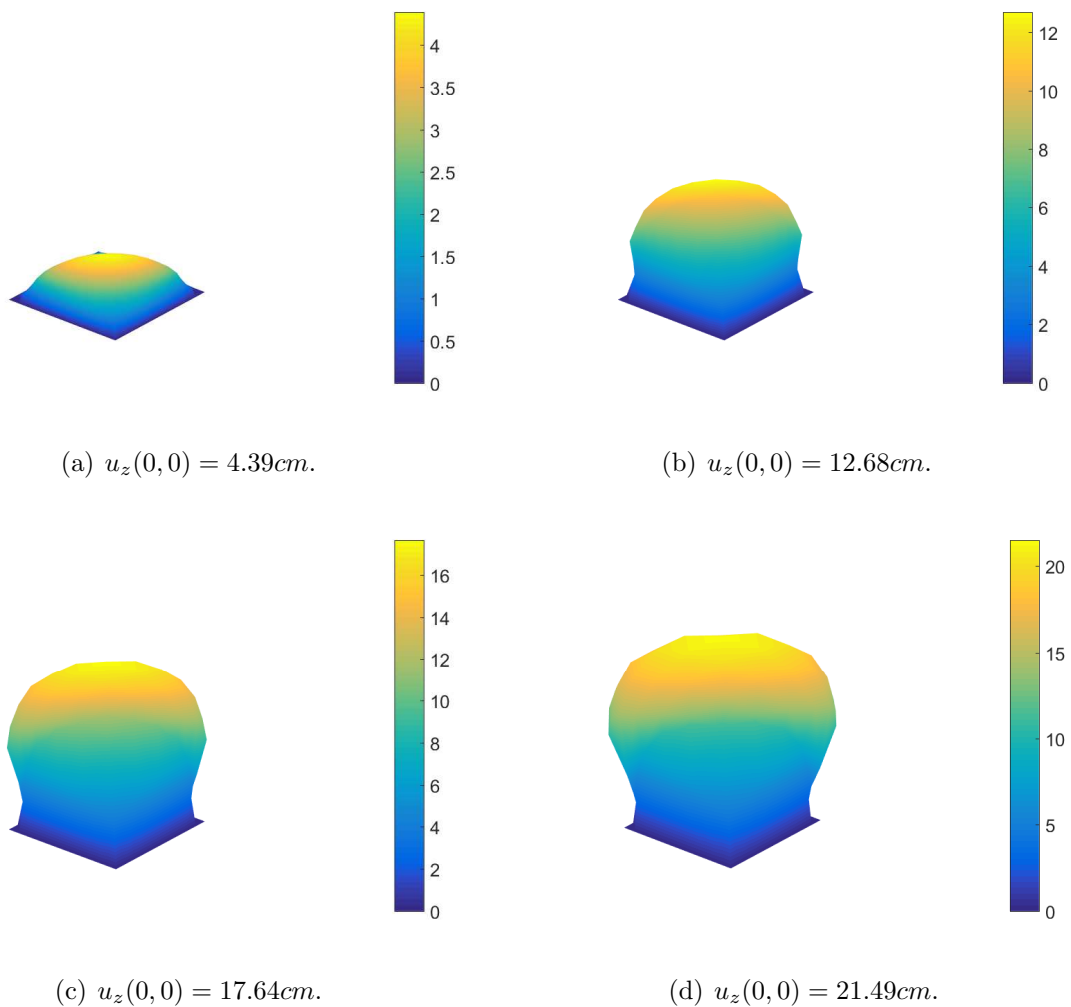
Figure 6.11: The deformed configurations with the out-of-plane displacement, u_z (cm) at different load steps of the square hyperelastic membrane problem subjected to a uniform pressure.
