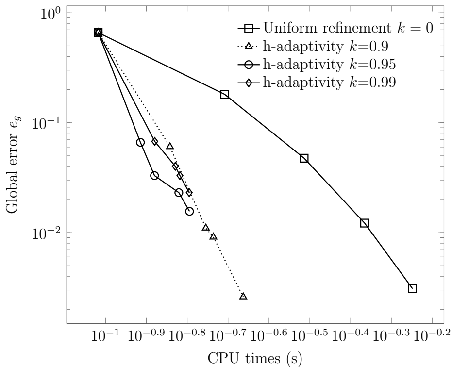
Figure 4.12: Convergence rate of e_g against CPU time of the one-dimensional bar problem using different k with N_s^* = 2 .
