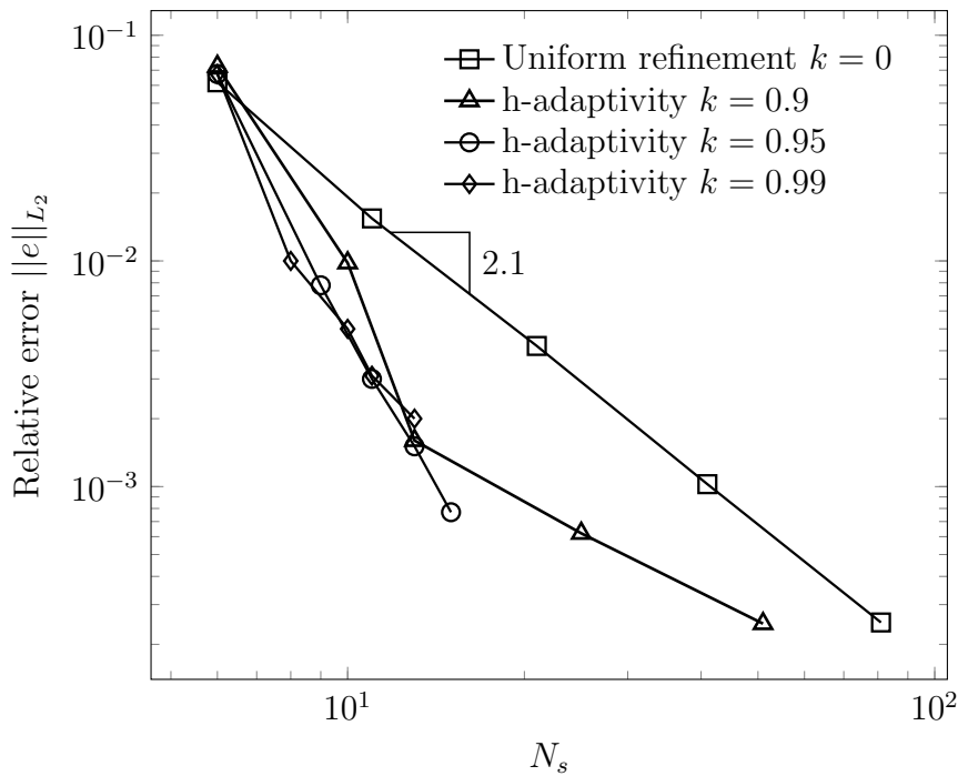
Figure 4.10: Convergence rate of \|e\|_{L_2} of the one-dimensional bar problem using different k with N_s^* = 2 .
