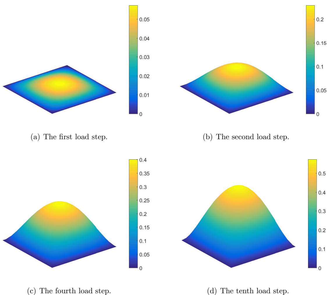
Figure 6.6: The deformed configurations with the out-of-plane displacement, u_z (m) at different load steps of the initially flat linear elastic membrane problem subjected to a uniform pressure.
