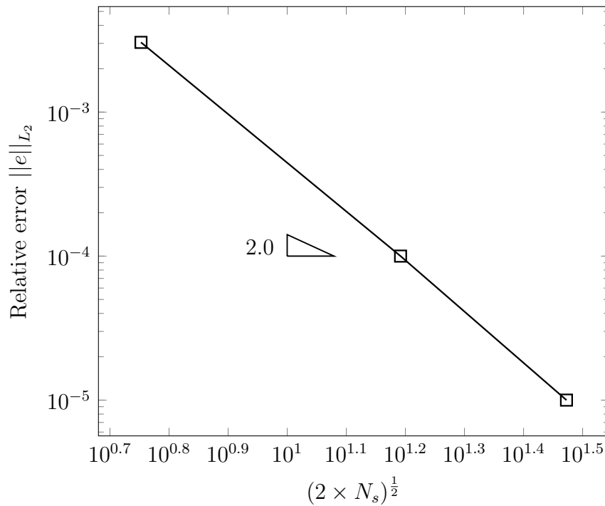
Figure 5.10: Tension of a two-dimensional square domain: convergence rate of \|e\|_{L_2} with uniform refinement.
