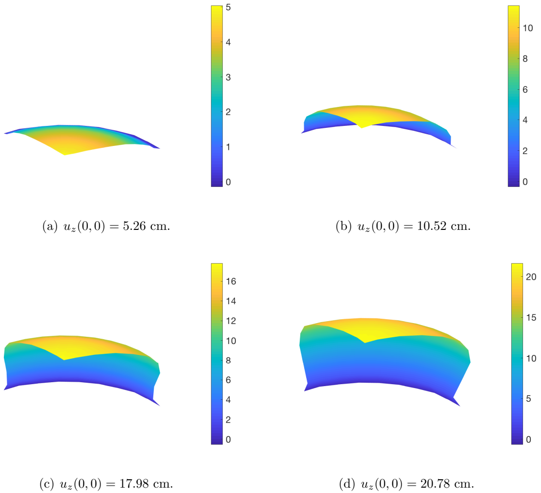
Figure 6.17: The deformed configurations with the out-of-plane displacement, u_z (cm) at different load steps of quarter of the circular hyperelastic membrane subjected to a uniform pressure.
