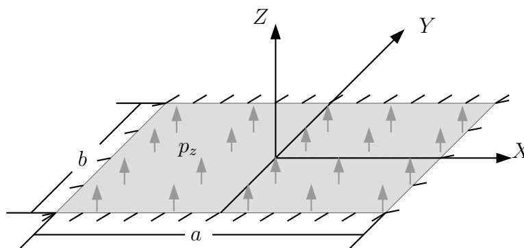
Figure 6.5: An initially flat linear elastic membrane model subjected to a uniform pressure.
