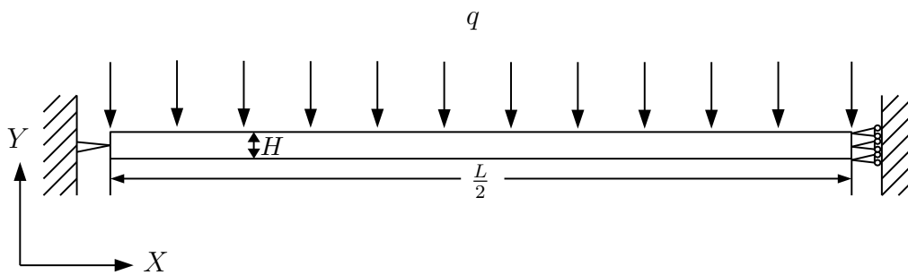
Figure 5.21: Geometry of the plate with uniformly distributed load, q , and simple supported ends
