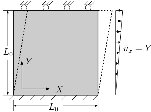
Figure 5.11: Geometry of a two-dimensional square domain under simple shear.
