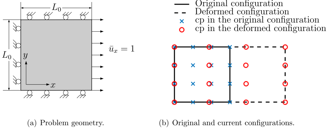
Figure 5.8: Tension of a two-dimensional square domain: geometry and configurations.
