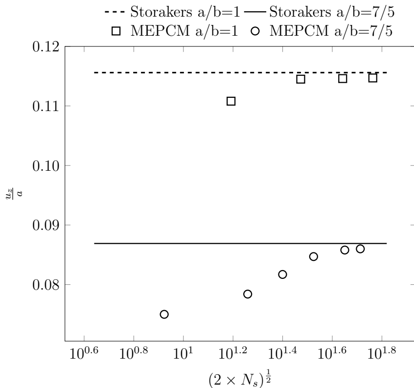
Figure 6.9: The normalised deflection u_z/a at the centre point against the number of degrees of freedom of the initially flat linear elastic membrane problem subjected to a uniform pressure.
