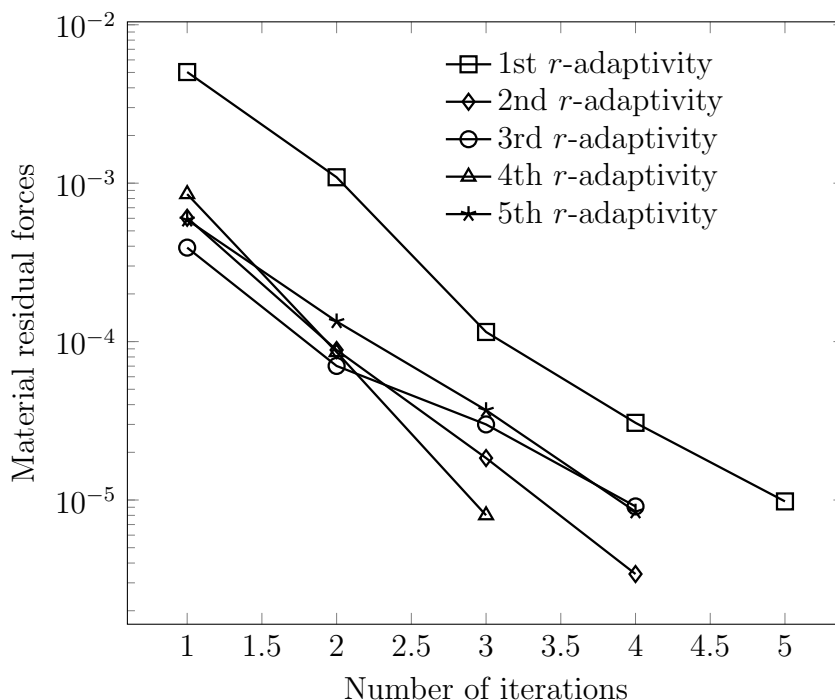
Figure 4.21: Material force residuals in the iteration process of the L-shaped plate with k = 0.3 .
