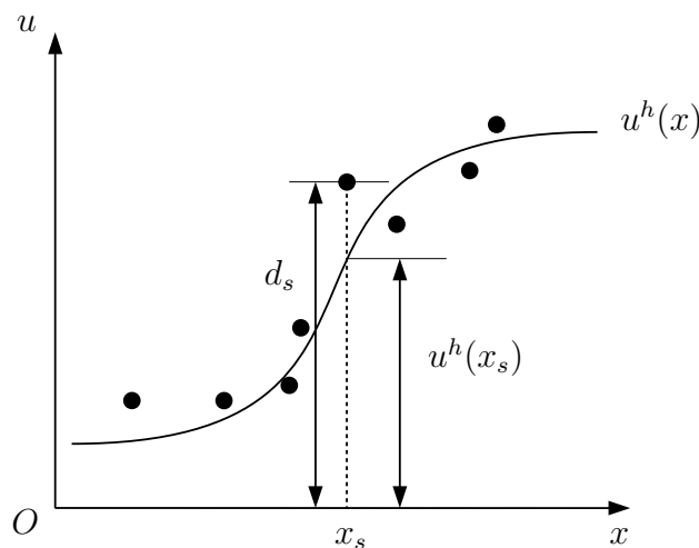
Figure 3.3: Moving least squares approximations in one dimension.
