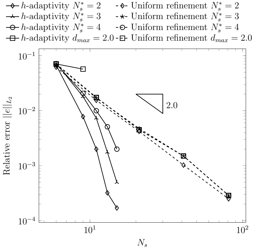
Figure 4.8: Convergence rate of \|e\|_{L_2} of the one-dimensional bar problem using different N_s^* with k = 0.95 .
