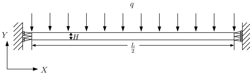
Figure 5.18: Geometry and boundary conditions of the plate with uniformly distributed load, q and fixed at two ends.
