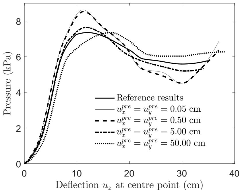
Figure 6.12: Pressure versus deflection at central point of the square hyperelastic membrane problem subjected to a uniform pressure.
