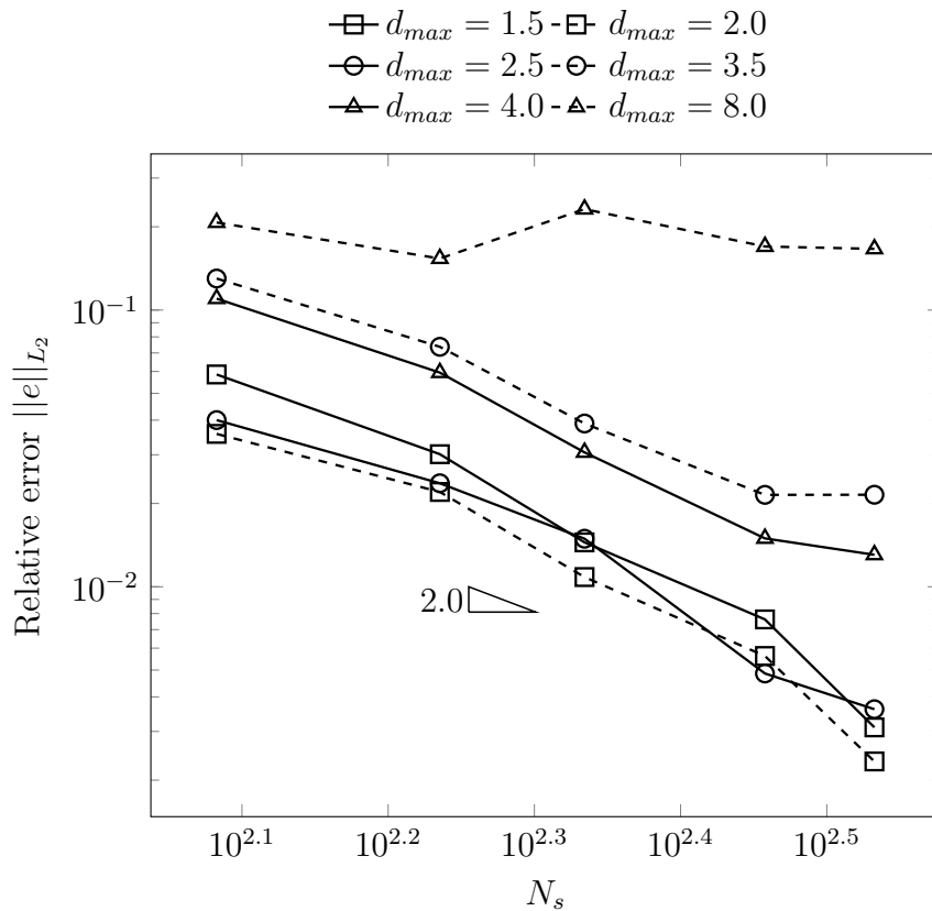
Figure 3.9: Convergence rate of \|e\|_{L_2} of the one-dimensional bar problem using the MEPCM with different d_{max} .
