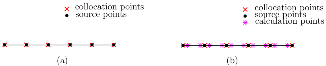
Figure 4.7: The collocation, source and calculation points generation in h -adaptivity of the one-dimensional bar problem.
