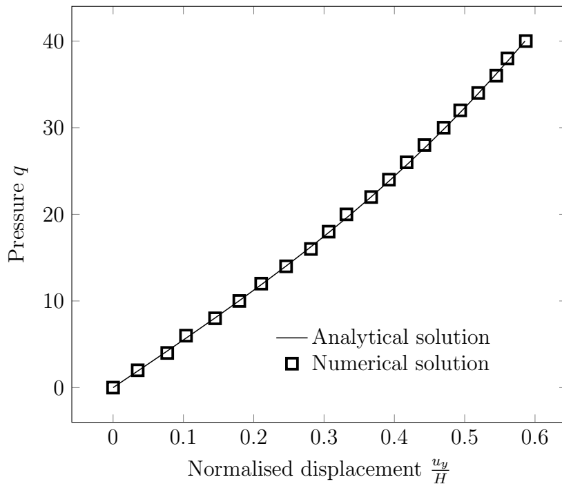
Figure 5.20: Pressure versus normalised displacement of the plate with uniformly distributed load, q , and fixed at two ends
