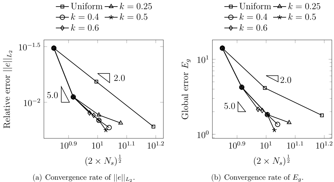
Figure 5.16: Convergence rate of \|e\|_{L_2} and E_g of the two-dimensional square domain under simple shear for the analyses with different k .
