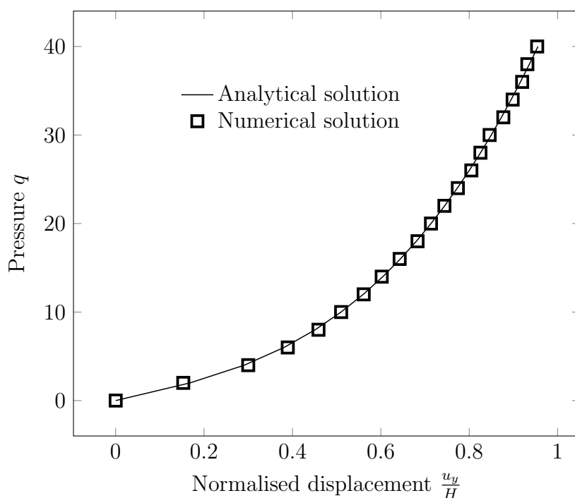
Figure 5.23: Pressure versus normalised displacement of the plate with uniformly distributed load, q , and simple supported ends.
