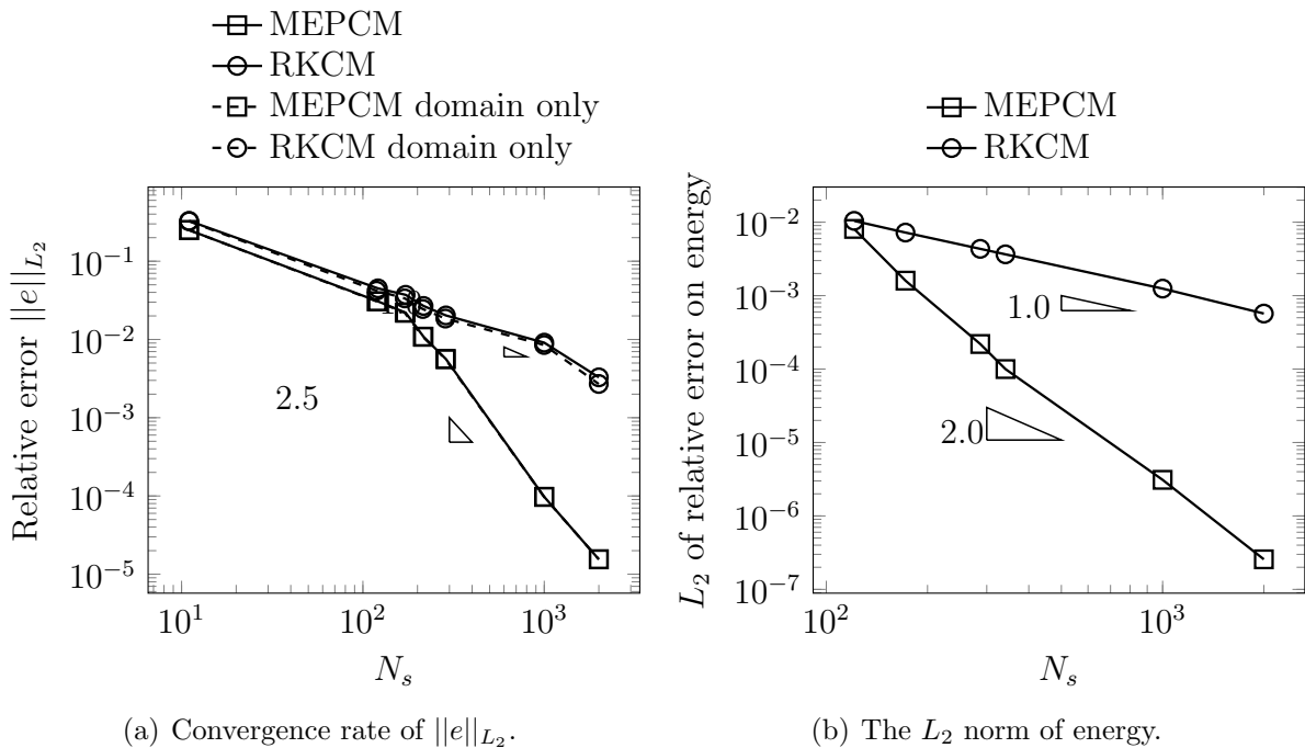
Figure 3.12: Convergence rate of \|e\|_{L_2} and energy norm of the one-dimensional bar problem using the MEPCM and the RKCM .
