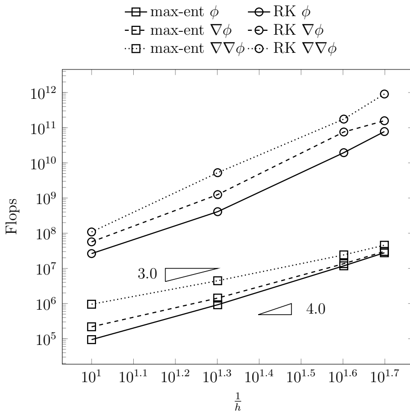
Figure 3.19: Flops of max-ent and RK basis functions and derivatives against 1/h in two dimensions.
