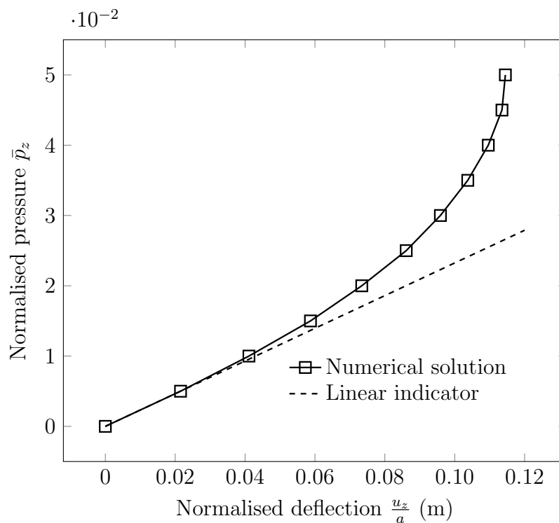
Figure 6.8: The normalised pressure \bar{p}_z at the centre point of the membrane surface against normalised deflection \frac{u_z}{a} of the initially flat linear elastic membrane problem subjected to a uniform pressure.
