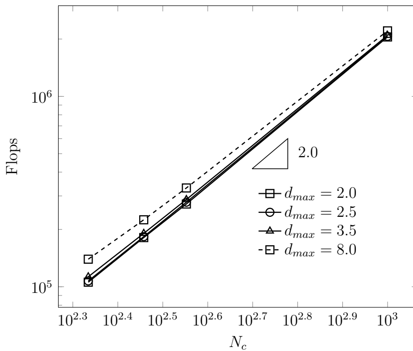
Figure 3.15: Flops of max-ent basis functions with different d_{max} of the one-dimensional bar problem.
