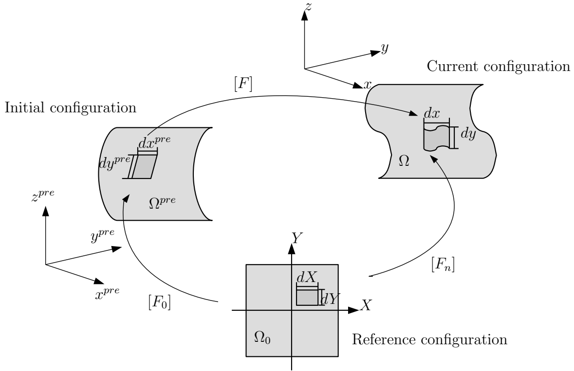
Figure 6.3: The reference, initial and current configurations of membranes.
