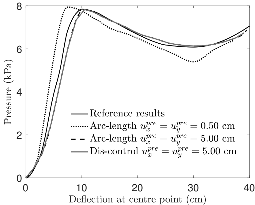
Figure 6.16: Pressure versus deflection at central point of the square hyperelastic membrane problem subjected to a uniform pressure.
