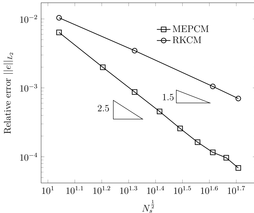
Figure 3.17: Convergence rate of \|e\|_{L_2} of the two-dimensional Poisson problem using the MEPCM and the RKCM.
