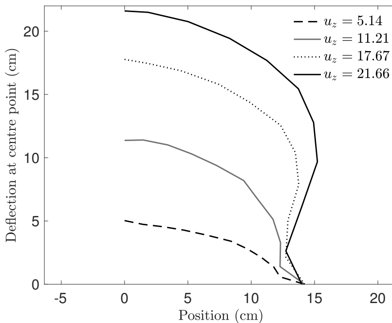
Figure 6.13: The deformed configurations with the out-of-plane displacement, u_z (cm) at different load steps of the half diagonal of the square hyperelastic membrane problem subjected to a uniform pressure.
