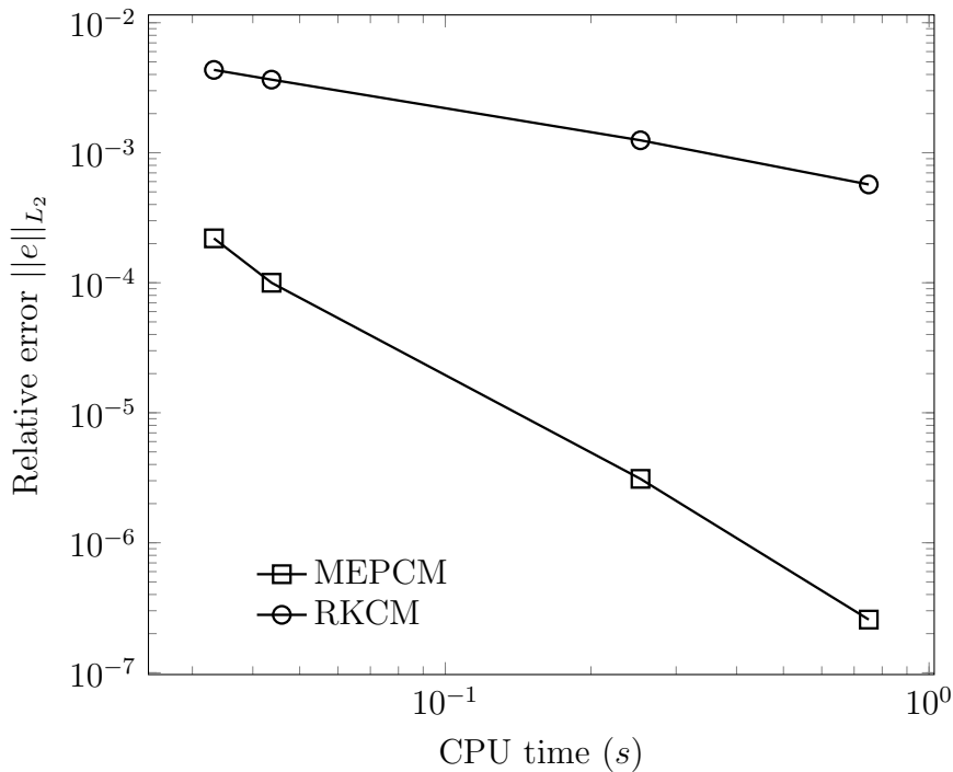
Figure 3.13: Convergence rate of \|e\|_{L_2} against CPU time of the one-dimensional bar problem using the MEPCM and the RKCM.
