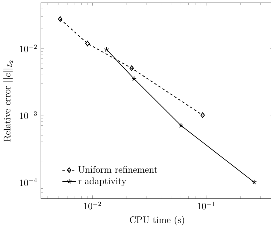
Figure 4.6: Convergence rate of \|e\|_{L_2} against CPU time of the one-dimensional bar problem using uniform refinement and r -adaptivity with N_s^* = 2 .
