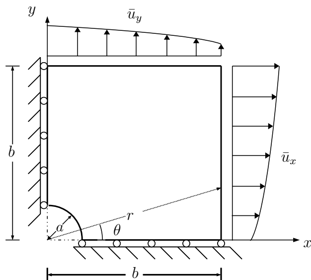
Figure 3.22: A portion of the infinite plate with a circular hole.
