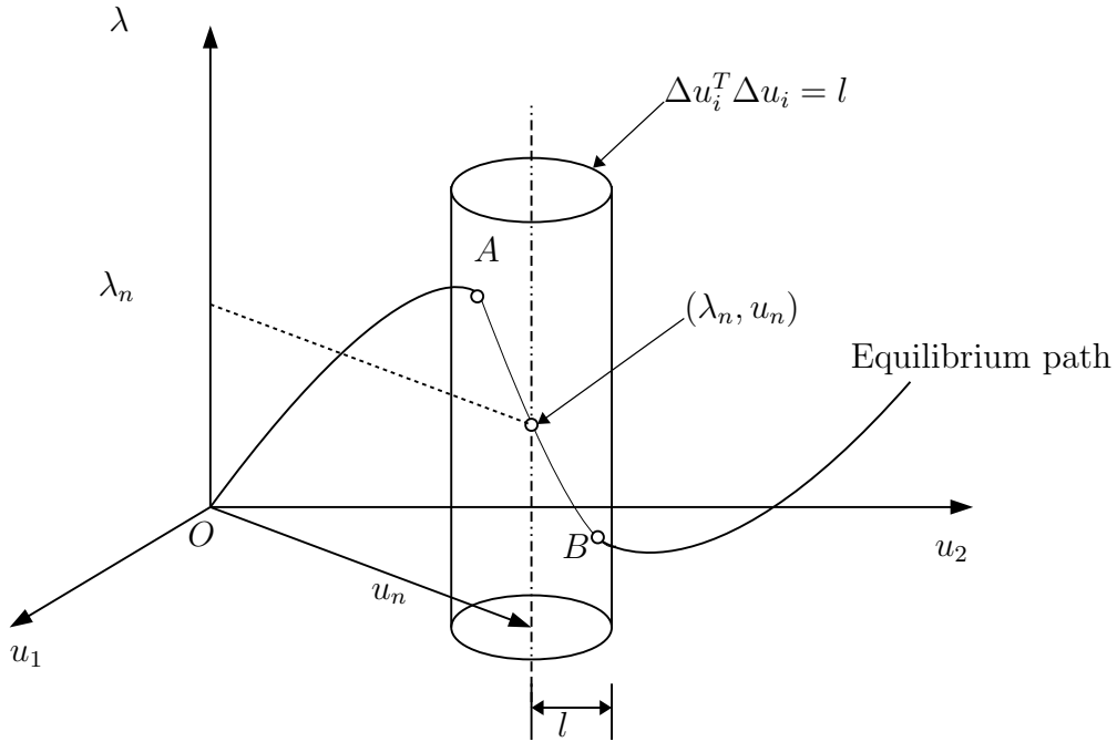
Figure D.1: The cylindrical arc-length method.
