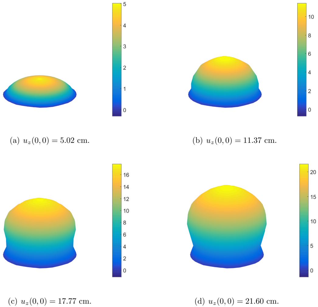
Figure 6.15: The deformed configurations with the out-of-plane displacement, u_z (cm) at different load steps of the circular hyperelastic membrane subjected to a uniform pressure.
