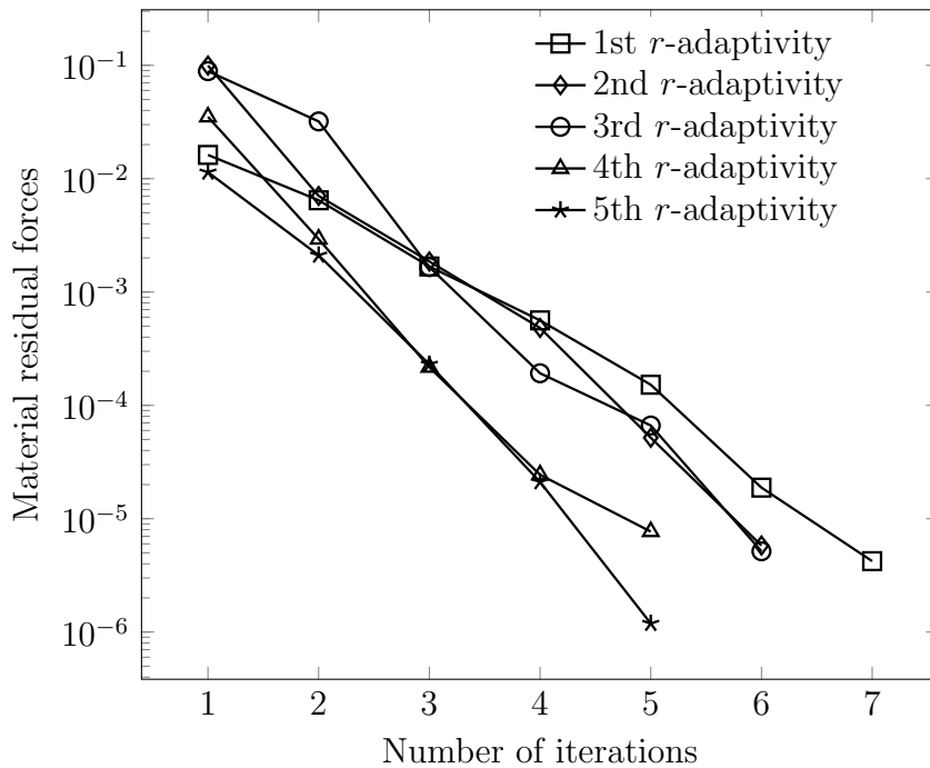
Figure 4.17: The material force residuals in the iteration process of the plate with a circular hole problem with k = 0.2 .
