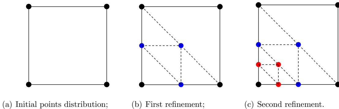
Figure 4.2: Step by step points refinement in h -adaptivity.
