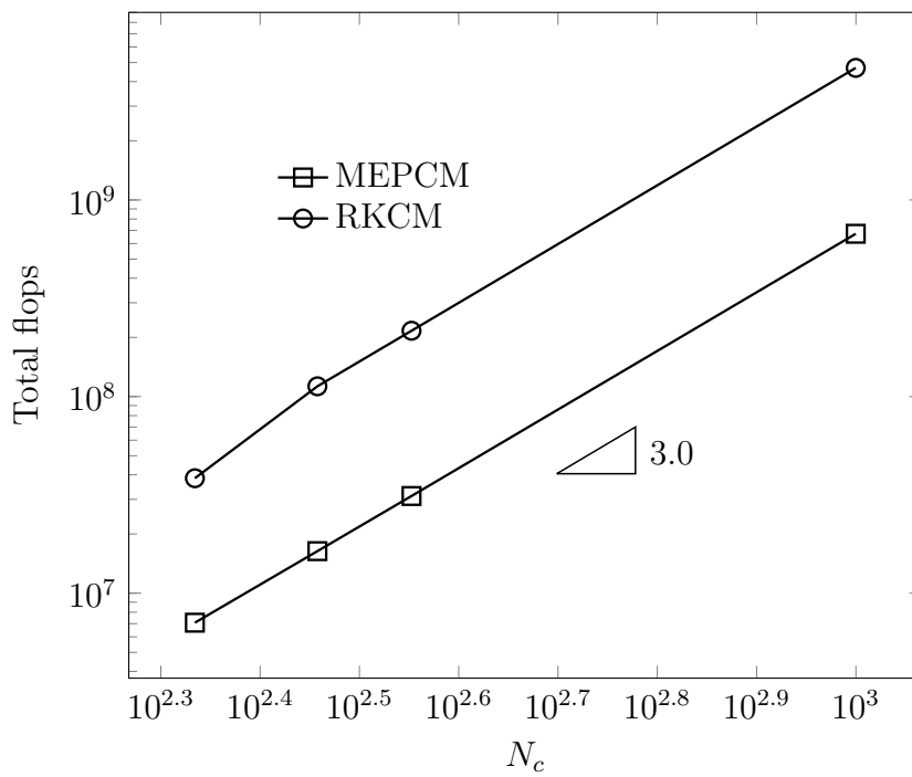
Figure 3.14: Total flops for analysis against N_c of the one-dimensional bar problem using the MEPCM and the RKCM.
