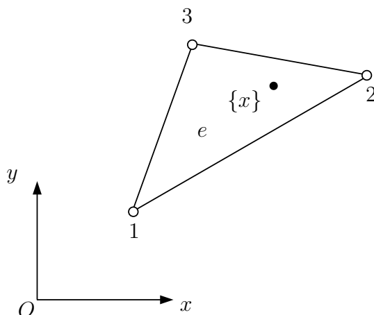
Figure 2.1: A two-dimensional element.
