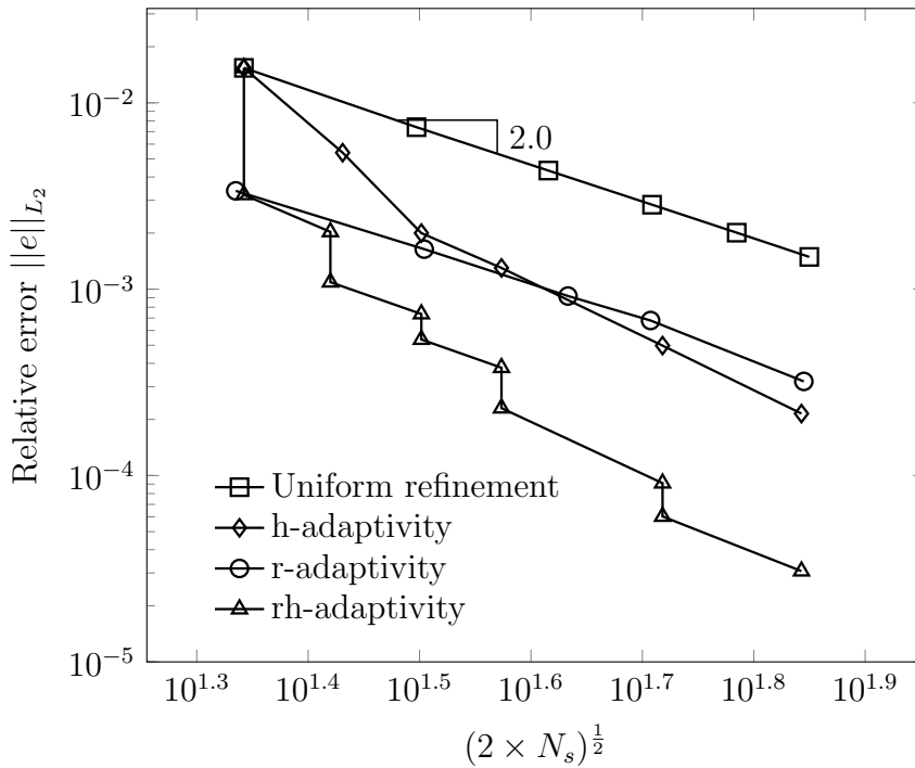
Figure 4.15: Convergence rate of \|e\|_{L_2} of the plate with a circular hole problem with k = 0.2 .
