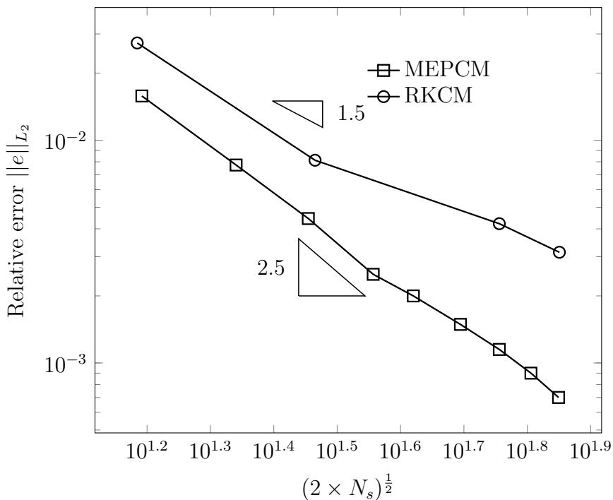
Figure 3.25: Convergence rate of \|e\|_{L_2} of an infinite plate with a circular hole problem using the MEPCM and the RKCM.
