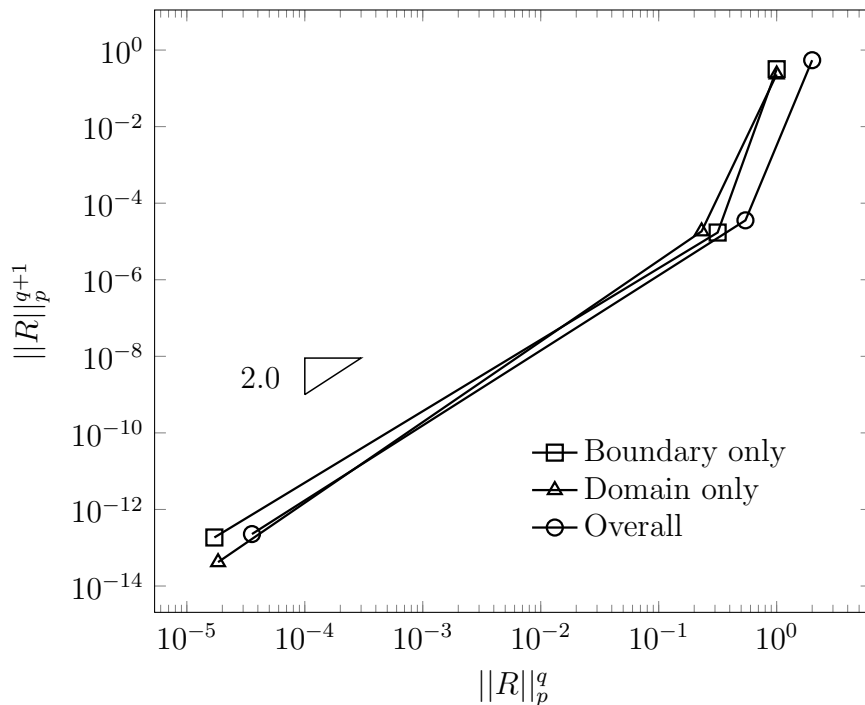
Figure 5.15: Convergence rate of residual norms in the second load step of the Newton-Raphson method of the two-dimensional square domain under simple shear.
