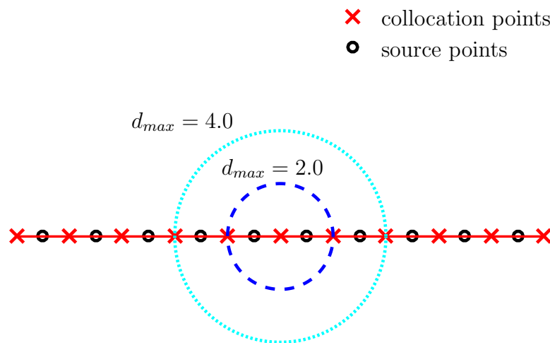
Figure 3.8: A portion of the one-dimensional bar with points distribution and different sizes of support domain.
