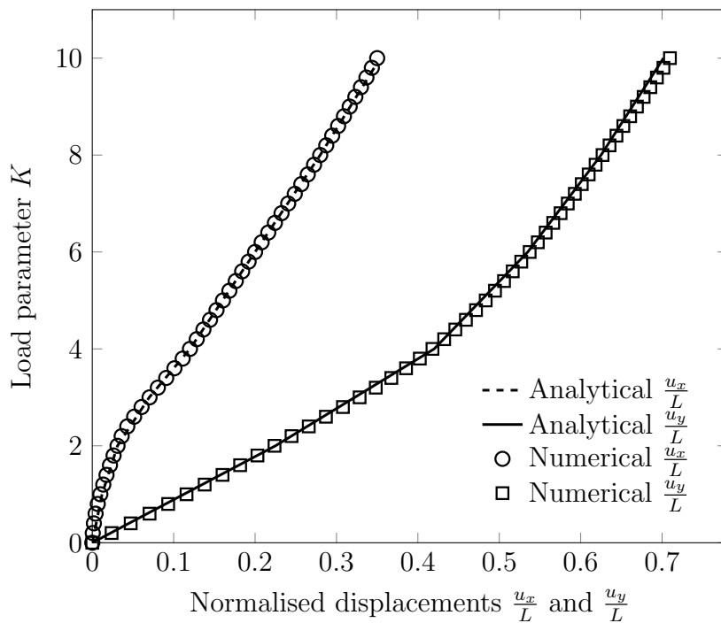
Figure 5.26: The load parameter K against normalised displacements, \frac{u_x}{L} and \frac{u_y}{L} , at the mid-depth point at the end of beam of the elastic cantilever beam problem with uniformly distributed load.
