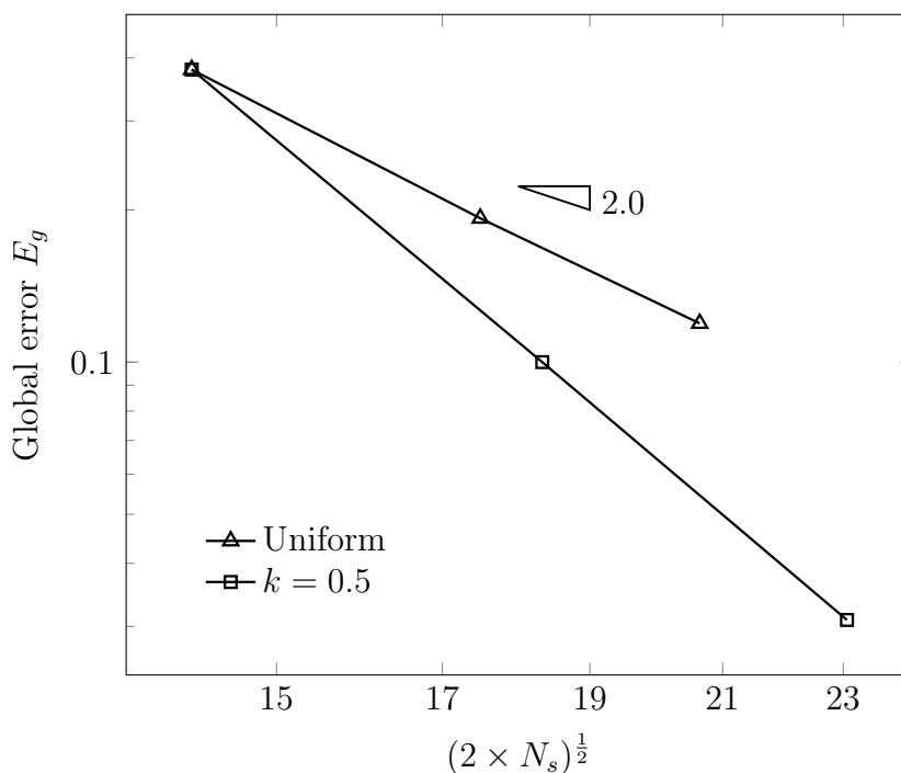
Figure 5.28: Convergence rate of E_g in h -adaptivity of the elastic cantilever beam problem with uniformly distributed load with k = 0.5 .
