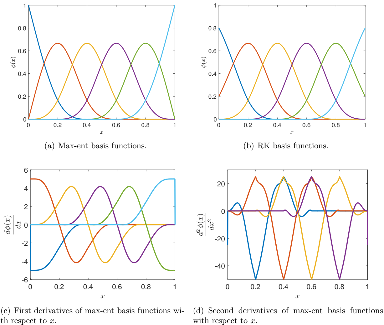
Figure 3.5: Max-ent and RK basis functions and first and second max-ent basis function derivatives over a one-dimensional domain.
