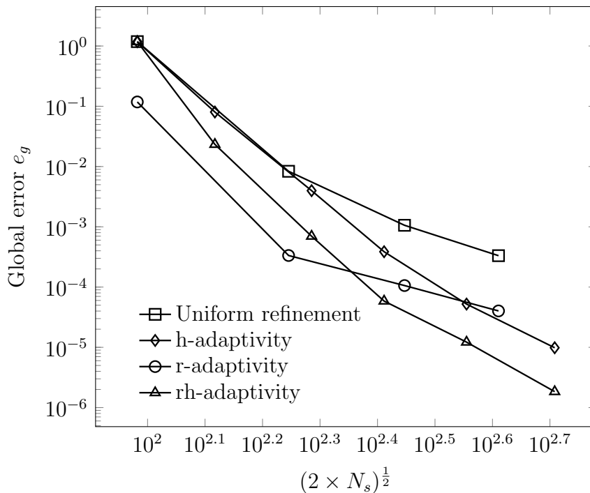
Figure 4.20: Convergence rate of e_g using different adaptivity of the L-shaped plate with k = 0.3 .
