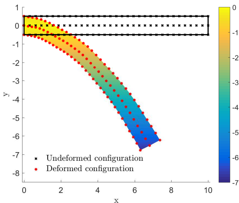
Figure 5.25: The reference and current configurations with displacement u_y of the elastic cantilever beam problem with uniformly distributed load.
