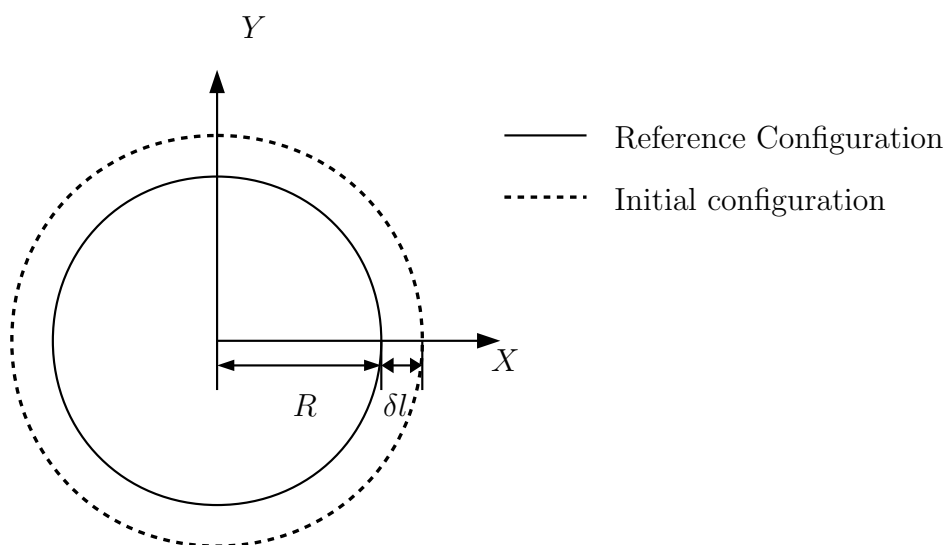
Figure 6.14: The reference and initial configurations of the circular hyperelastic membrane subjected to a uniform pressure.
