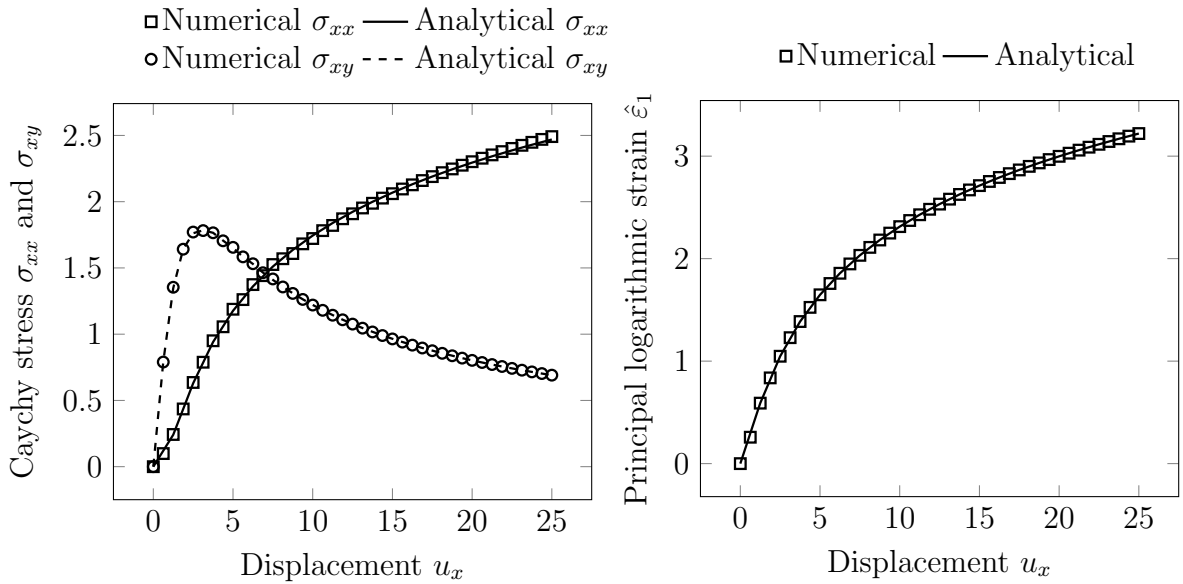
(a) Cauchy stress components \sigma_{xx} and \sigma_{xy} against displacement in x direction u_x .
