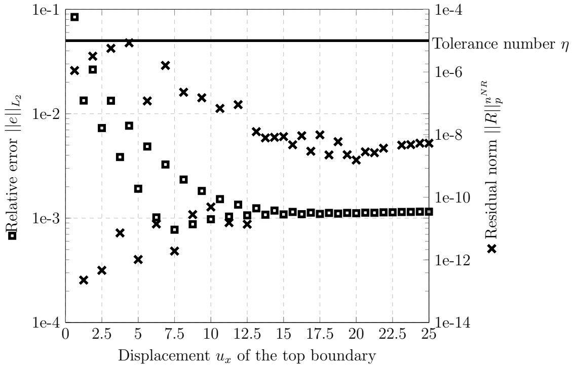
Figure 5.14: L_2 norm of relative error \|e\|_{L_2} and the residual norm \|R\|_p^{n_{NR}} in each load step of the Newton-Raphson method against displacement of the top boundary of the two-dimensional square domain under simple shear.
