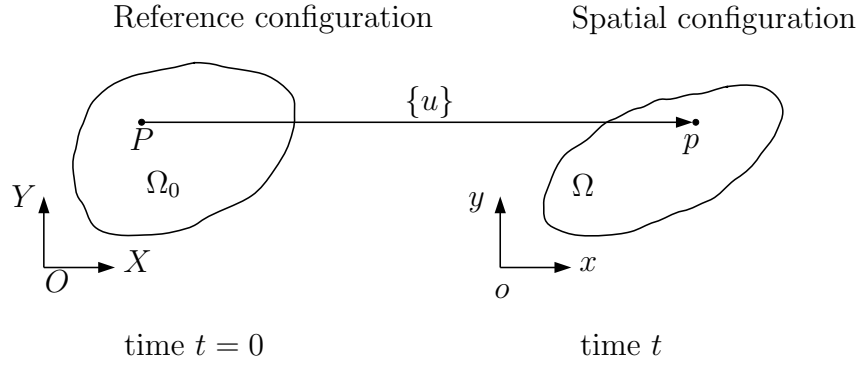
Figure 5.1: Configuration and motion of a continuum body.
