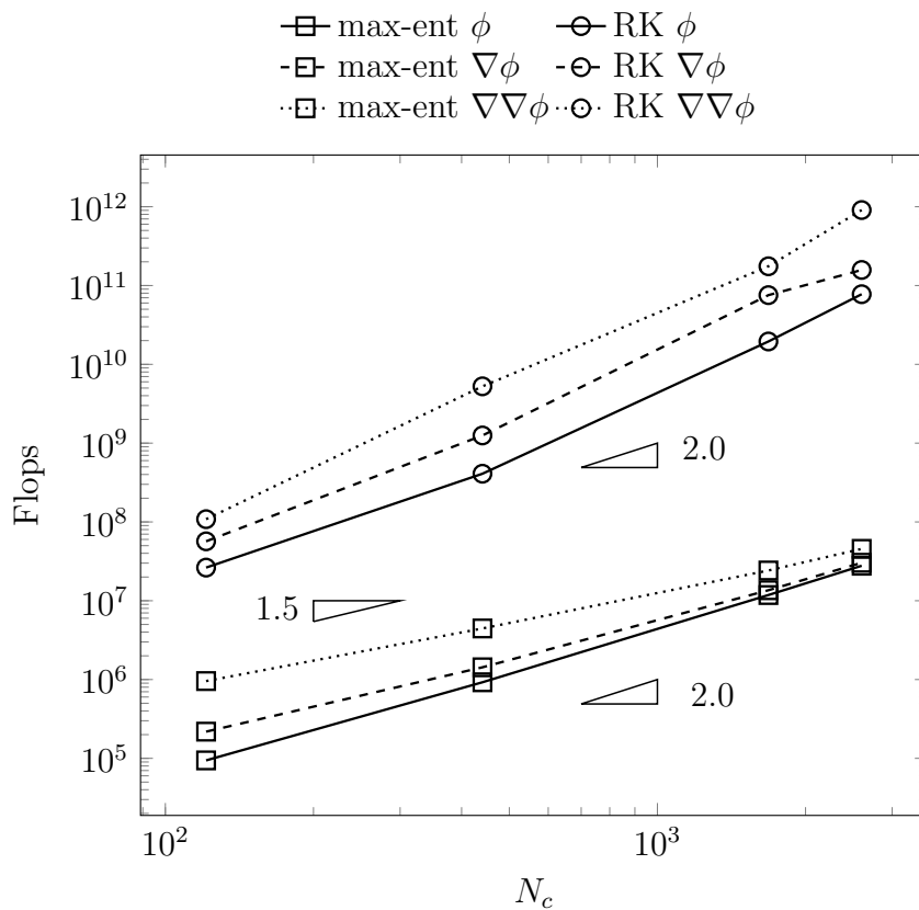
Figure 3.18: Flops of max-ent and RK basis functions and derivatives in two dimensions.
