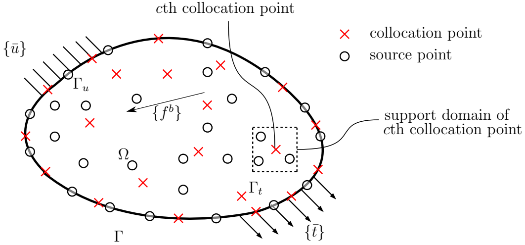
Figure 3.2: A two-dimensional problem domain subjected to the body force and boundary conditions with points discretisation.
