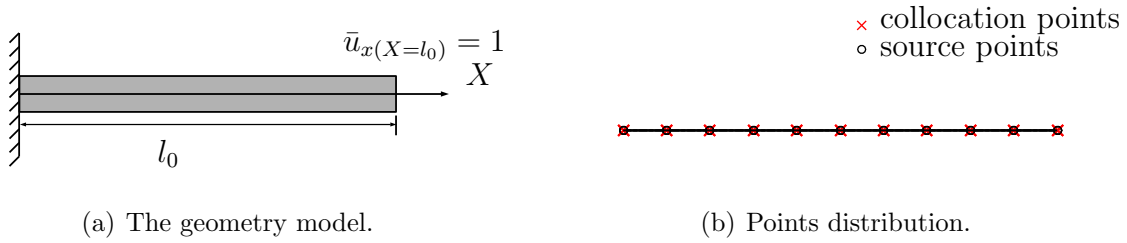
Figure 5.3: The geometry model and points distributions of the one-dimensional bar problem.
