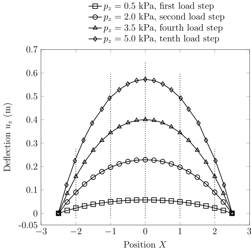
Figure 6.7: The deflections u_z (m) at Y = 0 over different load steps of the initially flat linear elastic membrane problem subjected to a uniform pressure.
