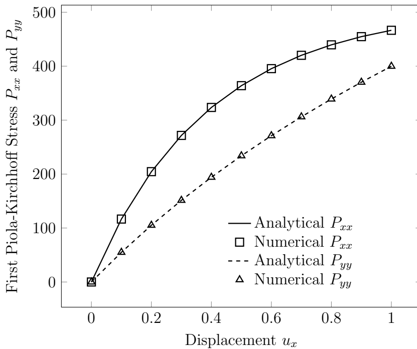
Figure 5.9: Tension of a two-dimensional square domain: first Piola-Kirchhoff stress components P_{xx} and P_{yy} against displacement in x direction u_x .
