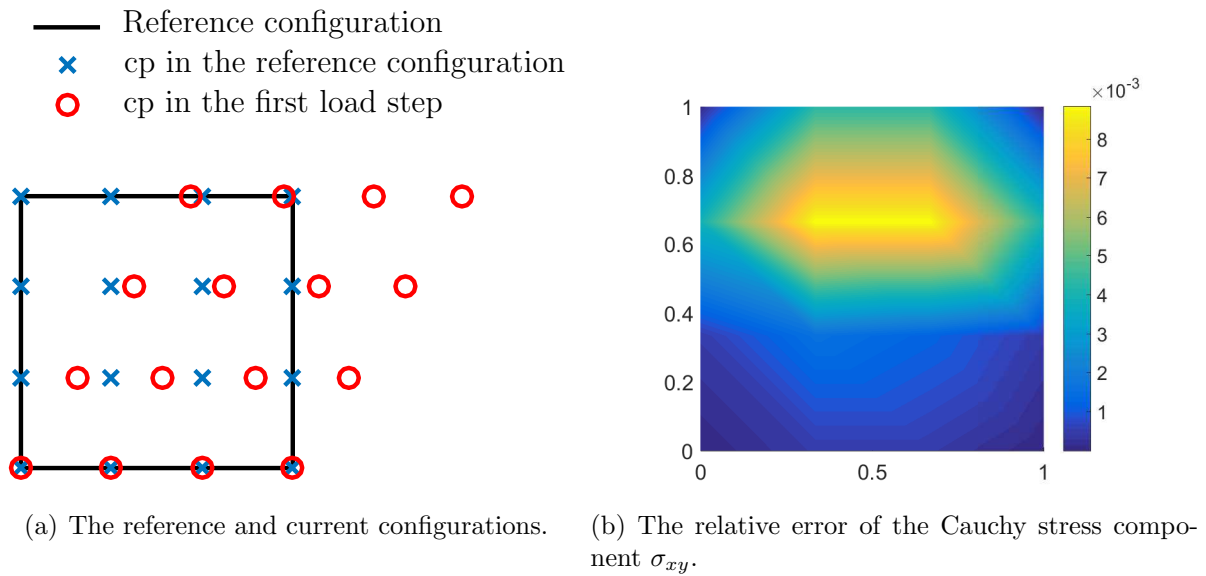
Figure 5.13: Configurations and relative error of Cauchy stress error component \sigma_{xy} of the two-dimensional square domain under simple shear.
