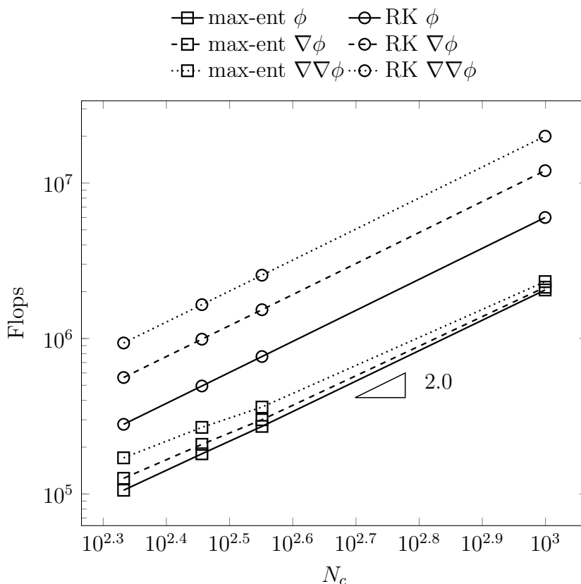
Figure 3.16: Flops of max-ent and RK basis functions and derivatives in one dimension.
