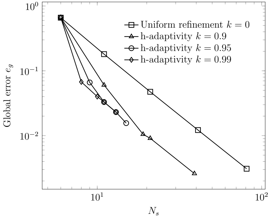
Figure 4.9: Convergence rate of e_g of the one-dimensional bar problem using different k with N_s^* = 2 .
