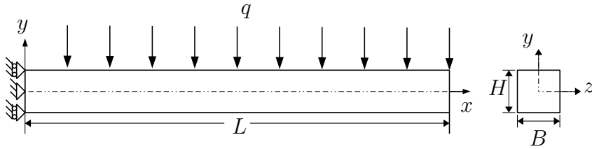
Figure 5.24: Geometry of the elastic cantilever beam problem with uniformly distributed load.
