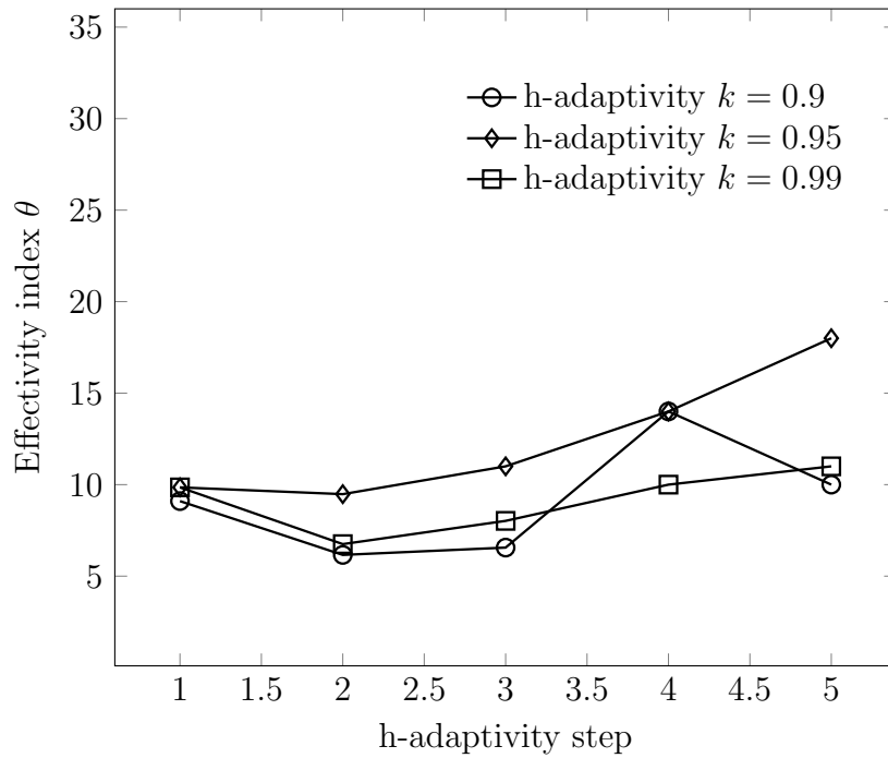
Figure 4.11: The effectivity index using h -adaptivity of a one-dimensional bar problem using different k with N_s^* = 2 .
