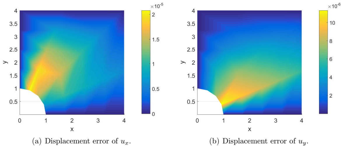
Figure 3.24: Absolute errors of displacement in x and y directions of the infinite plate with a circular hole problem using the MEPCM.
