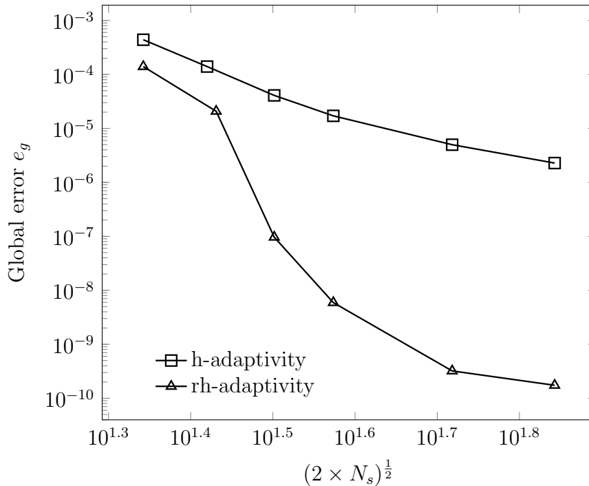
Figure 4.16: Convergence rate of e_g using h and hr -adaptivity of the plate with a circular hole problem with k = 0.2 .
