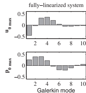
Figure 13. Amplitudes of the Galerkin modes that cause the maximum transient growth in Figure 12.
