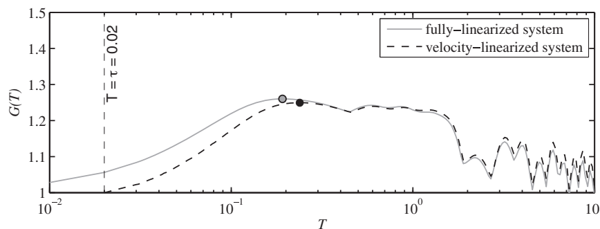
Figure 12. Maximum transient growth, G(T) , as a function of optimization time, T , for the 10 mode Rijke tube with x_f = 0.3 , c_1 = 0.05 , c_2 = 0.01 , \tau = 0.02 , and \beta = 0.75 for the fully-linearized system (solid line). The maximum value is G_{max} = 1.26 at T = 0.2 .
