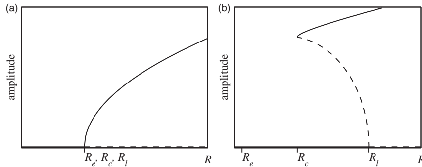
Figure 1. The steady state oscillation amplitude, a_{SS} , as a function of a control parameter, R , for (a) a supercritical bifurcation and (b) a subcritical bifurcation. R_l is the point at which the fixed point (i.e., the zero amplitude solution) becomes unstable. R_c is the point below which no oscillations can be sustained and R_e is the point below which all perturbations decrease monotonically to zero.
