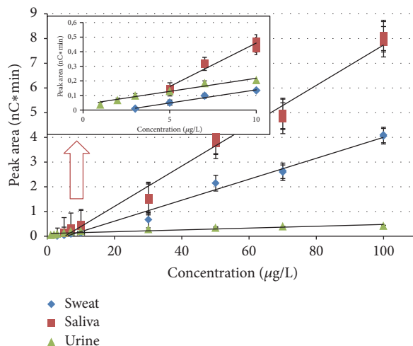
FIGURE 5: Ion chromatography calibration curves for cyanide ion analyzed in biological samples.
