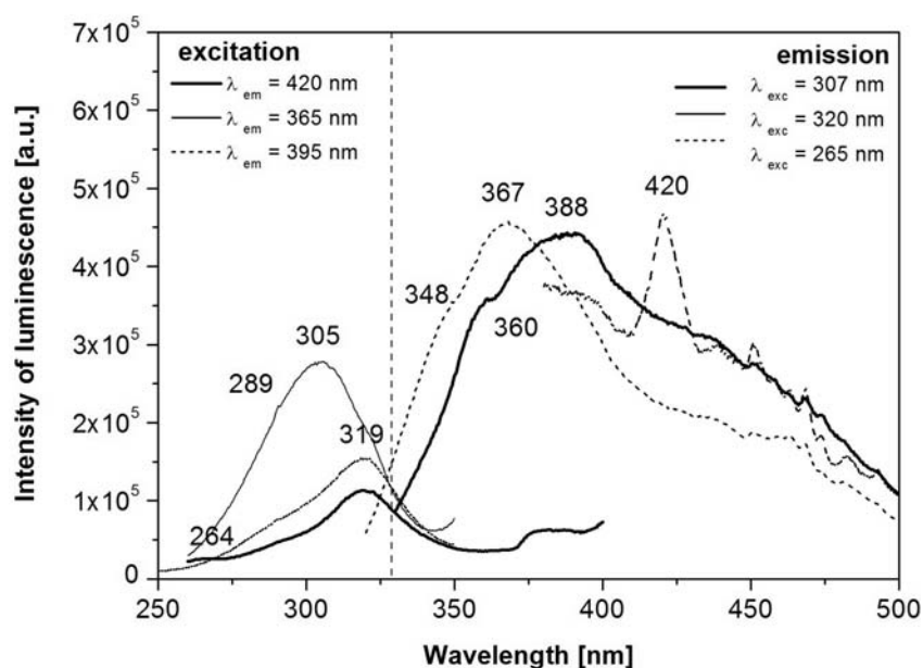
Fig. 5. The excitation and emission spectra of Ce^{3+} in the Spanish apatite (Table 1)
