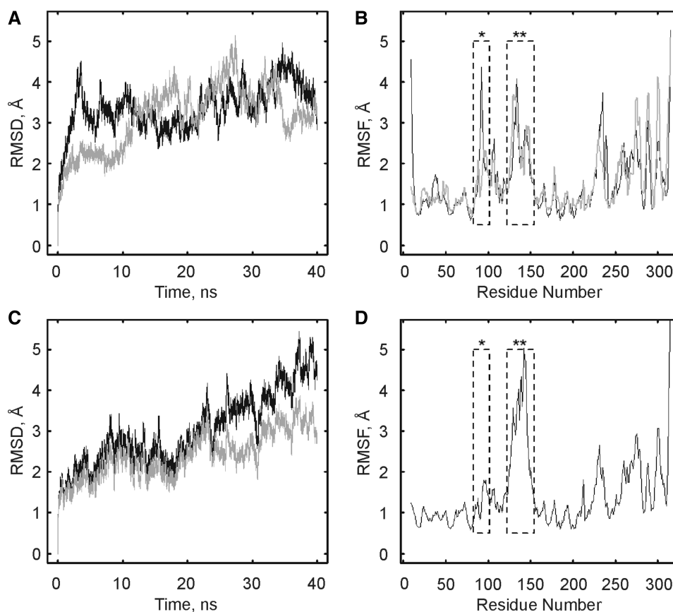
Figure 6. Global fluctuations of TruB during MD simulations. TruB wild type (in the absence of RNA, panels (A and B)) was simulated at 310 K in the apo and bound conformation based on available crystal structures with and without RNA, respectively (for details see ‘Materials and Methods’ section). TruB D90N (C and D) was simulated in the bound conformation only. (A) RMSD of the backbone atoms of all residues for TruB wild type simulations (apo conformation, gray; bound conformation, black). (B) RMSF values for simulation of TruB wild type from 5–40 ns, with insert 1 (asterisk) and thumb-loop (double asterisk) residues indicated by dashed boxes (apo conformation, gray; bound conformation, black). (C) TruB D90N simulation. RMSD of the backbone atoms of all residues (black) and for backbone atoms of all residues excluding thumb-loop residues 124–152 (gray). (D) RMSF values for TruB D90N residues from 5 to 40 ns of simulation; insert 1 (asterisk) and thumb loop (double asterisk).
