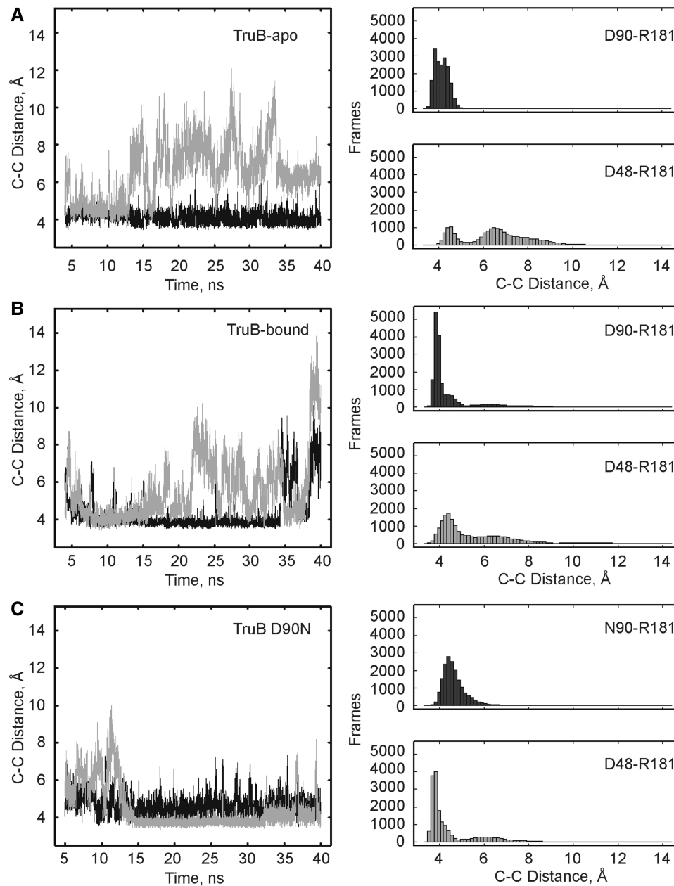
Figure 7. Active site residue interactions during MD simulations. Every 2 ps of simulation time, distances were measured between the guanidinium carbon of R181 and the carboxylate carbon of D48 and D90. The D48–R181 interaction is depicted in gray while the D90–R181 interaction is shown in black. Both time-resolved changes (left) as well as histograms of C-C distances (right) are reported. (A) TruB wild type in the apo conformation. (B) TruB wild type in the bound conformation. (C) TruB D90N in the bound conformation.
