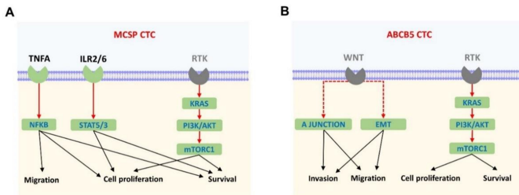
Figure 3. MCSP- and ABCB5-enriched CTCs exhibit distinct transcriptional programming, with ABCB5 CTCs displaying an invasive phenotype. Schematic representation of cellular hallmarks enriched by the genes found to be differentially up-regulated in (A) MCSP- and (B) ABCB5-enriched CTCs. Enriched cellular hallmarks in CTCs are shown in green boxes, while genes shown in grey are those that were not found enriched in this study but are known to be important for melanomagenesis. Canonical pathway signalling is indicated by continuous arrows and dotted arrows indicates a previously reported interaction.
